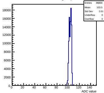
Pedestals mcm150-7A16-refv1-g0-s0-p1 ch 76 test1
