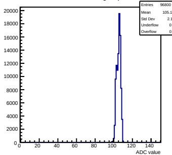
Pedestals mcm150-7A16-refv1-g0-s0-p1 ch 78 test1
