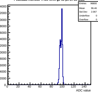
Pedestals mcm150-7A16-refv1-g0-s0-p1 ch 65 test1
