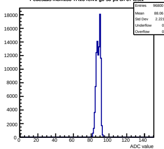
Pedestals mcm150-7A16-refv1-g0-s0-p1 ch 67 test1
