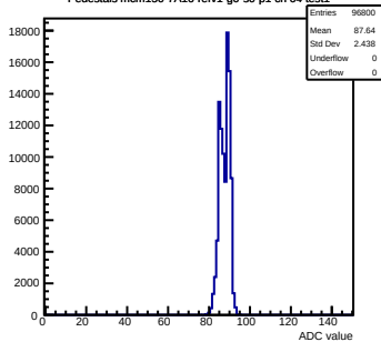
Pedestals mcm150-7A16-refv1-g0-s0-p1 ch 64 test1
