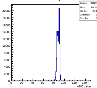
Pedestals mcm150-7A16-refv1-g0-s0-p1 ch 75 test1
