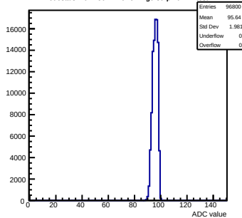
Pedestals mcm150-7A16-refv1-g0-s0-p1 ch 71 test1
