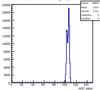
Pedestals mcm150-7A16-refv1-g0-s0-p1 ch 72 test1
