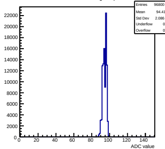
Pedestals mcm150-7A16-refv1-g0-s0-p1 ch 79 test1
