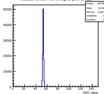
Pedestals mcm150-7A16-refv3-g0-s0-p1 ch 95 test1
