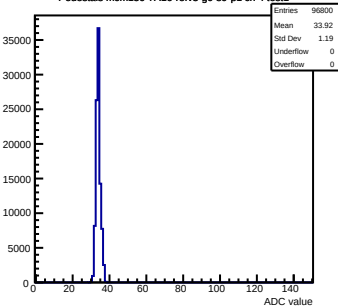
Pedestals mcm150-7A16-refV3-g0-s0-p1 ch 0 test1
