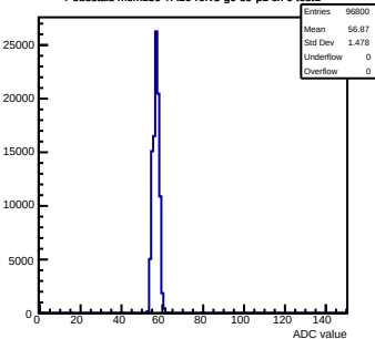
Pedestals mcm150-7A16-refV3-g0-s0-p1 ch 1 test1
