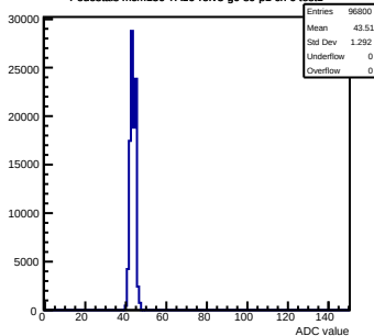
Pedestals mcm150-7A16-refV3-g0-s0-p1 ch 6 test1
