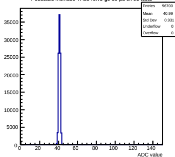
Pedestals mcm150-7A16-refv3-g0-s0-p1 ch 93 test1
