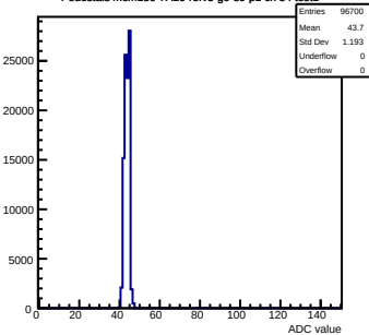
Pedestals mcm150-7A16-refv3-g0-s0-p1 ch 84 test1
