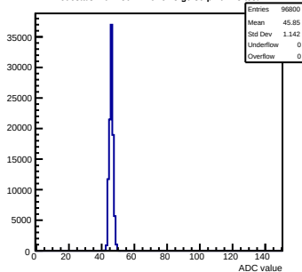
Pedestals mcm150-7A16-refV3-g0-s0-p1 ch 13 test1
