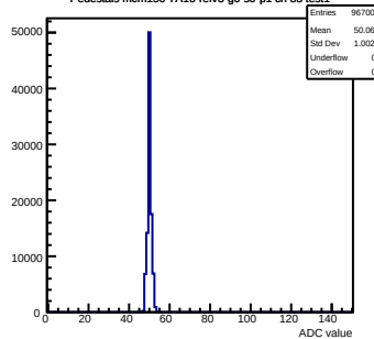
Pedestals mcm150-7A16-refv3-g0-s0-p1 ch 83 test1
