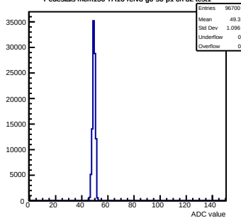
Pedestals mcm150-7A16-refv3-g0-s0-p1 ch 82 test1
