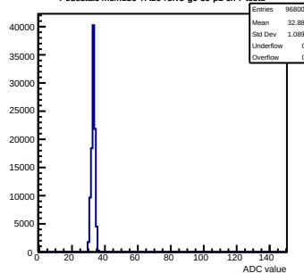
Pedestals mcm150-7A16-refV3-g0-s0-p1 ch 7 test1
