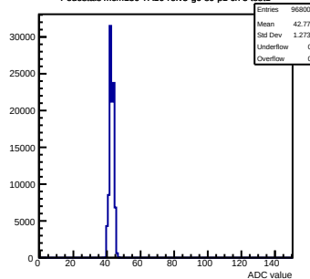
Pedestals mcm150-7A16-refV3-g0-s0-p1 ch 3 test1
