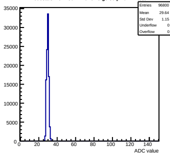
Pedestals mcm150-7A16-refV3-g0-s0-p1 ch 14 test1
