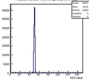
Pedestals mcm150-7A16-refv3-g0-s0-p1 ch 89 test1
