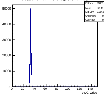
Pedestals mcm150-7A16-refV3-g0-s0-p1 ch 1 test1
