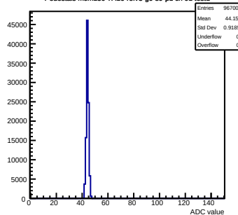
Pedestals mcm150-7A16-refv3-g0-s0-p1 ch 91 test1
