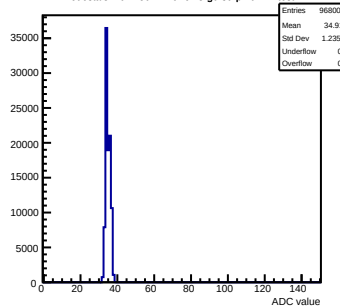
Pedestals mcm150-7A16-refV3-g0-s0-p1 ch 11 test1
