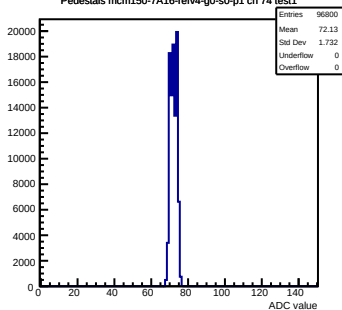
Pedestals mcm150-7A16-refv4-g0-s0-p1 ch 74 test1
