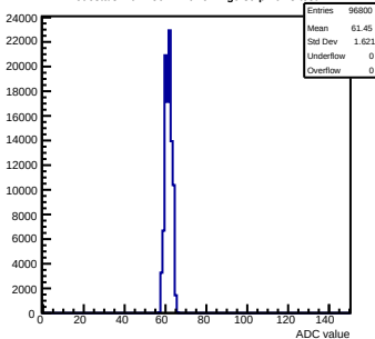
Pedestals mcm150-7A16-refv4-g0-s0-p1 ch 3 test1
