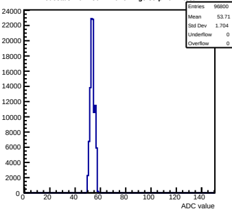
Pedestals mcm150-7A16-refv4-g0-s0-p1 ch 4 test1
