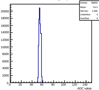
Pedestals mcm150-7A16-refv4-g0-s0-p1 ch 44 test1
