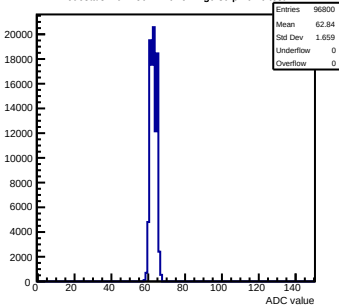
Pedestals mcm150-7A16-refv4-g0-s0-p1 ch 6 test1
