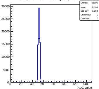
Pedestals mcm150-7A16-refv4-g0-s0-p1 ch 1 test1
