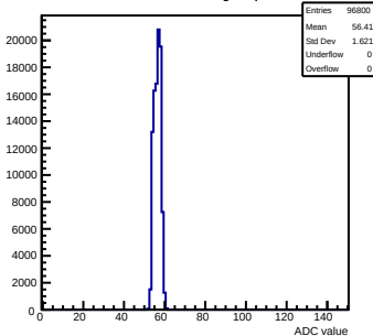
Pedestals mcm150-7A16-refv4-g0-s0-p1 ch 15 test1
