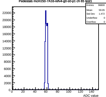
Pedestals mcm150-7A16-refv4-g0-s0-p1 ch 65 test1
