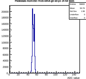
Pedestals mcm150-7A16-refv4-g0-s0-p1 ch 64 test1
