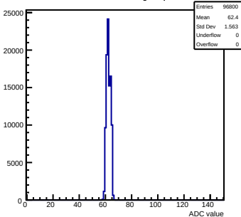
Pedestals mcm150-7A16-refv4-g0-s0-p1 ch 13 test1
