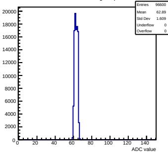
Pedestals mcm150-7A16-refv4-g0-s0-p1 ch 41 test1
