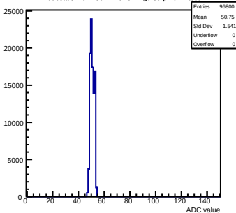
Pedestals mcm150-7A16-refv4-g0-s0-p1 ch 7 test1
