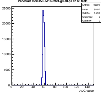
Pedestals mcm150-7A16-refv4-g0-s0-p1 ch 66 test1
