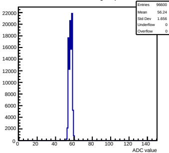
Pedestals mcm150-7A16-refv4-g0-s0-p1 ch 45 test1
