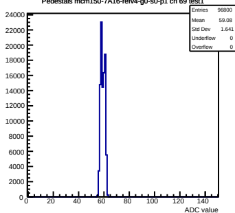
Pedestals mcm150-7A16-refv4-g0-s0-p1 ch 69 test1
