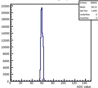
Pedestals mcm150-7A16-refv4-g0-s0-p1 ch 10 test1
