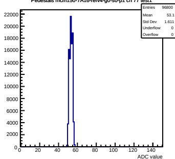
Pedestals mcm150-7A16-refv4-g0-s0-p1 ch 77 test1
