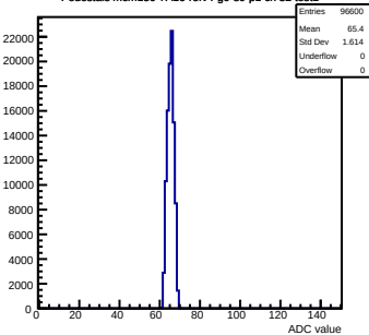
Pedestals mcm150-7A16-refv4-g0-s0-p1 ch 32 test1
