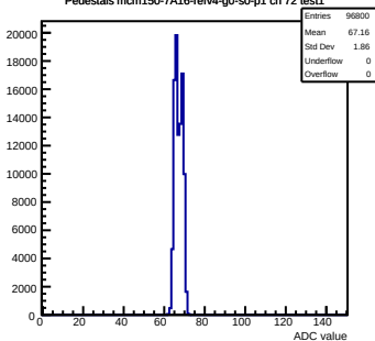
Pedestals mcm150-7A16-refv4-g0-s0-p1 ch 72 test1
