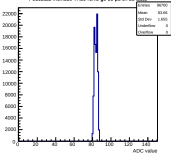
Pedestals mcm150-7A16-refV5-g0-s0-p1 ch 21 test1
