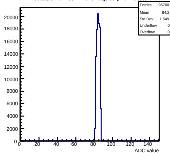
Pedestals mcm150-7A16-refV5-g0-s0-p1 ch 23 test1
