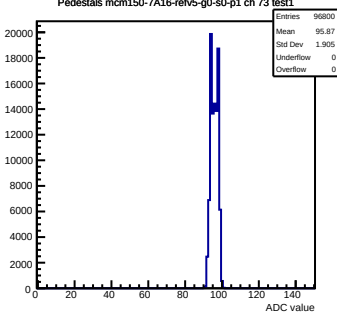
Pedestals mcm150-7A16-refV5-g0-s0-p1 ch 73 test1
