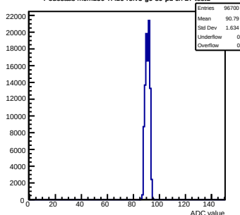
Pedestals mcm150-7A16-refV5-g0-s0-p1 ch 27 test1
