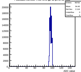
Pedestals mcm150-7A16-refV5-g0-s0-p1 ch 16 test1
