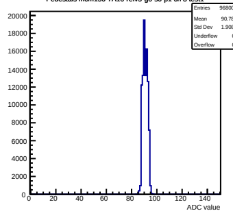
Pedestals mcm150-7A16-refV5-g0-s0-p1 ch 3 test1
