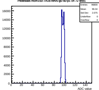
Pedestals mcm150-7A16-refV5-g0-s0-p1 ch 72 test1
