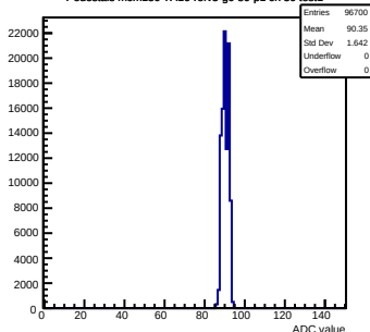
Pedestals mcm150-7A16-refV5-g0-s0-p1 ch 30 test1
