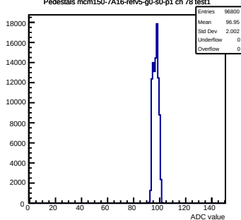
Pedestals mcm150-7A16-refV5-g0-s0-p1 ch 78 test1
