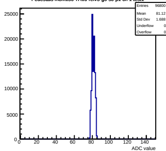
Pedestals mcm150-7A16-refV5-g0-s0-p1 ch 1 test1
