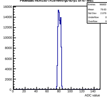
Pedestals mcm150-7A16-refV5-g0-s0-p1 ch 67 test1
