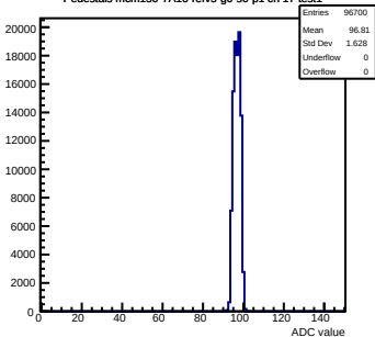
Pedestals mcm150-7A16-refV5-g0-s0-p1 ch 17 test1
