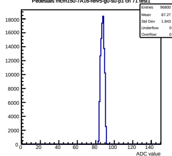
Pedestals mcm150-7A16-refV5-g0-s0-p1 ch 71 test1
