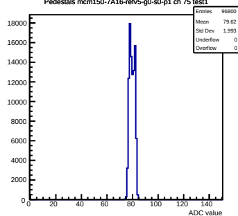
Pedestals mcm150-7A16-refV5-g0-s0-p1 ch 75 test1
