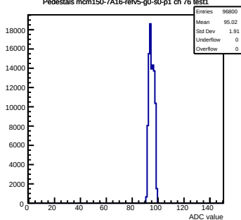
Pedestals mcm150-7A16-refV5-g0-s0-p1 ch 76 test1
