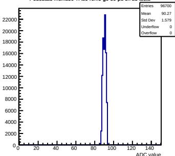
Pedestals mcm150-7A16-refV5-g0-s0-p1 ch 25 test1
