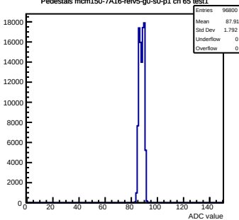
Pedestals mcm150-7A16-refV5-g0-s0-p1 ch 65 test1
