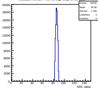
Pedestals mcm150-7A16-refV5-g0-s0-p1 ch 20 test1
