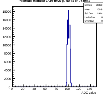
Pedestals mcm150-7A16-refV5-g0-s0-p1 ch 74 test1
