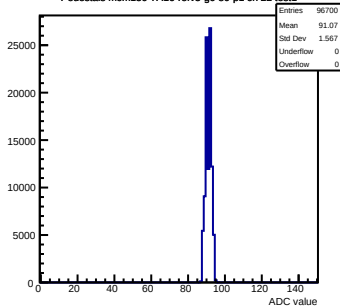
Pedestals mcm150-7A16-refV5-g0-s0-p1 ch 22 test1
