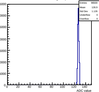
Pedestals mcm150-7A16-refV6-g0-s0-p1 ch 125 test1
