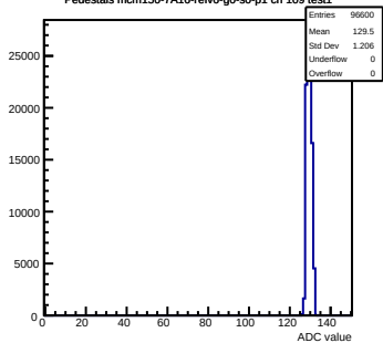
Pedestals mcm150-7A16-refv6-g0-s0-p1 ch 109 test1
