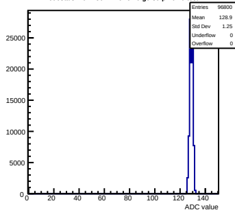
Pedestals mcm150-7A16-relv6-g0-s0-p1 ch 9 test1
