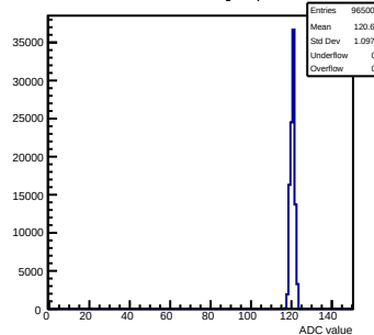
Pedestals mcm150-7A16-refV6-g0-s0-p1 ch 123 test1
