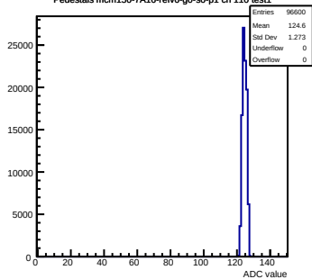
Pedestals mcm150-7A16-refv6-g0-s0-p1 ch 110 test1
