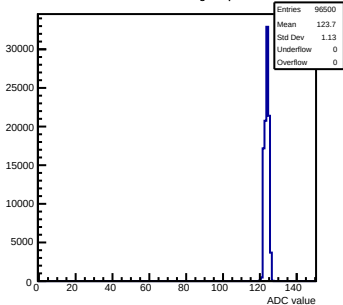
Pedestals mcm150-7A16-refV6-g0-s0-p1 ch 124 test1
