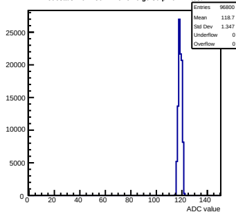
Pedestals mcm150-7A16-relv6-g0-s0-p1 ch 14 test1
