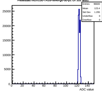
Pedestals mcm150-7A16-refv6-g0-s0-p1 ch 102 test1
