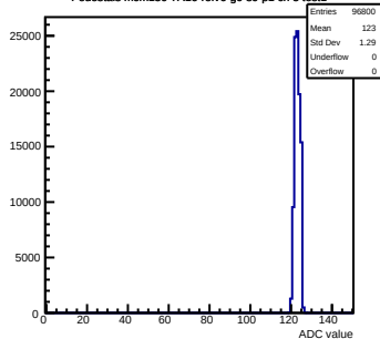
Pedestals mcm150-7A16-relv6-g0-s0-p1 ch 5 test1
