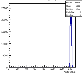
Pedestals mcm150-7A16-relv6-g0-s0-p1 ch 12 test1
