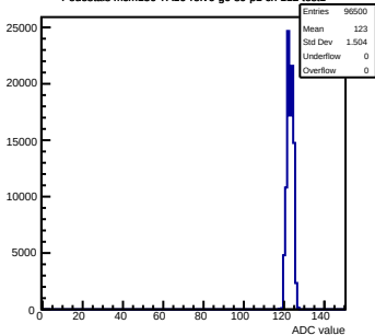
Pedestals mcm150-7A16-refV6-g0-s0-p1 ch 112 test1
