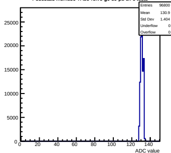
Pedestals mcm150-7A16-relv6-g0-s0-p1 ch 6 test1
