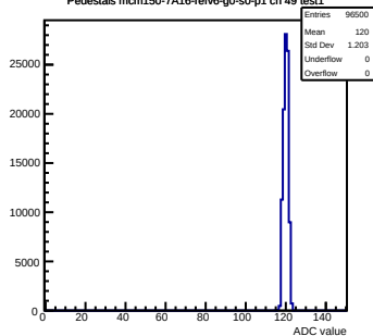
Pedestals mcm150-7A16-refv6-g0-s0-p1 ch 49 test1
