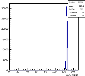
Pedestals mcm150-7A16-refV6-g0-s0-p1 ch 120 test1
