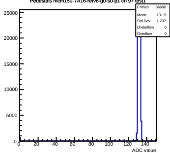
Pedestals mcm150-7A16-refv6-g0-s0-p1 ch 97 test1
