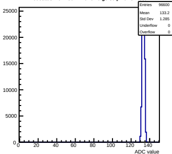
Pedestals mcm150-7A16-refv6-g0-s0-p1 ch 32 test1
