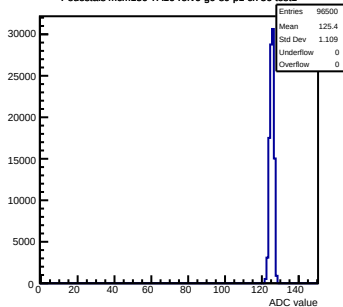
Pedestals mcm150-7A16-refv6-g0-s0-p1 ch 56 test1
