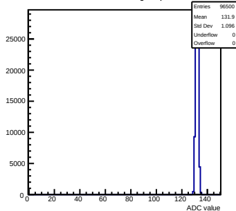
Pedestals mcm150-7A16-refV6-g0-s0-p1 ch 122 test1
