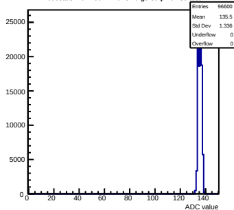
Pedestals mcm150-7A16-refv6-g0-s0-p1 ch 39 test1
