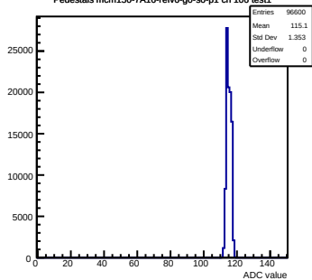
Pedestals mcm150-7A16-refv6-g0-s0-p1 ch 106 test1
