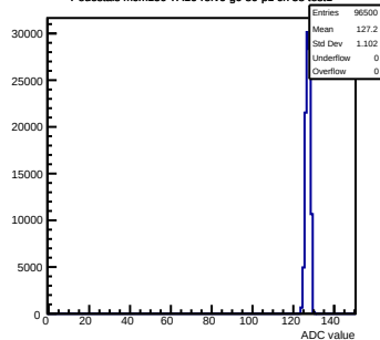
Pedestals mcm150-7A16-refv6-g0-s0-p1 ch 58 test1
