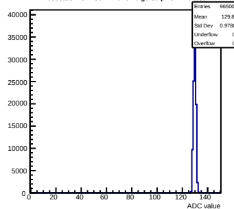
Pedestals mcm150-7A16-refV6-g0-s0-p1 ch 119 test1
