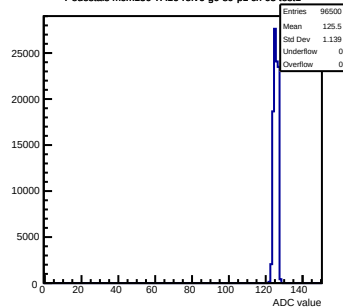
Pedestals mcm150-7A16-refv6-g0-s0-p1 ch 63 test1
