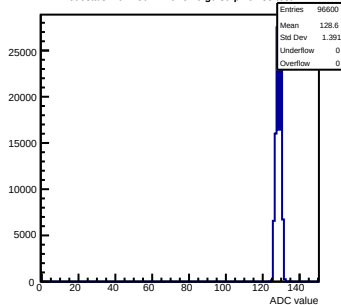
Pedestals mcm150-7A16-refv6-g0-s0-p1 ch 35 test1
