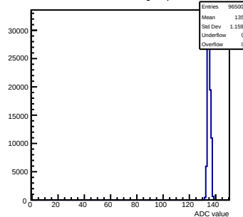
Pedestals mcm150-7A16-refV6-g0-s0-p1 ch 127 test1
