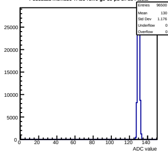
Pedestals mcm150-7A16-refV6-g0-s0-p1 ch 114 test1
