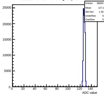
Pedestals mcm150-7A16-relv6-g0-s0-p1 ch 10 test1
