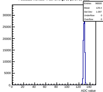
Pedestals mcm150-7A16-refv6-g0-s0-p1 ch 61 test1
