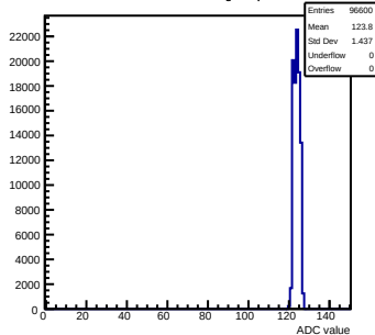
Pedestals mcm150-7A16-refv6-g0-s0-p1 ch 42 test1
