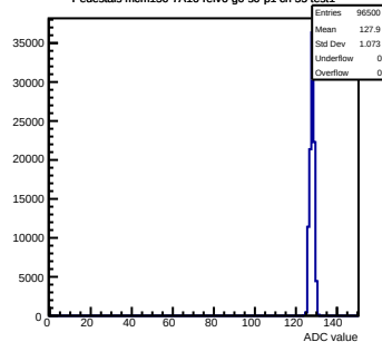
Pedestals mcm150-7A16-refv6-g0-s0-p1 ch 55 test1
