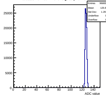
Pedestals mcm150-7A16-relv6-g0-s0-p1 ch 15 test1
