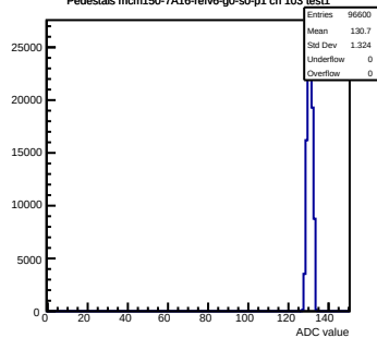
Pedestals mcm150-7A16-refv6-g0-s0-p1 ch 103 test1
