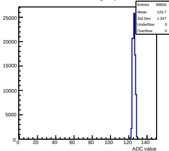
Pedestals mcm150-7A16-refv6-g0-s0-p1 ch 45 test1
