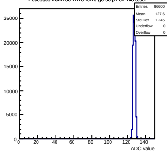
Pedestals mcm150-7A16-refv6-g0-s0-p1 ch 108 test1
