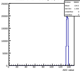
Pedestals mcm150-7A16-refv6-g0-s0-p1 ch 36 test1
