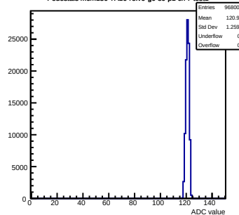
Pedestals mcm150-7A16-relv6-g0-s0-p1 ch 7 test1
