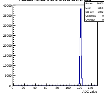
Pedestals mcm150-7A16-refv6-g0-s0-p1 ch 54 test1
