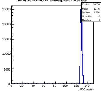
Pedestals mcm150-7A16-refv6-g0-s0-p1 ch 96 test1
