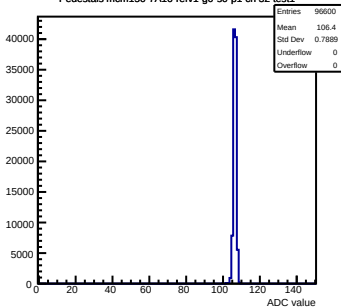
Pedestals mcm150-7A16-refv1-g0-s0-p1 ch 32 test1
