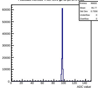
Pedestals mcm150-7A16-refv1-g0-s0-p1 ch 2 test1
