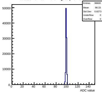
Pedestals mcm150-7A16-refv1-g0-s0-p1 ch 45 test1
