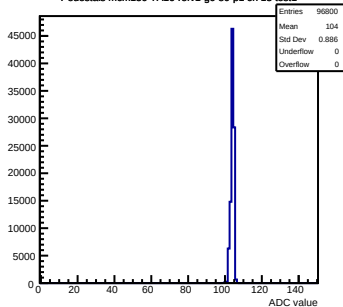
Pedestals mcm150-7A16-refv1-g0-s0-p1 ch 13 test1
