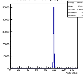
Pedestals mcm150-7A16-refv1-g0-s0-p1 ch 11 test1
