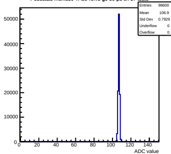
Pedestals mcm150-7A16-refv1-g0-s0-p1 ch 37 test1
