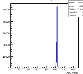
Pedestals mcm150-7A16-refv1-g0-s0-p1 ch 46 test1
