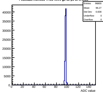
Pedestals mcm150-7A16-refv1-g0-s0-p1 ch 5 test1
