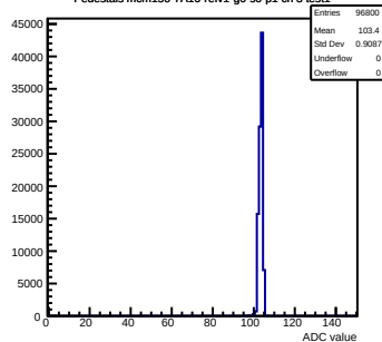
Pedestals mcm150-7A16-refv1-g0-s0-p1 ch 3 test1
