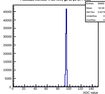
Pedestals mcm150-7A16-refv1-g0-s0-p1 ch 7 test1
