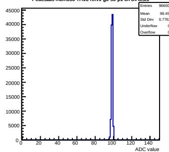
Pedestals mcm150-7A16-refv1-g0-s0-p1 ch 34 test1
