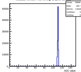
Pedestals mcm150-7A16-refv1-g0-s0-p1 ch 39 test1
