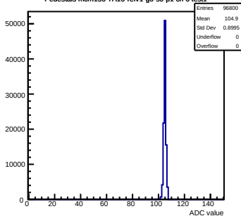
Pedestals mcm150-7A16-refv1-g0-s0-p1 ch 6 test1
