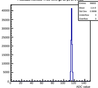
Pedestals mcm150-7A16-refv1-g0-s0-p1 ch 0 test1
