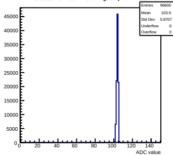
Pedestals mcm150-7A16-refv1-g0-s0-p1 ch 41 test1
