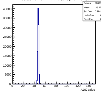
Pedestals mcm150-7A16-refv3-g0-s0-p1 ch 103 test1
