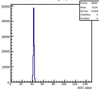
Pedestals mcm150-7A16-refv3-g0-s0-p1 ch 108 test1
