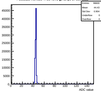
Pedestals mcm150-7A16-refv3-g0-s0-p1 ch 100 test1
