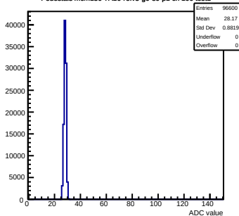
Pedestals mcm150-7A16-refv3-g0-s0-p1 ch 106 test1
