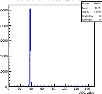
Pedestals mcm150-7A16-refv3-g0-s0-p1 ch 105 test1
