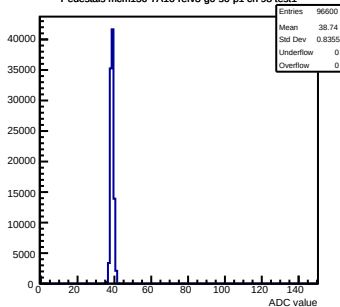
Pedestals mcm150-7A16-refv3-g0-s0-p1 ch 98 test1
