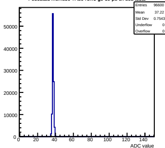
Pedestals mcm150-7A16-refv3-g0-s0-p1 ch 102 test1
