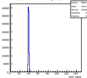
Pedestals mcm150-7A16-refv3-g0-s0-p1 ch 110 test1
