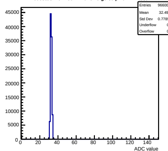
Pedestals mcm150-7A16-refv3-g0-s0-p1 ch 111 test1
