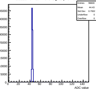
Pedestals mcm150-7A16-refv3-g0-s0-p1 ch 109 test1
