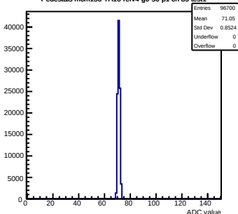
Pedestals mcm150-7A16-refv4-g0-s0-p1 ch 85 test1
