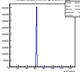
Pedestals mcm150-7A16-refv4-g0-s0-p1 ch 87 test1
