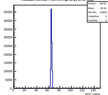
Pedestals mcm150-7A16-refv4-g0-s0-p1 ch 84 test1
