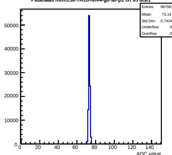
Pedestals mcm150-7A16-refv4-g0-s0-p1 ch 95 test1
