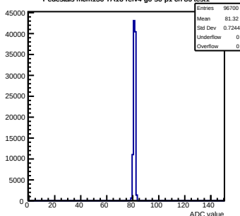
Pedestals mcm150-7A16-refv4-g0-s0-p1 ch 86 test1
