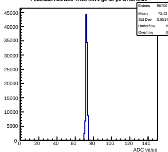
Pedestals mcm150-7A16-refv4-g0-s0-p1 ch 83 test1
