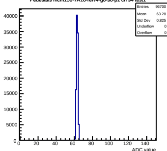
Pedestals mcm150-7A16-refv4-g0-s0-p1 ch 94 test1
