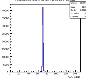
Pedestals mcm150-7A16-refv4-g0-s0-p1 ch 82 test1
