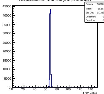
Pedestals mcm150-7A16-refv4-g0-s0-p1 ch 91 test1
