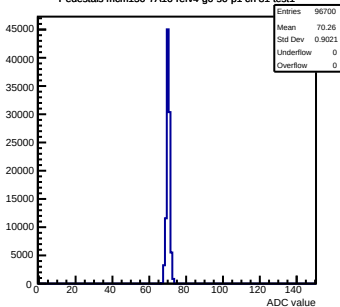
Pedestals mcm150-7A16-refv4-g0-s0-p1 ch 81 test1
