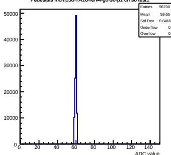
Pedestals mcm150-7A16-refv4-g0-s0-p1 ch 90 test1
