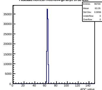
Pedestals mcm150-7A16-refv4-g0-s0-p1 ch 88 test1
