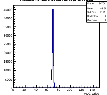
Pedestals mcm150-7A16-refv4-g0-s0-p1 ch 80 test1
