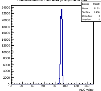
Pedestals mcm150-7A16-refV5-g0-s0-p1 ch 56 test1
