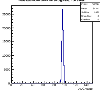
Pedestals mcm150-7A16-refV5-g0-s0-p1 ch 9 test1
