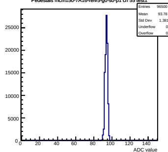
Pedestals mcm150-7A16-refV5-g0-s0-p1 ch 55 test1
