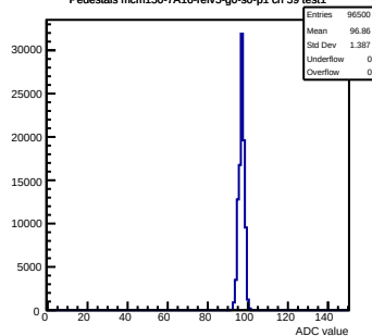
Pedestals mcm150-7A16-refV5-g0-s0-p1 ch 59 test1
