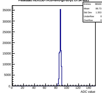
Pedestals mcm150-7A16-refV5-g0-s0-p1 ch 54 test1
