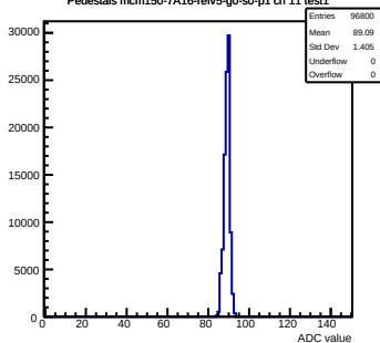
Pedestals mcm150-7A16-refV5-g0-s0-p1 ch 11 test1
