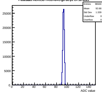
Pedestals mcm150-7A16-refV5-g0-s0-p1 ch 58 test1
