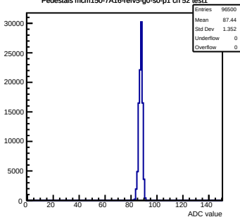
Pedestals mcm150-7A16-refV5-g0-s0-p1 ch 52 test1
