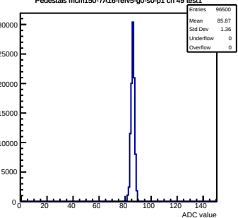
Pedestals mcm150-7A16-refV5-g0-s0-p1 ch 49 test1
