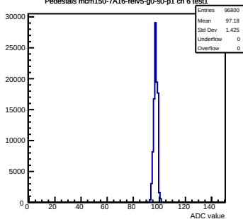
Pedestals mcm150-7A16-refV5-g0-s0-p1 ch 6 test1
