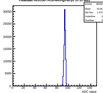
Pedestals mcm150-7A16-refV5-g0-s0-p1 ch 51 test1
