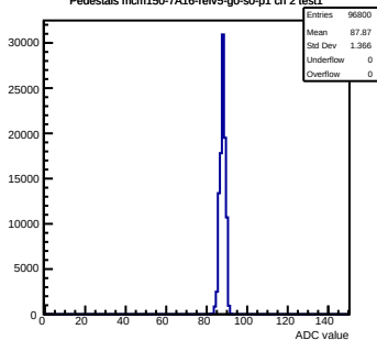
Pedestals mcm150-7A16-refV5-g0-s0-p1 ch 2 test1
