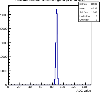
Pedestals mcm150-7A16-refV5-g0-s0-p1 ch 57 test1
