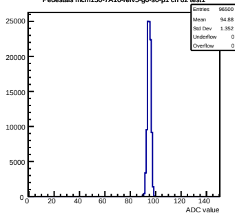
Pedestals mcm150-7A16-refV5-g0-s0-p1 ch 62 test1
