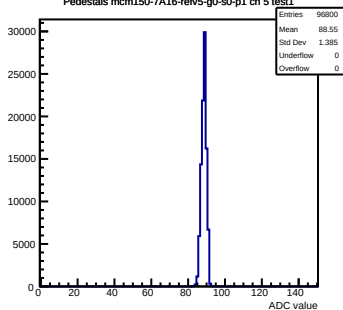
Pedestals mcm150-7A16-refV5-g0-s0-p1 ch 5 test1
