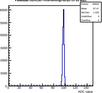
Pedestals mcm150-7A16-refV5-g0-s0-p1 ch 53 test1
