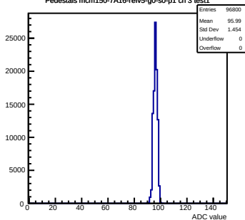
Pedestals mcm150-7A16-refV5-g0-s0-p1 ch 3 test1
