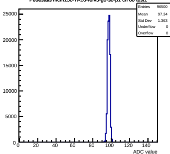
Pedestals mcm150-7A16-refV5-g0-s0-p1 ch 60 test1
