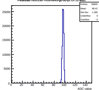
Pedestals mcm150-7A16-refV5-g0-s0-p1 ch 13 test1
