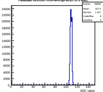
Pedestals mcm150-7A16-refV5-g0-s0-p1 ch 0 test1
