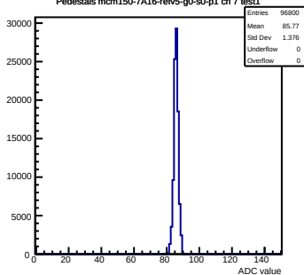
Pedestals mcm150-7A16-refV5-g0-s0-p1 ch 7 test1
