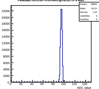
Pedestals mcm150-7A16-refV5-g0-s0-p1 ch 8 test1
