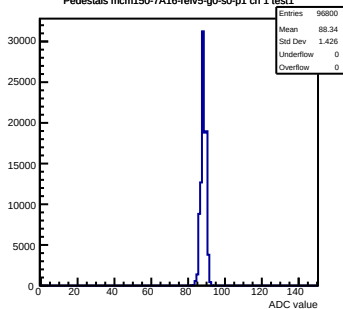
Pedestals mcm150-7A16-refV5-g0-s0-p1 ch 1 test1
