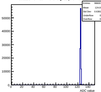
Pedestals mcm150-7A16-refv6-g0-s0-p1 ch 105 test1
