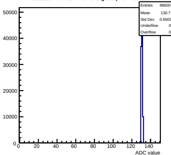
Pedestals mcm150-7A16-refv6-g0-s0-p1 ch 109 test1
