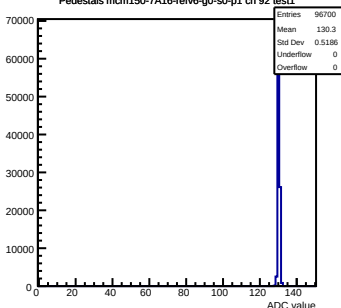
Pedestals mcm150-7A16-refv6-g0-s0-p1 ch 92 test1
