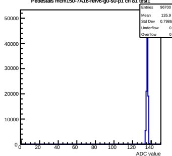
Pedestals mcm150-7A16-refv6-g0-s0-p1 ch 81 test1
