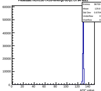
Pedestals mcm150-7A16-refv6-g0-s0-p1 ch 94 test1
