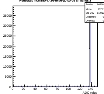
Pedestals mcm150-7A16-refv6-g0-s0-p1 ch 83 test1
