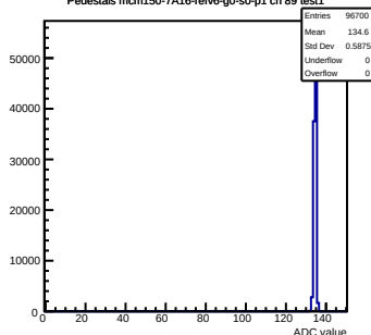
Pedestals mcm150-7A16-refv6-g0-s0-p1 ch 89 test1
