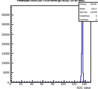
Pedestals mcm150-7A16-refv6-g0-s0-p1 ch 80 test1
