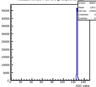
Pedestals mcm150-7A16-refv6-g0-s0-p1 ch 98 test1
