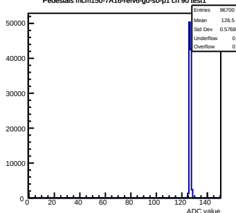
Pedestals mcm150-7A16-refv6-g0-s0-p1 ch 90 test1
