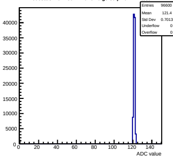
Pedestals mcm150-7A16-refv6-g0-s0-p1 ch 111 test1
