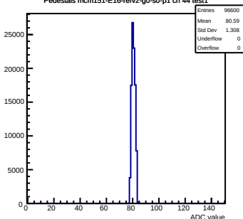
Pedestals mcm151-E16-refv2-g0-s0-p1 ch 44 test1
