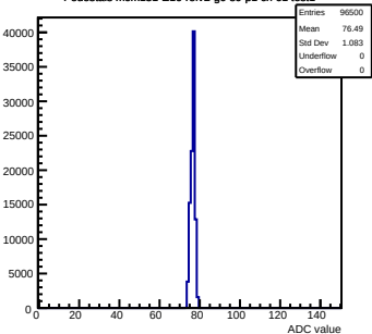
Pedestals mcm151-E16-refv2-g0-s0-p1 ch 61 test1
