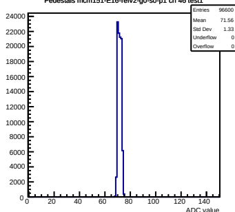
Pedestals mcm151-E16-refv2-g0-s0-p1 ch 46 test1
