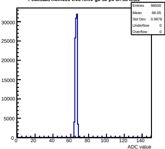
Pedestals mcm151-E16-refv2-g0-s0-p1 ch 53 test1
