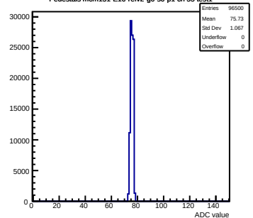
Pedestals mcm151-E16-refv2-g0-s0-p1 ch 55 test1
