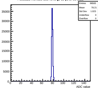
Pedestals mcm151-E16-refv2-g0-s0-p1 ch 56 test1
