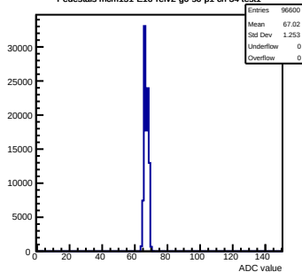
Pedestals mcm151-E16-refv2-g0-s0-p1 ch 34 test1
