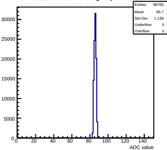
Pedestals mcm151-E16-refv2-g0-s0-p1 ch 84 test1
