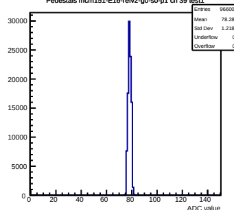
Pedestals mcm151-E16-refv2-g0-s0-p1 ch 39 test1
