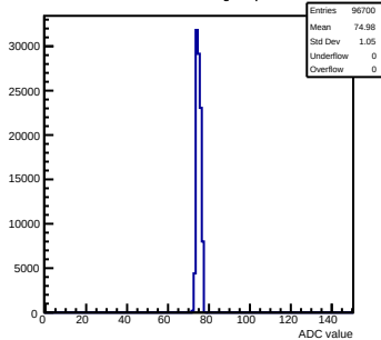
Pedestals mcm151-E16-refv2-g0-s0-p1 ch 89 test1
