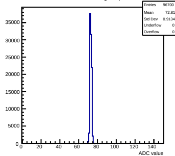
Pedestals mcm151-E16-refv2-g0-s0-p1 ch 95 test1
