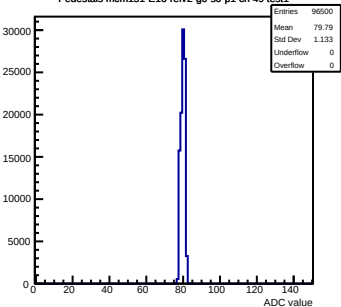
Pedestals mcm151-E16-refv2-g0-s0-p1 ch 49 test1
