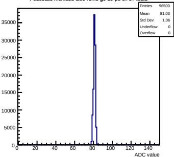
Pedestals mcm151-E16-refv2-g0-s0-p1 ch 57 test1
