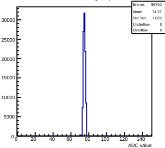
Pedestals mcm151-E16-refv2-g0-s0-p1 ch 88 test1
