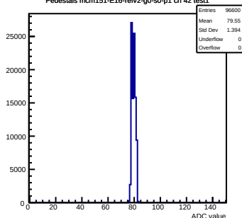
Pedestals mcm151-E16-refv2-g0-s0-p1 ch 42 test1
