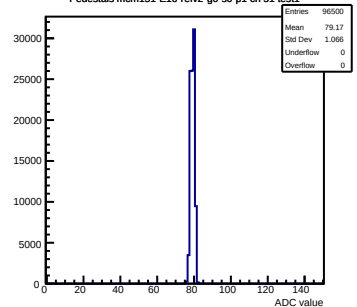
Pedestals mcm151-E16-refv2-g0-s0-p1 ch 51 test1
