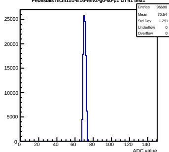
Pedestals mcm151-E16-refv2-g0-s0-p1 ch 41 test1
