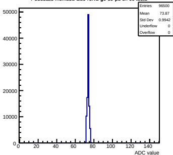
Pedestals mcm151-E16-refv2-g0-s0-p1 ch 60 test1
