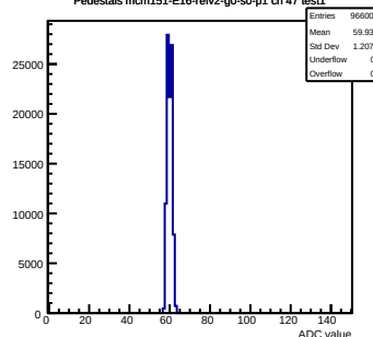
Pedestals mcm151-E16-refv2-g0-s0-p1 ch 47 test1
