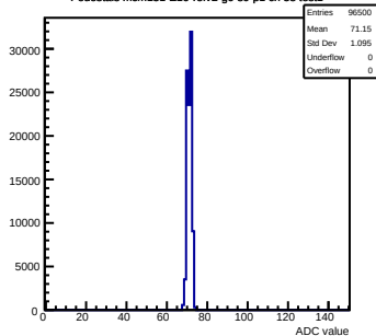
Pedestals mcm151-E16-refv2-g0-s0-p1 ch 58 test1
