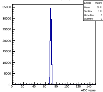
Pedestals mcm151-E16-refv2-g0-s0-p1 ch 90 test1
