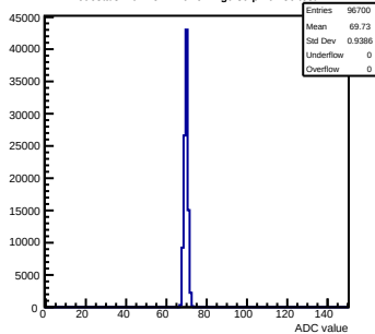
Pedestals mcm151-E16-refv2-g0-s0-p1 ch 86 test1
