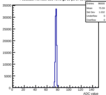
Pedestals mcm151-E16-refv2-g0-s0-p1 ch 62 test1
