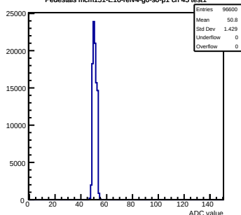
Pedestals mcm151-E16-refv4-g0-s0-p1 ch 45 test1
