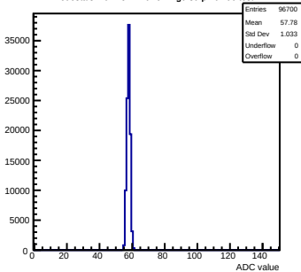
Pedestals mcm151-E16-refv4-g0-s0-p1 ch 90 test1
