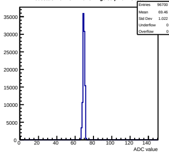
Pedestals mcm151-E16-refv4-g0-s0-p1 ch 23 test1
