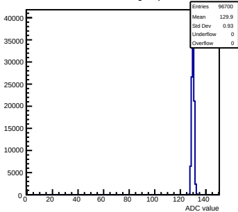
Pedestals mcm151-E16-refv6-g0-s0-p1 ch 28 test1
