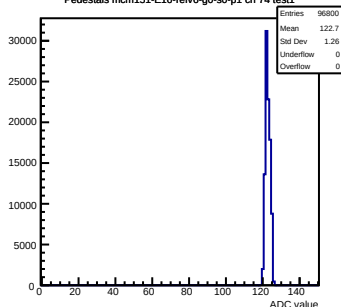
Pedestals mcm151-E16-refv6-g0-s0-p1 ch 74 test1
