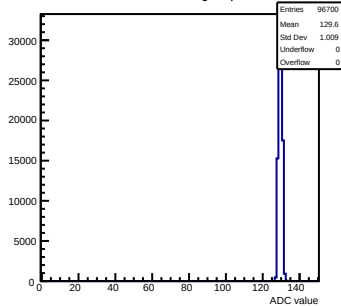
Pedestals mcm151-E16-refv6-g0-s0-p1 ch 31 test1
