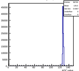
Pedestals mcm151-E16-refv6-g0-s0-p1 ch 94 test1
