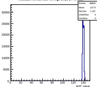
Pedestals mcm151-E16-refv6-g0-s0-p1 ch 76 test1
