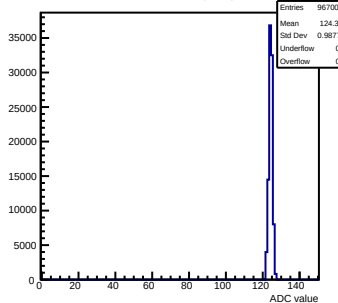
Pedestals mcm151-E16-refv6-g0-s0-p1 ch 83 test1
