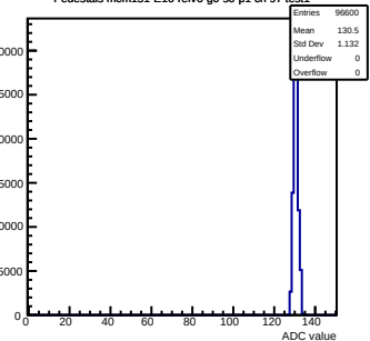
Pedestals mcm151-E16-refv6-g0-s0-p1 ch 97 test1
