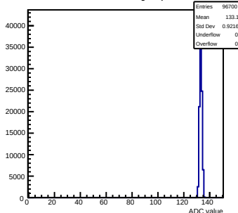
Pedestals mcm151-E16-refv6-g0-s0-p1 ch 93 test1
