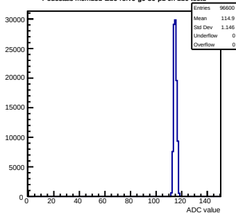
Pedestals mcm151-E16-refv6-g0-s0-p1 ch 110 test1
