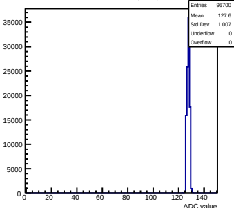
Pedestals mcm151-E16-refv6-g0-s0-p1 ch 86 test1
