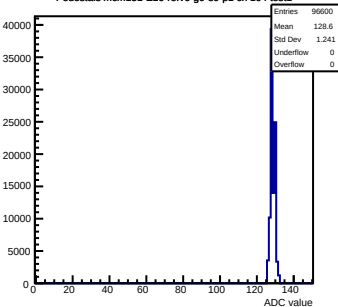
Pedestals mcm151-E16-refv6-g0-s0-p1 ch 104 test1
