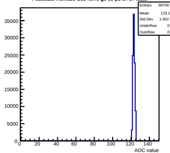
Pedestals mcm151-E16-refv6-g0-s0-p1 ch 17 test1
