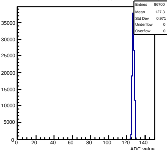
Pedestals mcm151-E16-refv6-g0-s0-p1 ch 92 test1
