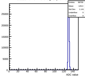
Pedestals mcm151-E16-refv6-g0-s0-p1 ch 20 test1
