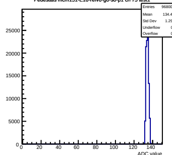
Pedestals mcm151-E16-refv6-g0-s0-p1 ch 75 test1
