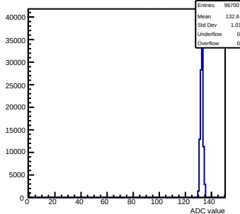
Pedestals mcm151-E16-refv6-g0-s0-p1 ch 81 test1
