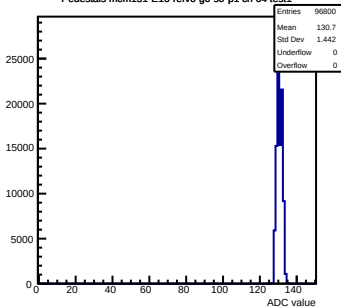
Pedestals mcm151-E16-refv6-g0-s0-p1 ch 64 test1
