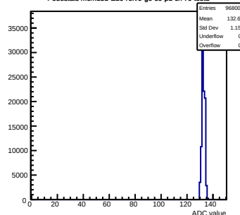
Pedestals mcm151-E16-refv6-g0-s0-p1 ch 79 test1
