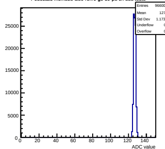
Pedestals mcm151-E16-refv6-g0-s0-p1 ch 111 test1
