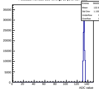
Pedestals mcm151-E16-refv6-g0-s0-p1 ch 107 test1
