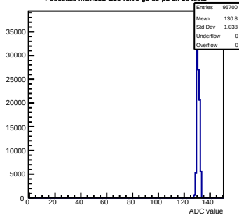
Pedestals mcm151-E16-refv6-g0-s0-p1 ch 18 test1
