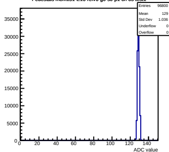
Pedestals mcm151-E16-refv6-g0-s0-p1 ch 65 test1
