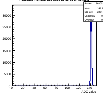
Pedestals mcm151-E16-refv6-g0-s0-p1 ch 66 test1
