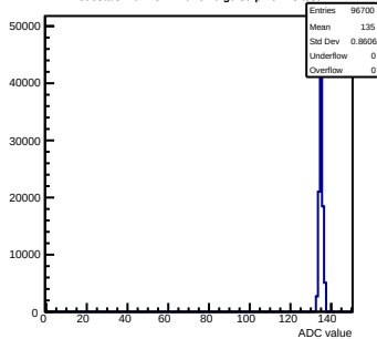
Pedestals mcm151-E16-refv6-g0-s0-p1 ch 23 test1
