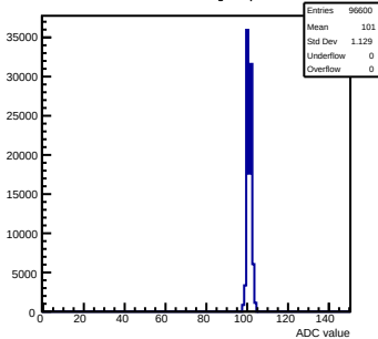
Pedestals mcm151-E16-refv1-g0-s0-p1 ch 104 test1
