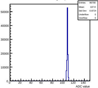
Pedestals mcm151-E16-refv1-g0-s0-p1 ch 91 test1
