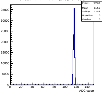
Pedestals mcm151-E16-refv1-g0-s0-p1 ch 48 test1
