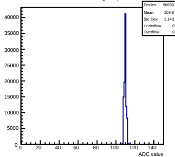
Pedestals mcm151-E16-refv1-g0-s0-p1 ch 102 test1
