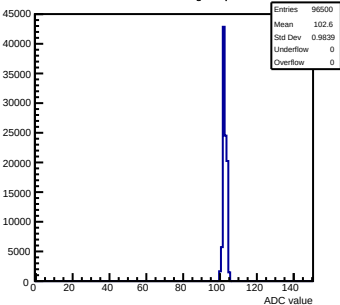
Pedestals mcm151-E16-refv1-g0-s0-p1 ch 60 test1
