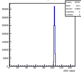
Pedestals mcm151-E16-refv1-g0-s0-p1 ch 89 test1
