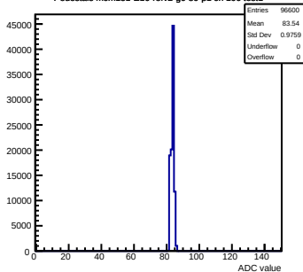
Pedestals mcm151-E16-refv2-g0-s0-p1 ch 102 test1
