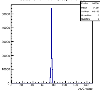
Pedestals mcm151-E16-refv2-g0-s0-p1 ch 100 test1
