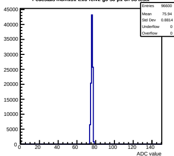
Pedestals mcm151-E16-refv2-g0-s0-p1 ch 98 test1
