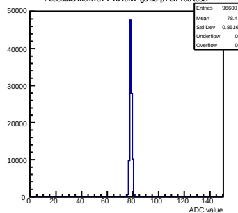
Pedestals mcm151-E16-refv2-g0-s0-p1 ch 99 test1
