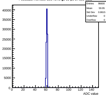
Pedestals mcm151-E16-refv2-g0-s0-p1 ch 110 test1
