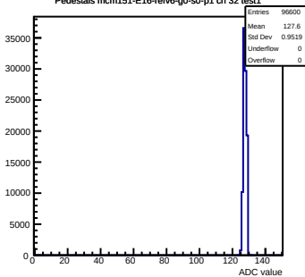
Pedestals mcm151-E16-refv6-g0-s0-p1 ch 32 test1
