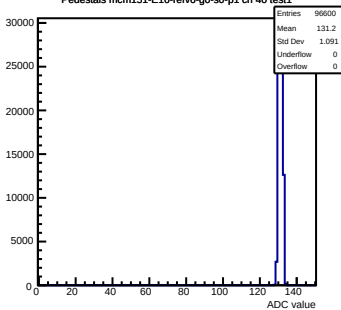
Pedestals mcm151-E16-refv6-g0-s0-p1 ch 40 test1
