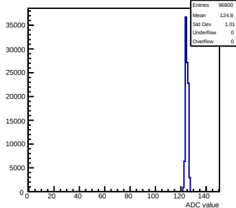
Pedestals mcm151-E16-refv6-g0-s0-p1 ch 14 test1
