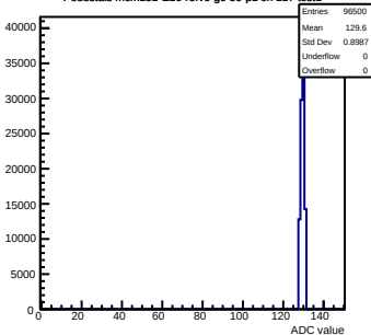
Pedestals mcm151-E16-relv6-g0-s0-p1 ch 117 test1
