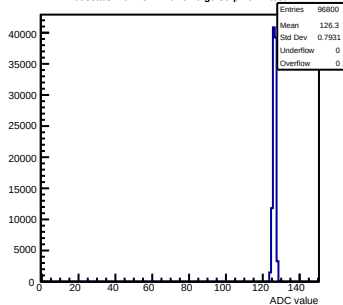
Pedestals mcm151-E16-refv6-g0-s0-p1 ch 2 test1
