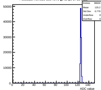
Pedestals mcm151-E16-refv6-g0-s0-p1 ch 53 test1
