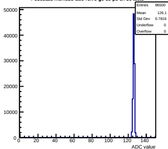
Pedestals mcm151-E16-refv6-g0-s0-p1 ch 50 test1
