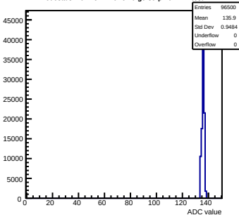
Pedestals mcm151-E16-relv6-g0-s0-p1 ch 127 test1
