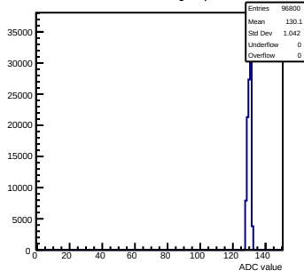
Pedestals mcm151-E16-refv6-g0-s0-p1 ch 10 test1
