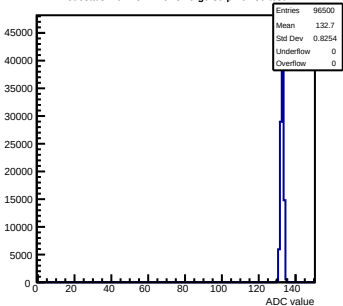
Pedestals mcm151-E16-refv6-g0-s0-p1 ch 59 test1
