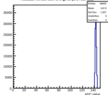
Pedestals mcm151-E16-refv6-g0-s0-p1 ch 109 test1
