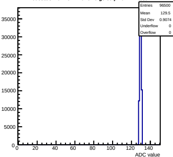
Pedestals mcm151-E16-relv6-g0-s0-p1 ch 124 test1
