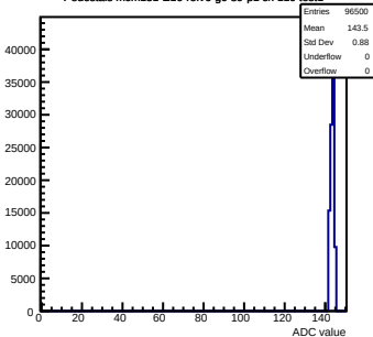
Pedestals mcm151-E16-relv6-g0-s0-p1 ch 119 test1
