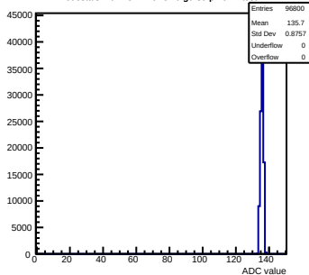
Pedestals mcm151-E16-refv6-g0-s0-p1 ch 1 test1
