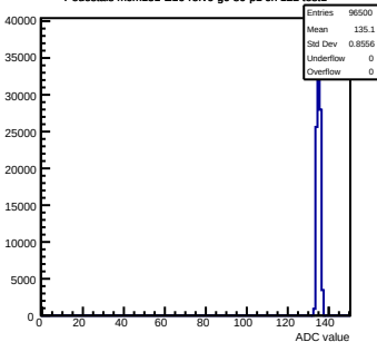
Pedestals mcm151-E16-relv6-g0-s0-p1 ch 122 test1
