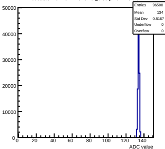
Pedestals mcm151-E16-relv6-g0-s0-p1 ch 125 test1
