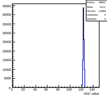
Pedestals mcm151-E16-refv6-g0-s0-p1 ch 13 test1
