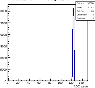
Pedestals mcm151-E16-refv6-g0-s0-p1 ch 45 test1
