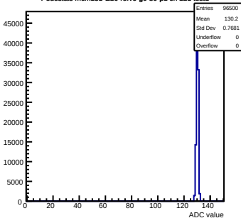
Pedestals mcm151-E16-relv6-g0-s0-p1 ch 121 test1
