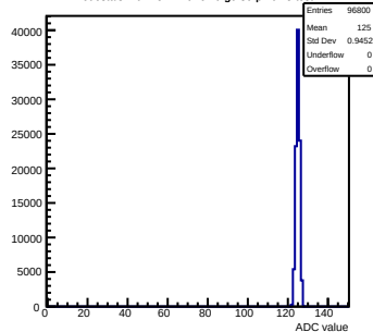
Pedestals mcm151-E16-refv6-g0-s0-p1 ch 3 test1
