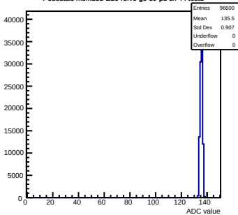
Pedestals mcm151-E16-refv6-g0-s0-p1 ch 44 test1
