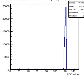
Pedestals mcm152-4E12-refV0-g0-s0-p1 ch 94 test1
