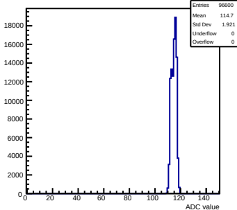
Pedestals mcm152-4E12-refV0-g0-s0-p1 ch 40 test1
