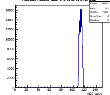
Pedestals mcm152-4E12-refV0-g0-s0-p1 ch 96 test1
