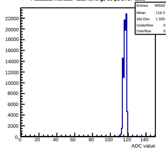
Pedestals mcm152-4E12-refV0-g0-s0-p1 ch 57 test1
