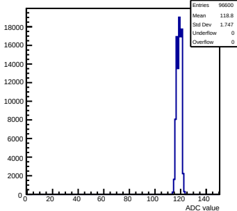
Pedestals mcm152-4E12-refV0-g0-s0-p1 ch 44 test1
