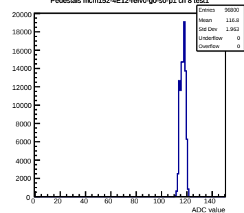
Pedestals mcm152-4E12-refV0-g0-s0-p1 ch 8 test1
