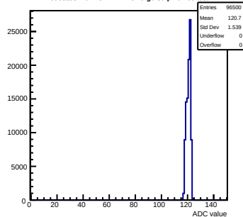
Pedestals mcm152-4E12-refV0-g0-s0-p1 ch 63 test1
