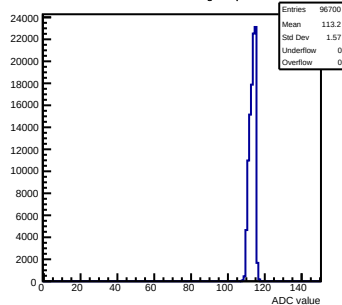
Pedestals mcm152-4E12-refV0-g0-s0-p1 ch 26 test1
