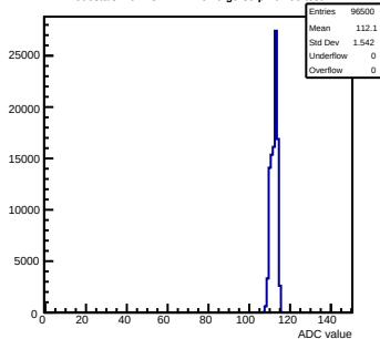
Pedestals mcm152-4E12-refV0-g0-s0-p1 ch 60 test1
