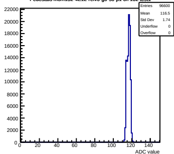
Pedestals mcm152-4E12-refV0-g0-s0-p1 ch 102 test1
