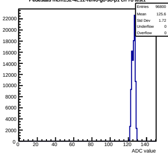
Pedestals mcm152-4E12-refV0-g0-s0-p1 ch 78 test1
