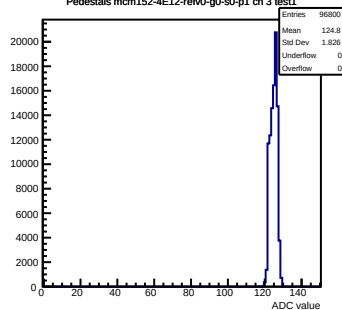
Pedestals mcm152-4E12-refV0-g0-s0-p1 ch 3 test1
