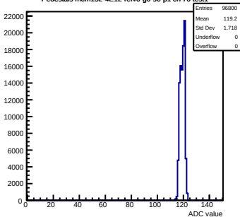
Pedestals mcm152-4E12-refV0-g0-s0-p1 ch 70 test1
