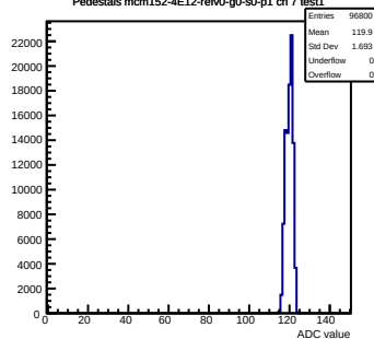
Pedestals mcm152-4E12-refV0-g0-s0-p1 ch 7 test1
