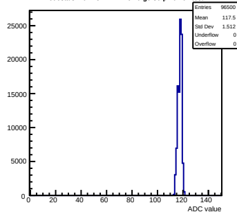
Pedestals mcm152-4E12-refV0-g0-s0-p1 ch 62 test1
