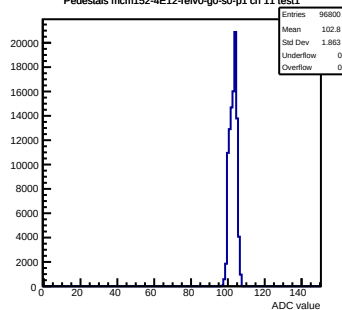
Pedestals mcm152-4E12-refV0-g0-s0-p1 ch 11 test1
