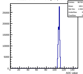
Pedestals mcm152-4E12-refV0-g0-s0-p1 ch 18 test1
