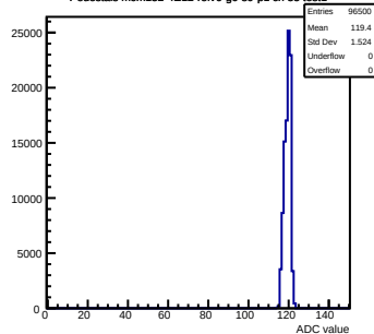
Pedestals mcm152-4E12-refV0-g0-s0-p1 ch 55 test1
