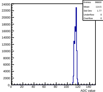
Pedestals mcm152-4E12-refV0-g0-s0-p1 ch 41 test1
