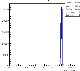
Pedestals mcm152-4E12-refV0-g0-s0-p1 ch 89 test1
