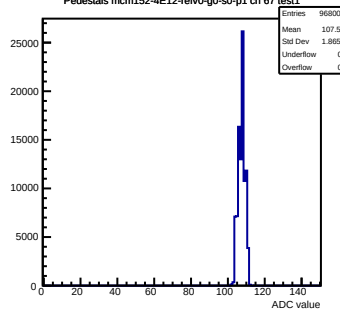
Pedestals mcm152-4E12-refV0-g0-s0-p1 ch 67 test1
