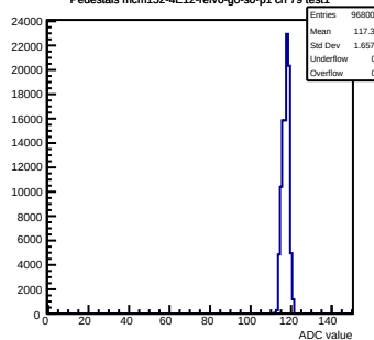
Pedestals mcm152-4E12-refV0-g0-s0-p1 ch 79 test1
