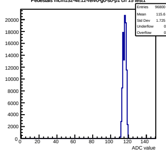
Pedestals mcm152-4E12-refV0-g0-s0-p1 ch 15 test1
