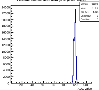
Pedestals mcm152-4E12-refV0-g0-s0-p1 ch 74 test1
