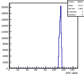
Pedestals mcm152-4E12-refV0-g0-s0-p1 ch 42 test1
