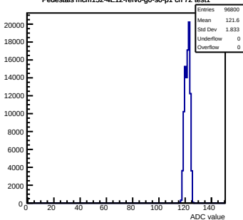
Pedestals mcm152-4E12-refV0-g0-s0-p1 ch 72 test1
