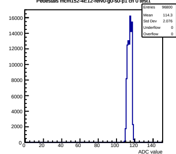
Pedestals mcm152-4E12-refV0-g0-s0-p1 ch 0 test1
