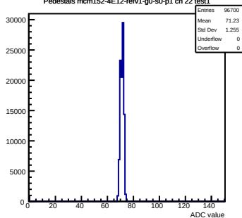
Pedestals mcm152-4E12-refv1-g0-s0-p1 ch 22 test1
