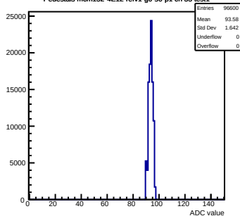
Pedestals mcm152-4E12-refv1-g0-s0-p1 ch 33 test1
