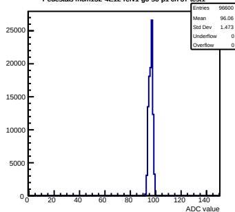
Pedestals mcm152-4E12-refv1-g0-s0-p1 ch 37 test1
