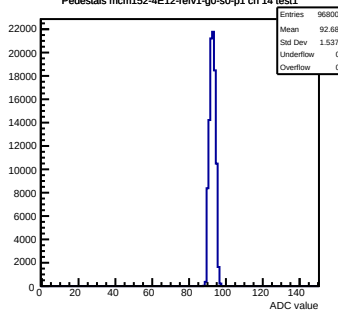
Pedestals mcm152-4E12-reV1-g0-s0-p1 ch 14 test1
