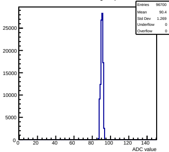
Pedestals mcm152-4E12-refv1-g0-s0-p1 ch 92 test1
