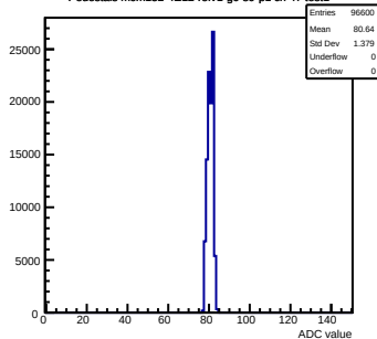
Pedestals mcm152-4E12-refv1-g0-s0-p1 ch 47 test1
