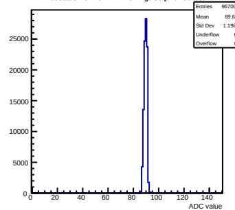
Pedestals mcm152-4E12-refv1-g0-s0-p1 ch 86 test1
