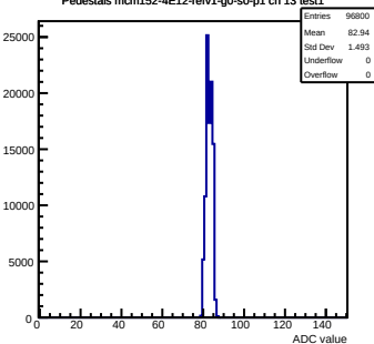
Pedestals mcm152-4E12-reV1-g0-s0-p1 ch 13 test1
