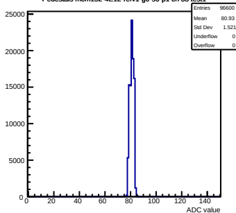
Pedestals mcm152-4E12-refv1-g0-s0-p1 ch 38 test1
