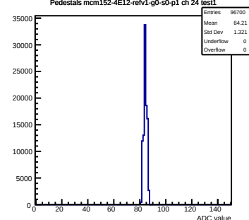
Pedestals mcm152-4E12-refv1-g0-s0-p1 ch 24 test1
