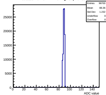
Pedestals mcm152-4E12-refv1-g0-s0-p1 ch 89 test1
