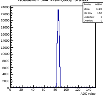
Pedestals mcm152-4E12-reV1-g0-s0-p1 ch 9 test1
