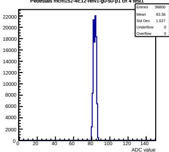
Pedestals mcm152-4E12-reV1-g0-s0-p1 ch 4 test1
