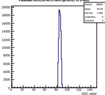
Pedestals mcm152-4E12-reV1-g0-s0-p1 ch 8 test1
