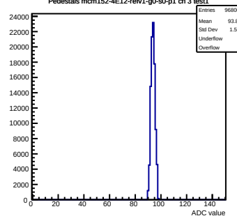
Pedestals mcm152-4E12-reV1-g0-s0-p1 ch 3 test1
