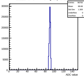
Pedestals mcm152-4E12-refv1-g0-s0-p1 ch 88 test1
