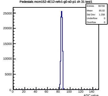
Pedestals mcm152-4E12-refv1-g0-s0-p1 ch 31 test1
