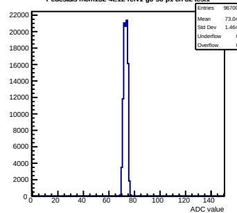
Pedestals mcm152-4E12-refv1-g0-s0-p1 ch 82 test1
