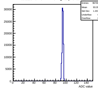
Pedestals mcm152-4E12-refv1-g0-s0-p1 ch 90 test1
