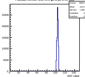
Pedestals mcm152-4E12-refv1-g0-s0-p1 ch 34 test1
