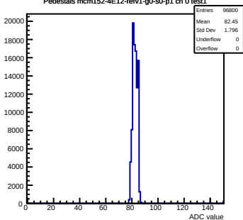
Pedestals mcm152-4E12-reV1-g0-s0-p1 ch 1 test1
