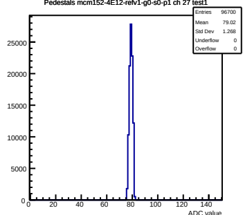
Pedestals mcm152-4E12-refv1-g0-s0-p1 ch 27 test1
