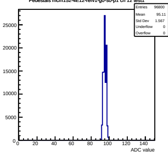
Pedestals mcm152-4E12-reV1-g0-s0-p1 ch 12 test1
