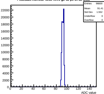
Pedestals mcm152-4E12-refv1-g0-s0-p1 ch 32 test1
