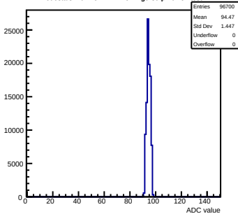
Pedestals mcm152-4E12-refv1-g0-s0-p1 ch 84 test1
