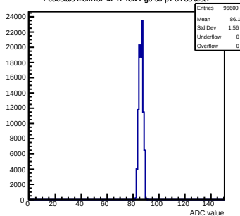
Pedestals mcm152-4E12-refv1-g0-s0-p1 ch 35 test1
