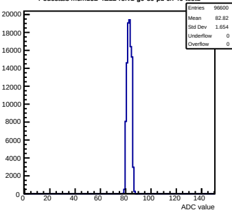
Pedestals mcm152-4E12-refv1-g0-s0-p1 ch 40 test1
