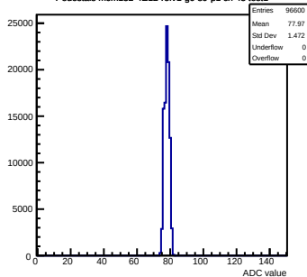
Pedestals mcm152-4E12-refv1-g0-s0-p1 ch 43 test1
