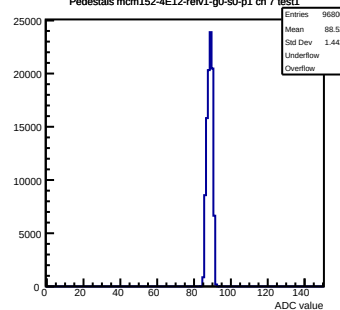
Pedestals mcm152-4E12-reV1-g0-s0-p1 ch 7 test1
