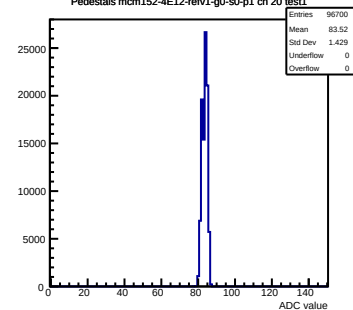
Pedestals mcm152-4E12-refv1-g0-s0-p1 ch 20 test1
