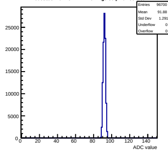
Pedestals mcm152-4E12-refv1-g0-s0-p1 ch 85 test1
