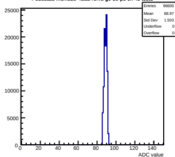
Pedestals mcm152-4E12-refv1-g0-s0-p1 ch 45 test1
