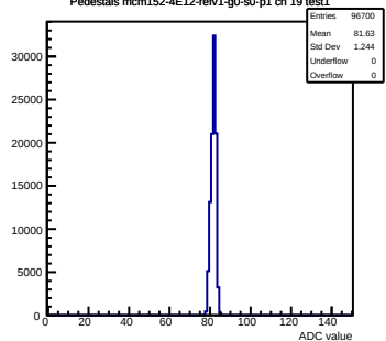
Pedestals mcm152-4E12-refv1-g0-s0-p1 ch 19 test1
