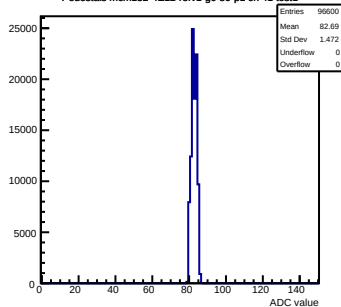
Pedestals mcm152-4E12-refv1-g0-s0-p1 ch 41 test1
