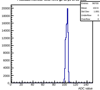
Pedestals mcm152-4E12-refv1-g0-s0-p1 ch 80 test1
