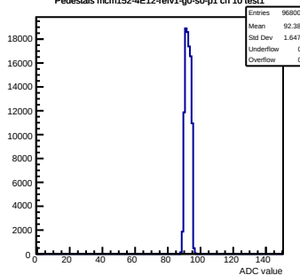
Pedestals mcm152-4E12-reV1-g0-s0-p1 ch 10 test1
