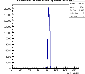
Pedestals mcm152-4E12-refv1-g0-s0-p1 ch 16 test1
