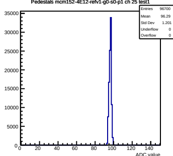
Pedestals mcm152-4E12-refv1-g0-s0-p1 ch 25 test1
