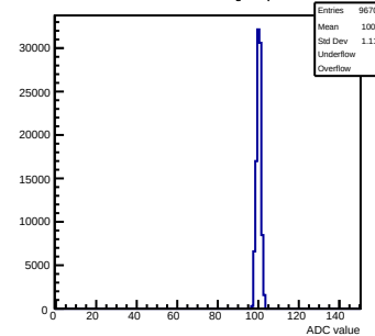
Pedestals mcm152-4E12-refv1-g0-s0-p1 ch 95 test1
