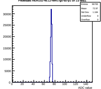
Pedestals mcm152-4E12-refv1-g0-s0-p1 ch 23 test1
