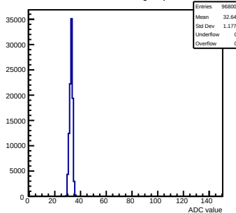
Pedestals mcm152-4E12-refv3-g0-s0-p1 ch 79 test1
