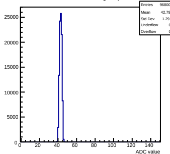
Pedestals mcm152-4E12-refv3-g0-s0-p1 ch 78 test1
