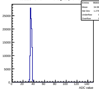
Pedestals mcm152-4E12-refv3-g0-s0-p1 ch 70 test1
