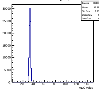
Pedestals mcm152-4E12-refv3-g0-s0-p1 ch 75 test1
