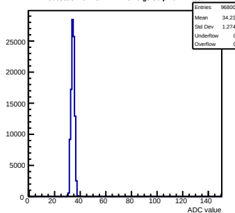
Pedestals mcm152-4E12-refv3-g0-s0-p1 ch 74 test1
