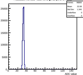
Pedestals mcm152-4E12-refv3-g0-s0-p1 ch 64 test1
