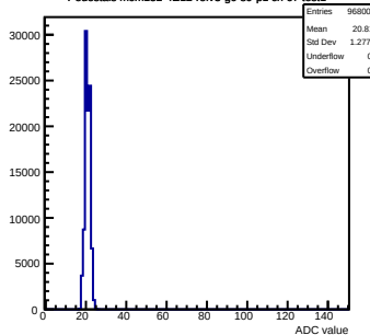
Pedestals mcm152-4E12-refv3-g0-s0-p1 ch 67 test1
