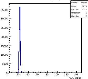
Pedestals mcm152-4E12-refv3-g0-s0-p1 ch 76 test1
