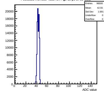
Pedestals mcm152-4E12-refv4-g0-s0-p1 ch 60 test1
