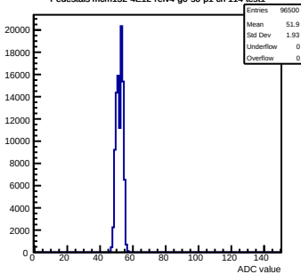
Pedestals mcm152-4E12-refV4-g0-s0-p1 ch 114 test1
