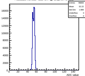
Pedestals mcm152-4E12-refv4-g0-s0-p1 ch 72 test1
