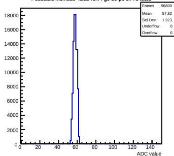
Pedestals mcm152-4E12-refv4-g0-s0-p1 ch 78 test1
