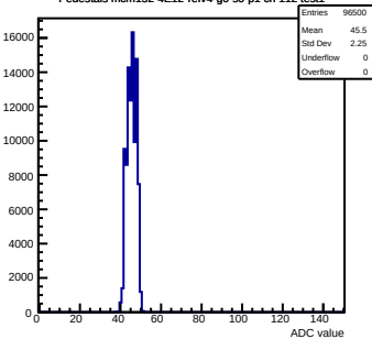
Pedestals mcm152-4E12-refV4-g0-s0-p1 ch 112 test1
