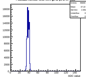
Pedestals mcm152-4E12-refv4-g0-s0-p1 ch 67 test1
