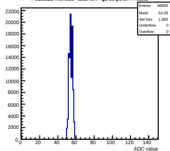
Pedestals mcm152-4E12-refv4-g0-s0-p1 ch 77 test1
