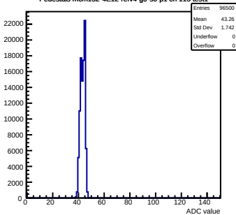
Pedestals mcm152-4E12-refV4-g0-s0-p1 ch 115 test1
