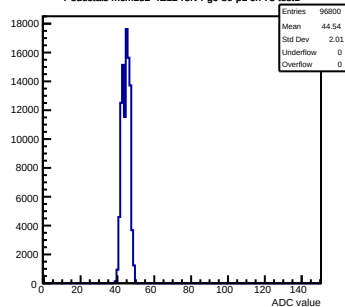
Pedestals mcm152-4E12-refv4-g0-s0-p1 ch 73 test1
