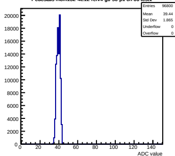
Pedestals mcm152-4E12-refv4-g0-s0-p1 ch 66 test1
