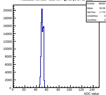
Pedestals mcm152-4E12-refv4-g0-s0-p1 ch 63 test1
