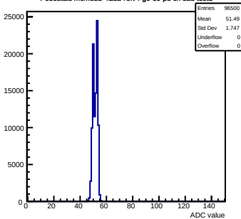
Pedestals mcm152-4E12-refV4-g0-s0-p1 ch 122 test1
