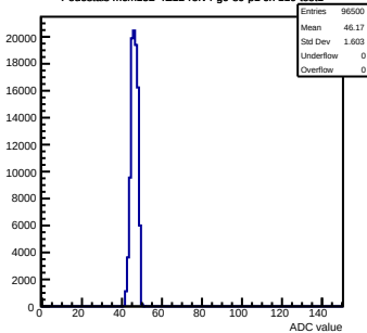
Pedestals mcm152-4E12-refV4-g0-s0-p1 ch 119 test1
