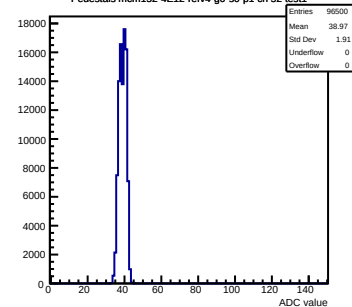
Pedestals mcm152-4E12-refv4-g0-s0-p1 ch 52 test1
