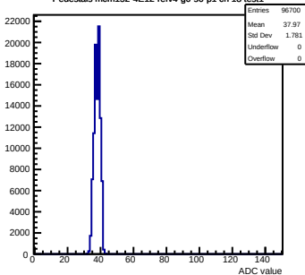
Pedestals mcm152-4E12-refv4-g0-s0-p1 ch 18 test1
