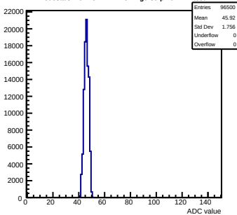
Pedestals mcm152-4E12-refV4-g0-s0-p1 ch 127 test1
