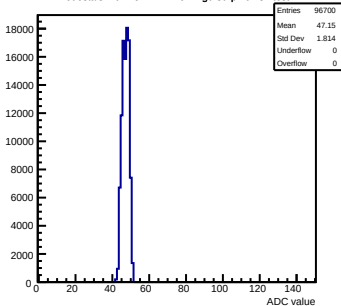
Pedestals mcm152-4E12-refv4-g0-s0-p1 ch 31 test1
