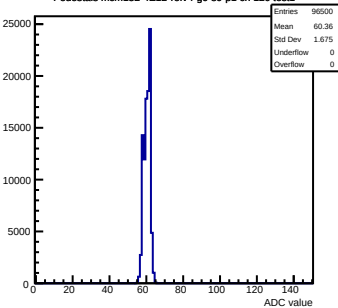
Pedestals mcm152-4E12-refV4-g0-s0-p1 ch 120 test1
