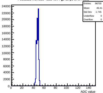
Pedestals mcm152-4E12-refv4-g0-s0-p1 ch 24 test1
