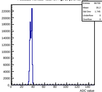
Pedestals mcm152-4E12-refv4-g0-s0-p1 ch 23 test1
