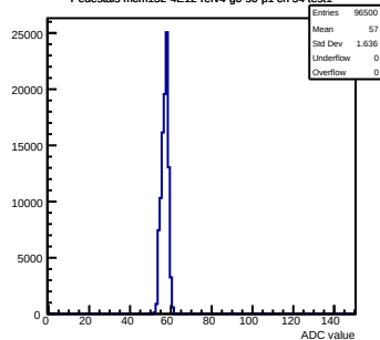
Pedestals mcm152-4E12-refv4-g0-s0-p1 ch 54 test1
