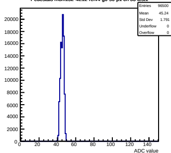
Pedestals mcm152-4E12-refv4-g0-s0-p1 ch 53 test1
