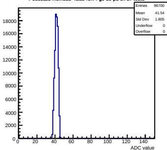
Pedestals mcm152-4E12-refv4-g0-s0-p1 ch 27 test1
