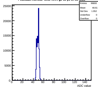
Pedestals mcm152-4E12-refv4-g0-s0-p1 ch 65 test1
