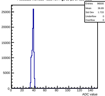
Pedestals mcm152-4E12-refV4-g0-s0-p1 ch 121 test1
