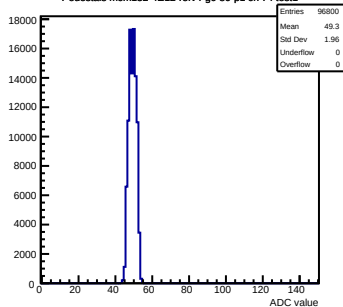
Pedestals mcm152-4E12-refv4-g0-s0-p1 ch 74 test1
