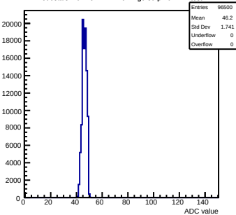
Pedestals mcm152-4E12-refV4-g0-s0-p1 ch 124 test1
