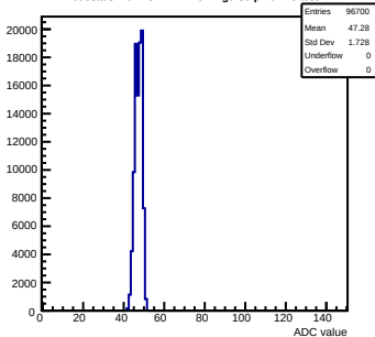
Pedestals mcm152-4E12-refv4-g0-s0-p1 ch 28 test1
