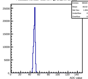
Pedestals mcm152-4E12-refv4-g0-s0-p1 ch 62 test1
