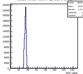
Pedestals mcm152-4E12-refv4-g0-s0-p1 ch 58 test1
