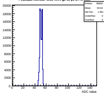
Pedestals mcm152-4E12-refv4-g0-s0-p1 ch 70 test1
