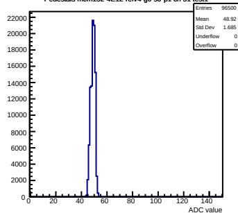
Pedestals mcm152-4E12-refv4-g0-s0-p1 ch 51 test1
