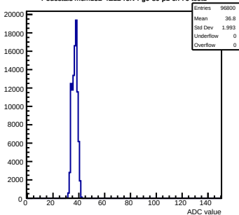
Pedestals mcm152-4E12-refv4-g0-s0-p1 ch 76 test1
