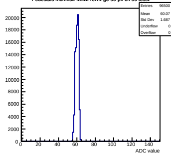
Pedestals mcm152-4E12-refv4-g0-s0-p1 ch 50 test1
