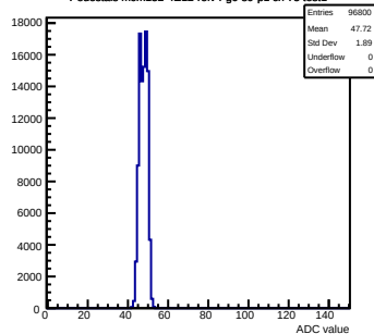
Pedestals mcm152-4E12-refv4-g0-s0-p1 ch 75 test1
