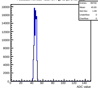
Pedestals mcm152-4E12-refv4-g0-s0-p1 ch 20 test1
