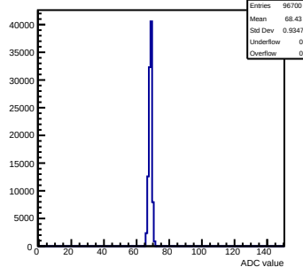
Pedestals mcm152-4E12-rtv5-g0-s0-p1 ch 23 test1
