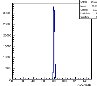
Pedestals mcm152-4E12-refV5-g0-s0-p1 ch 127 test1
