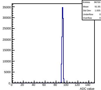
Pedestals mcm152-4E12-rtv5-g0-s0-p1 ch 25 test1
