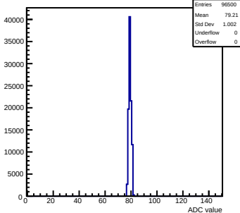
Pedestals mcm152-4E12-refV5-g0-s0-p1 ch 124 test1
