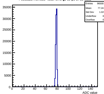
Pedestals mcm152-4E12-refV5-g0-s0-p1 ch 59 test1
