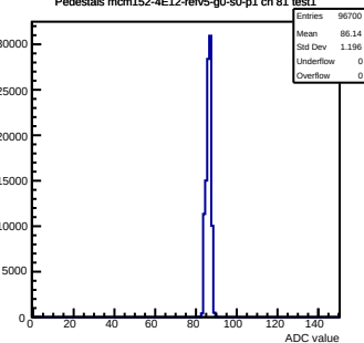
Pedestals mcm152-4E12-refv5-g0-s0-p1 ch 81 test1
