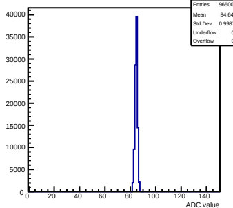
Pedestals mcm152-4E12-refV5-g0-s0-p1 ch 122 test1
