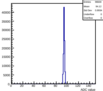
Pedestals mcm152-4E12-refV5-g0-s0-p1 ch 120 test1
