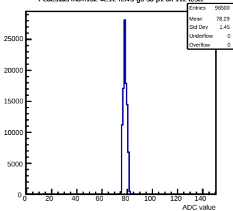
Pedestals mcm152-4E12-refV5-g0-s0-p1 ch 112 test1
