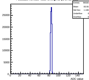
Pedestals mcm152-4E12-refV5-g0-s0-p1 ch 55 test1
