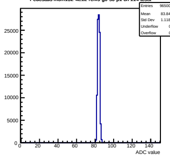
Pedestals mcm152-4E12-refV5-g0-s0-p1 ch 114 test1
