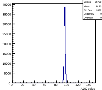
Pedestals mcm152-4E12-rtv5-g0-s0-p1 ch 30 test1
