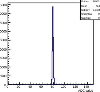
Pedestals mcm152-4E12-refV5-g0-s0-p1 ch 117 test1
