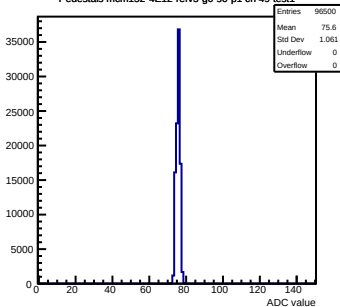
Pedestals mcm152-4E12-refV5-g0-s0-p1 ch 49 test1
