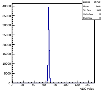
Pedestals mcm152-4E12-rtv5-g0-s0-p1 ch 22 test1
