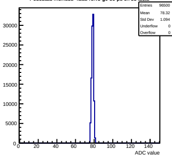
Pedestals mcm152-4E12-refV5-g0-s0-p1 ch 53 test1
