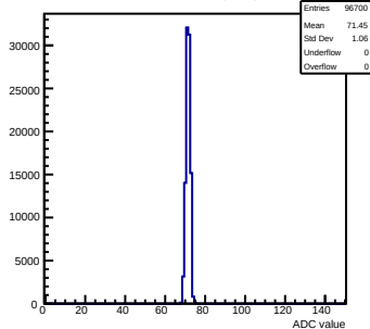
Pedestals mcm152-4E12-rtv5-g0-s0-p1 ch 18 test1
