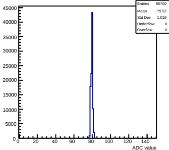
Pedestals mcm152-4E12-rtv5-g0-s0-p1 ch 24 test1
