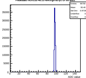
Pedestals mcm152-4E12-refv5-g0-s0-p1 ch 95 test1
