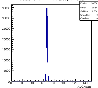
Pedestals mcm152-4E12-refV5-g0-s0-p1 ch 58 test1
