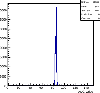
Pedestals mcm152-4E12-refV5-g0-s0-p1 ch 125 test1
