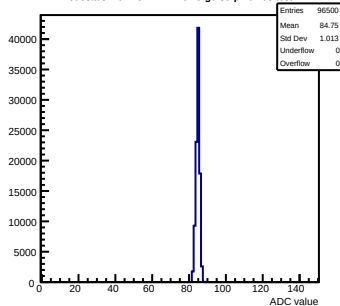
Pedestals mcm152-4E12-refV5-g0-s0-p1 ch 63 test1
