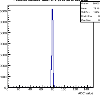
Pedestals mcm152-4E12-refV5-g0-s0-p1 ch 113 test1
