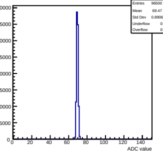
Pedestals mcm152-4E12-refV5-g0-s0-p1 ch 121 test1
