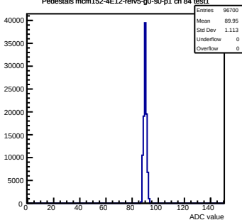
Pedestals mcm152-4E12-refv5-g0-s0-p1 ch 84 test1
