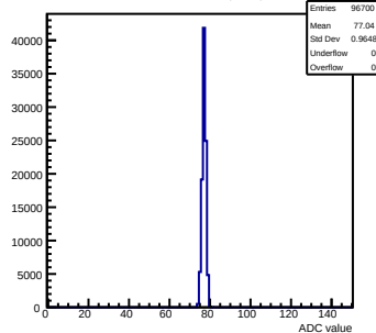
Pedestals mcm152-4E12-rtv5-g0-s0-p1 ch 19 test1
