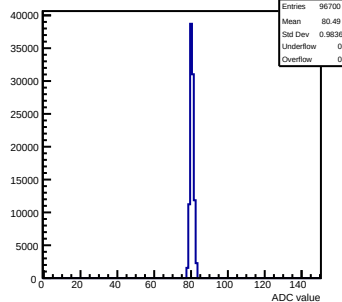
Pedestals mcm152-4E12-rtv5-g0-s0-p1 ch 31 test1
