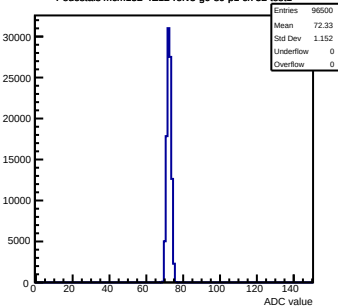
Pedestals mcm152-4E12-refV5-g0-s0-p1 ch 52 test1
