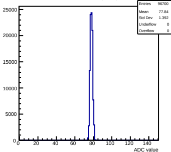
Pedestals mcm152-4E12-rtv5-g0-s0-p1 ch 16 test1
