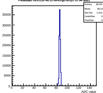
Pedestals mcm152-4E12-refv5-g0-s0-p1 ch 94 test1
