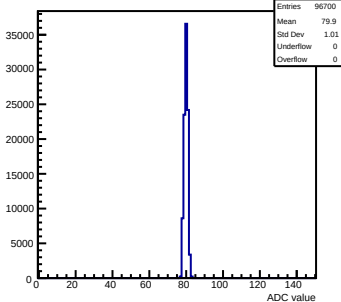
Pedestals mcm152-4E12-rtv5-g0-s0-p1 ch 28 test1
