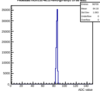
Pedestals mcm152-4E12-refv5-g0-s0-p1 ch 88 test1
