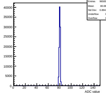
Pedestals mcm152-4E12-refV5-g0-s0-p1 ch 119 test1
