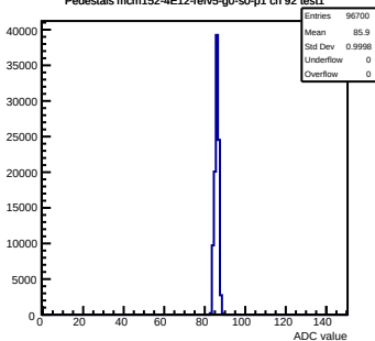
Pedestals mcm152-4E12-refv5-g0-s0-p1 ch 92 test1
