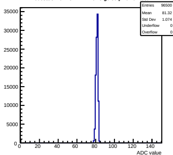
Pedestals mcm152-4E12-refV5-g0-s0-p1 ch 62 test1
