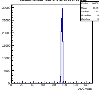
Pedestals mcm152-4E12-refV5-g0-s0-p1 ch 50 test1
