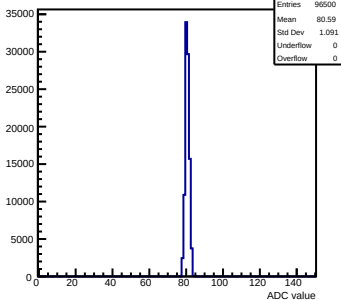
Pedestals mcm152-4E12-refV5-g0-s0-p1 ch 116 test1
