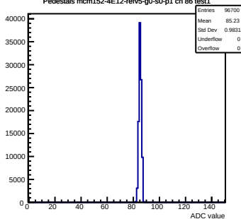
Pedestals mcm152-4E12-refv5-g0-s0-p1 ch 86 test1
