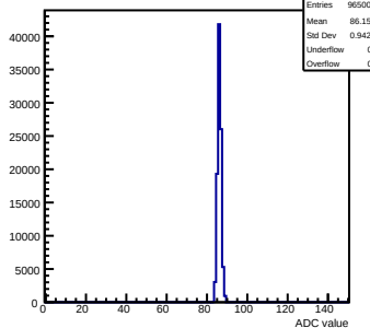
Pedestals mcm152-4E12-refV5-g0-s0-p1 ch 118 test1
