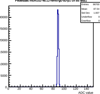
Pedestals mcm152-4E12-refv5-g0-s0-p1 ch 85 test1
