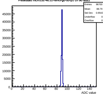
Pedestals mcm152-4E12-refv5-g0-s0-p1 ch 90 test1
