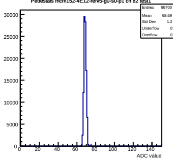
Pedestals mcm152-4E12-refv5-g0-s0-p1 ch 82 test1
