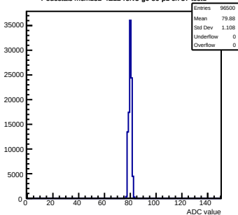
Pedestals mcm152-4E12-refV5-g0-s0-p1 ch 57 test1
