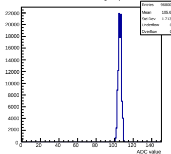
Pedestals mcm153-5E14-refV0-g0-s0-p1 ch 15 test1
