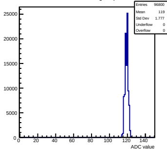
Pedestals mcm153-5E14-refV0-g0-s0-p1 ch 75 test1
