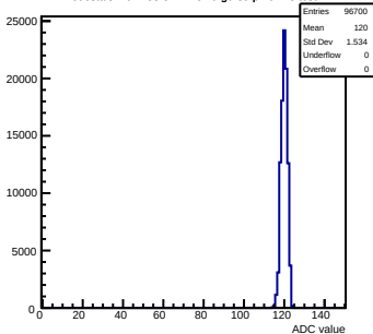
Pedestals mcm153-5E14-refV0-g0-s0-p1 ch 28 test1
