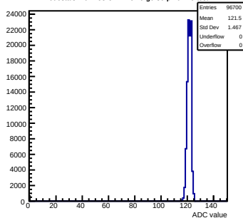
Pedestals mcm153-5E14-refV0-g0-s0-p1 ch 25 test1
