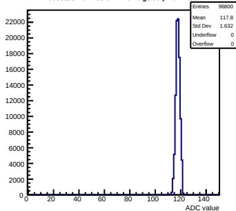
Pedestals mcm153-5E14-refV0-g0-s0-p1 ch 1 test1
