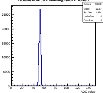
Pedestals mcm153-5E14-refv4-g0-s0-p1 ch 48 test1
