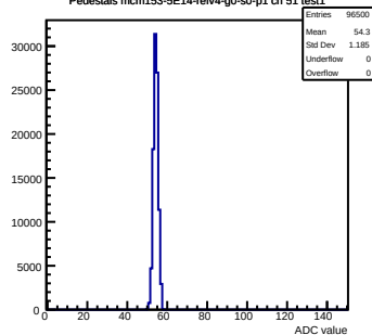
Pedestals mcm153-5E14-refv4-g0-s0-p1 ch 51 test1
