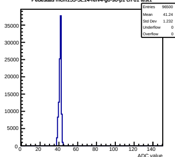
Pedestals mcm153-5E14-refv4-g0-s0-p1 ch 61 test1
