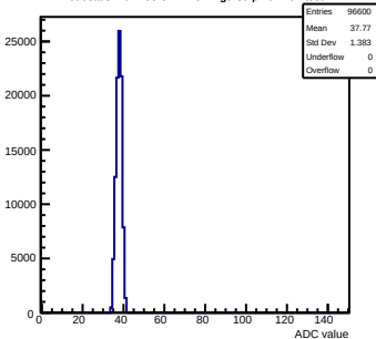
Pedestals mcm153-5E14-refv4-g0-s0-p1 ch 107 test1
