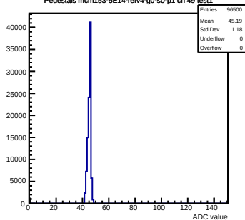
Pedestals mcm153-5E14-refv4-g0-s0-p1 ch 49 test1
