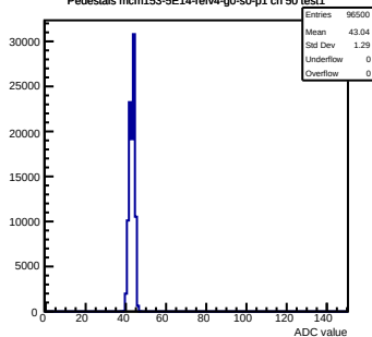
Pedestals mcm153-5E14-refv4-g0-s0-p1 ch 50 test1
