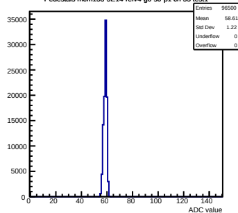
Pedestals mcm153-5E14-refv4-g0-s0-p1 ch 55 test1
