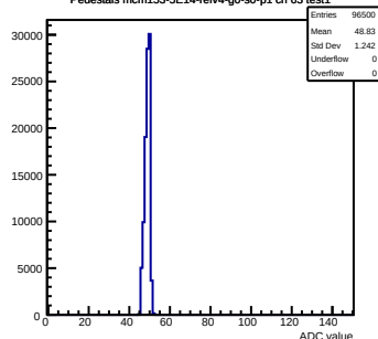
Pedestals mcm153-5E14-refv4-g0-s0-p1 ch 63 test1
