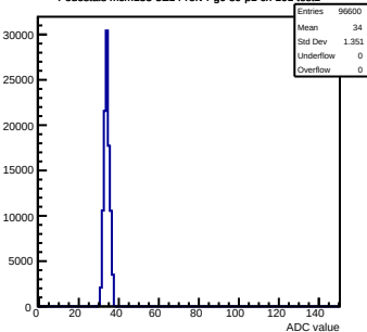
Pedestals mcm153-5E14-refv4-g0-s0-p1 ch 101 test1
