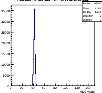
Pedestals mcm153-5E14-refv4-g0-s0-p1 ch 98 test1
