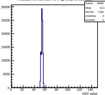
Pedestals mcm153-5E14-refv4-g0-s0-p1 ch 103 test1
