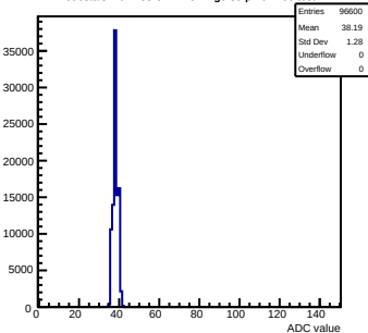
Pedestals mcm153-5E14-refv4-g0-s0-p1 ch 109 test1
