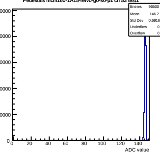
Pedestals mcm160-1A15-refV0-g0-s0-p1 ch 53 test1
