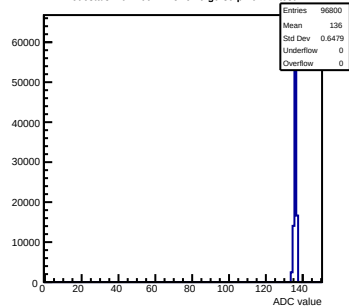
Pedestals mcm160-1A15-refV0-g0-s0-p1 ch 12 test1
