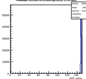
Pedestals mcm160-1A15-refV0-g0-s0-p1 ch 63 test1
