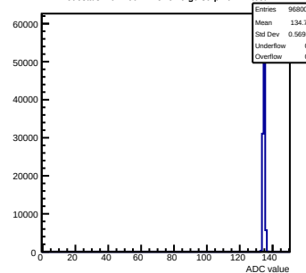
Pedestals mcm160-1A15-refV0-g0-s0-p1 ch 11 test1
