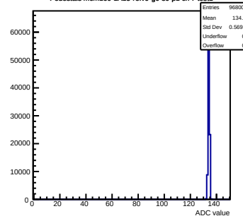
Pedestals mcm160-1A15-refV0-g0-s0-p1 ch 7 test1
