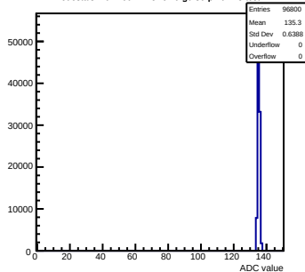
Pedestals mcm160-1A15-refV0-g0-s0-p1 ch 13 test1
