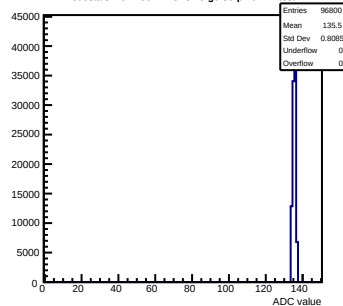
Pedestals mcm160-1A15-refV0-g0-s0-p1 ch 14 test1
