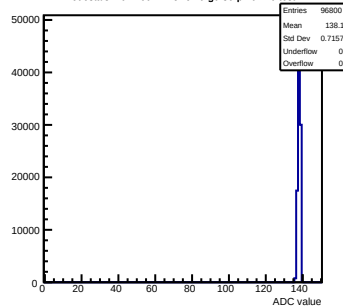
Pedestals mcm160-1A15-refV0-g0-s0-p1 ch 10 test1
