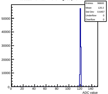
Pedestals mcm160-1A15-refv1-g0-s0-p1 ch 45 test1
