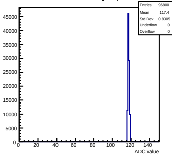
Pedestals mcm160-1A15-refv1-g0-s0-p1 ch 79 test1
