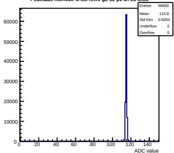
Pedestals mcm160-1A15-refv1-g0-s0-p1 ch 35 test1
