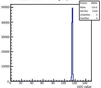
Pedestals mcm160-1A15-refv1-g0-s0-p1 ch 41 test1
