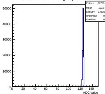
Pedestals mcm160-1A15-refv1-g0-s0-p1 ch 26 test1
