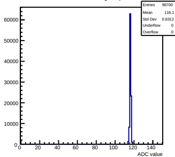
Pedestals mcm160-1A15-refv1-g0-s0-p1 ch 29 test1
