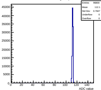
Pedestals mcm160-1A15-refv1-g0-s0-p1 ch 77 test1
