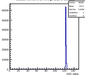
Pedestals mcm160-1A15-refv1-g0-s0-p1 ch 119 test1
