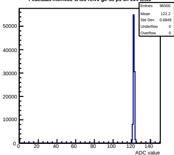
Pedestals mcm160-1A15-refv1-g0-s0-p1 ch 114 test1
