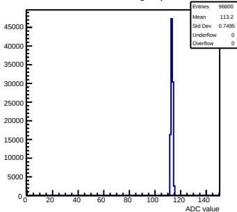
Pedestals mcm160-1A15-refv1-g0-s0-p1 ch 72 test1
