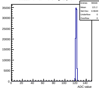
Pedestals mcm160-1A15-refv1-g0-s0-p1 ch 127 test1
