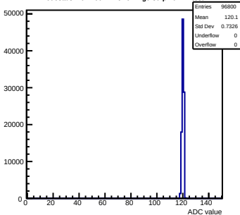
Pedestals mcm160-1A15-refv1-g0-s0-p1 ch 71 test1
