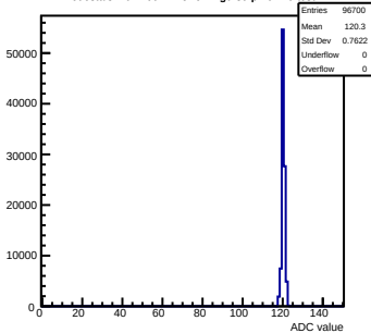
Pedestals mcm160-1A15-refv1-g0-s0-p1 ch 20 test1
