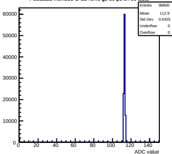
Pedestals mcm160-1A15-refv1-g0-s0-p1 ch 66 test1
