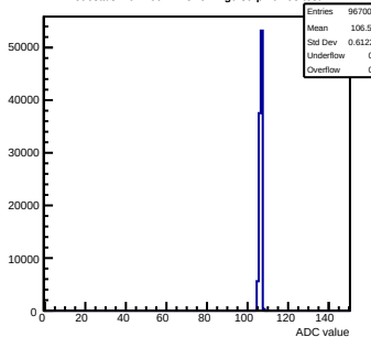
Pedestals mcm160-1A15-refv1-g0-s0-p1 ch 95 test1
