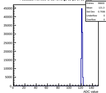
Pedestals mcm160-1A15-refv1-g0-s0-p1 ch 36 test1
