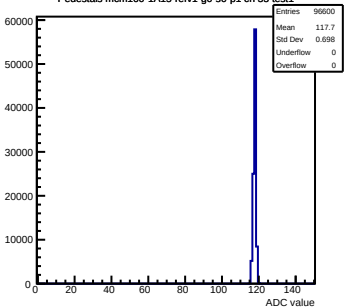
Pedestals mcm160-1A15-refv1-g0-s0-p1 ch 33 test1
