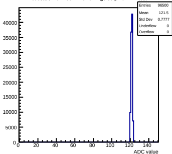
Pedestals mcm160-1A15-refv1-g0-s0-p1 ch 121 test1
