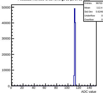
Pedestals mcm160-1A15-refv1-g0-s0-p1 ch 85 test1
