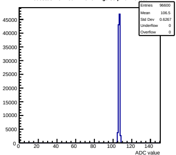
Pedestals mcm160-1A15-refv1-g0-s0-p1 ch 46 test1
