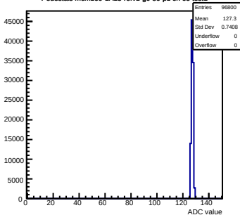
Pedestals mcm160-1A15-refv1-g0-s0-p1 ch 65 test1
