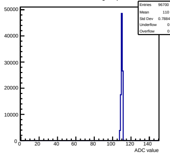
Pedestals mcm160-1A15-refv1-g0-s0-p1 ch 31 test1
