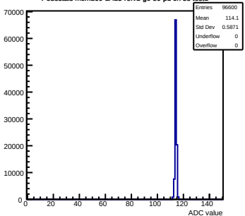
Pedestals mcm160-1A15-refv1-g0-s0-p1 ch 38 test1
