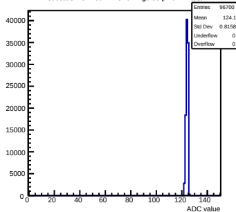
Pedestals mcm160-1A15-refv1-g0-s0-p1 ch 27 test1
