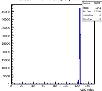
Pedestals mcm160-1A15-refv1-g0-s0-p1 ch 67 test1
