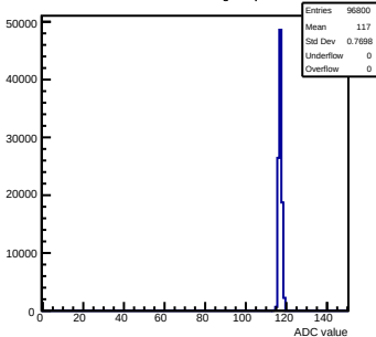
Pedestals mcm160-1A15-refv1-g0-s0-p1 ch 74 test1
