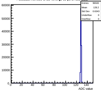
Pedestals mcm160-1A15-refv1-g0-s0-p1 ch 118 test1
