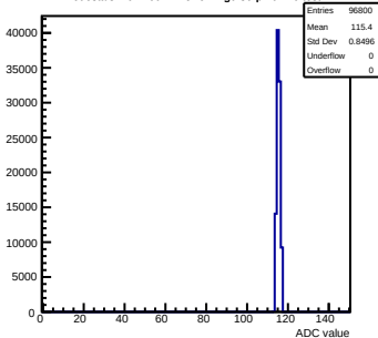
Pedestals mcm160-1A15-refv1-g0-s0-p1 ch 70 test1
