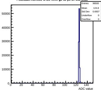
Pedestals mcm160-1A15-refv1-g0-s0-p1 ch 113 test1
