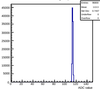
Pedestals mcm160-1A15-refv1-g0-s0-p1 ch 78 test1
