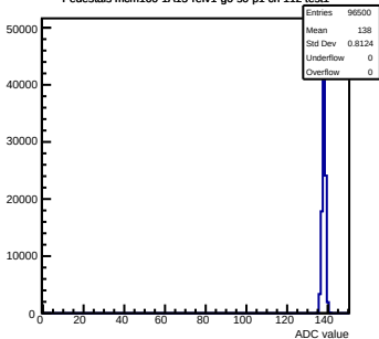
Pedestals mcm160-1A15-refv1-g0-s0-p1 ch 112 test1
