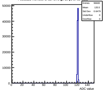
Pedestals mcm160-1A15-refv1-g0-s0-p1 ch 39 test1
