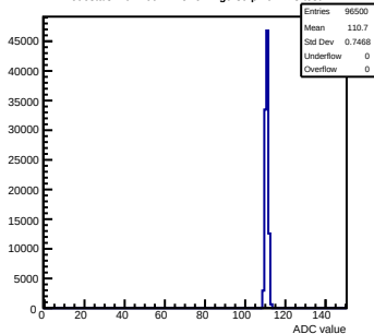
Pedestals mcm160-1A15-refv1-g0-s0-p1 ch 123 test1
