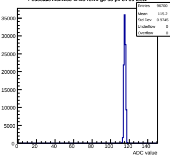
Pedestals mcm160-1A15-refv1-g0-s0-p1 ch 80 test1
