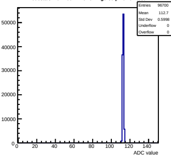
Pedestals mcm160-1A15-refv1-g0-s0-p1 ch 92 test1
