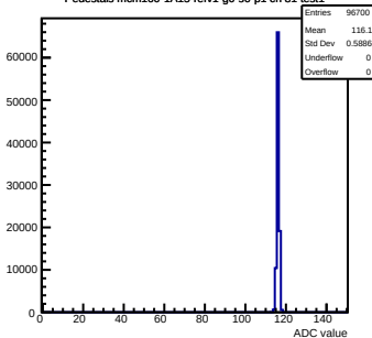
Pedestals mcm160-1A15-refv1-g0-s0-p1 ch 81 test1
