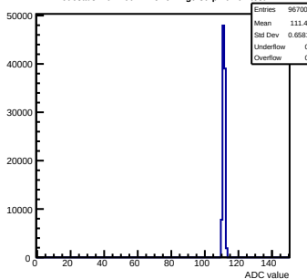
Pedestals mcm160-1A15-refv1-g0-s0-p1 ch 91 test1
