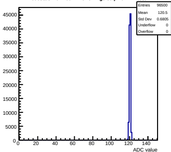
Pedestals mcm160-1A15-refv1-g0-s0-p1 ch 124 test1
