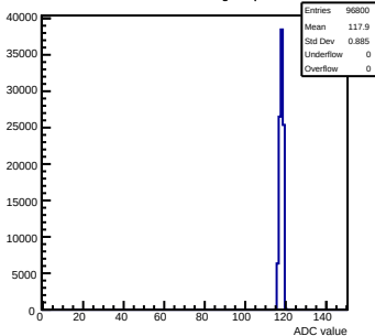
Pedestals mcm160-1A15-refv1-g0-s0-p1 ch 76 test1
