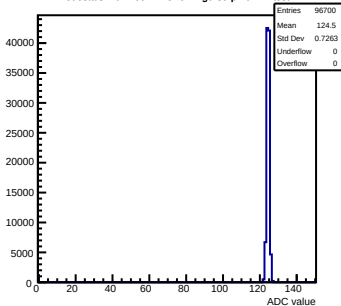
Pedestals mcm160-1A15-refv1-g0-s0-p1 ch 24 test1
