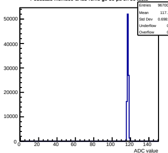
Pedestals mcm160-1A15-refv1-g0-s0-p1 ch 86 test1
