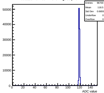
Pedestals mcm160-1A15-refv1-g0-s0-p1 ch 22 test1
