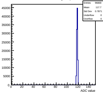
Pedestals mcm160-1A15-refv1-g0-s0-p1 ch 75 test1
