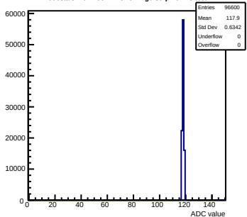
Pedestals mcm160-1A15-refv1-g0-s0-p1 ch 43 test1
