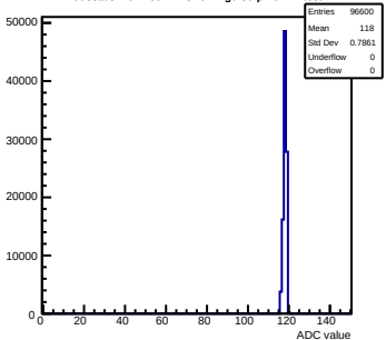
Pedestals mcm160-1A15-refv1-g0-s0-p1 ch 42 test1
