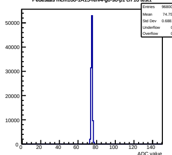
Pedestals mcm160-1A15-refv4-g0-s0-p1 ch 10 test1
