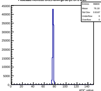
Pedestals mcm160-1A15-refv4-g0-s0-p1 ch 4 test1
