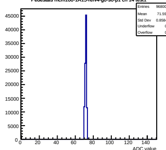
Pedestals mcm160-1A15-refv4-g0-s0-p1 ch 14 test1
