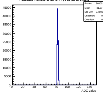
Pedestals mcm160-1A15-refv4-g0-s0-p1 ch 5 test1
