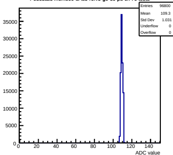
Pedestals mcm160-1A15-refV5-g0-s0-p1 ch 76 test1
