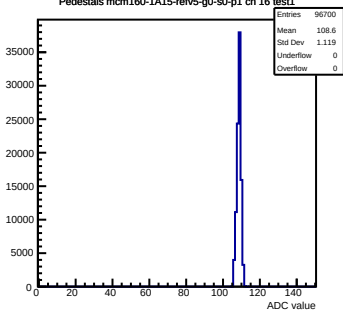
Pedestals mcm160-1A15-relv5-g0-s0-p1 ch 16 test1
