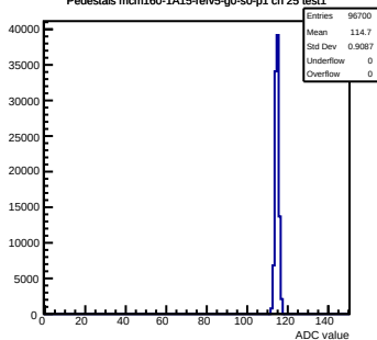
Pedestals mcm160-1A15-relv5-g0-s0-p1 ch 25 test1
