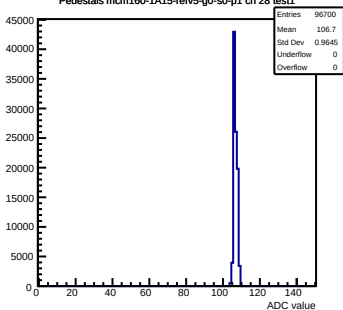
Pedestals mcm160-1A15-relv5-g0-s0-p1 ch 28 test1
