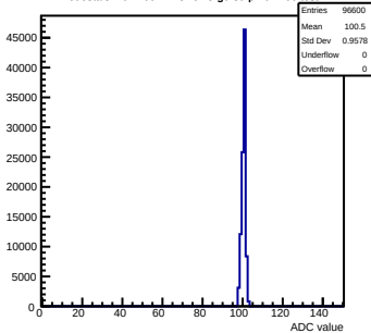
Pedestals mcm160-1A15-refV5-g0-s0-p1 ch 100 test1
