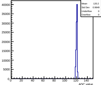
Pedestals mcm160-1A15-refV5-g0-s0-p1 ch 120 test1
