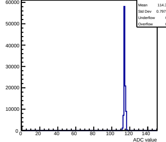
Pedestals mcm160-1A15-refV5-g0-s0-p1 ch 119 test1
