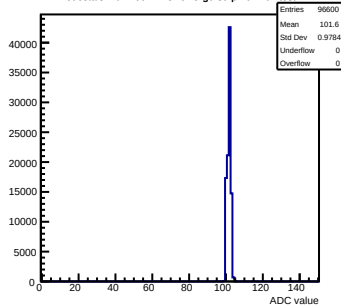
Pedestals mcm160-1A15-refV5-g0-s0-p1 ch 101 test1
