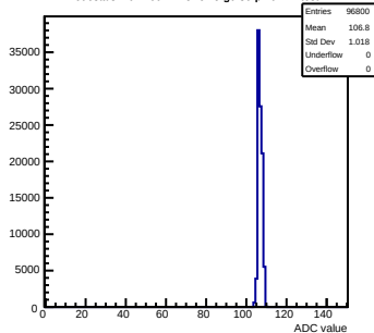
Pedestals mcm160-1A15-relV5-g0-s0-p1 ch 14 test1
