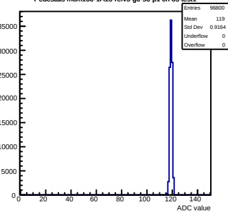
Pedestals mcm160-1A15-refV5-g0-s0-p1 ch 65 test1
