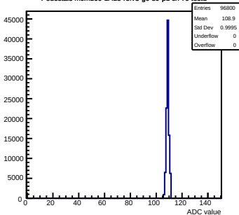
Pedestals mcm160-1A15-refV5-g0-s0-p1 ch 79 test1
