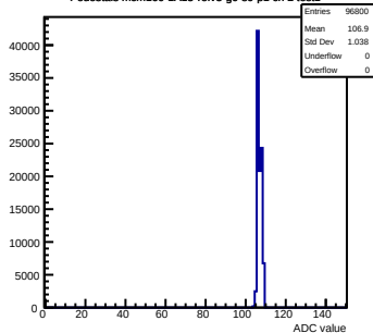
Pedestals mcm160-1A15-relV5-g0-s0-p1 ch 2 test1
