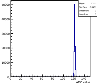
Pedestals mcm160-1A15-refV5-g0-s0-p1 ch 125 test1
