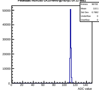
Pedestals mcm160-1A15-relv5-g0-s0-p1 ch 22 test1
