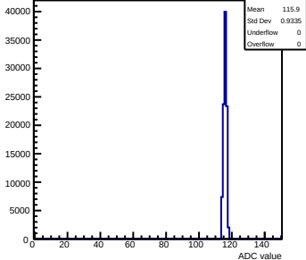
Pedestals mcm160-1A15-refV5-g0-s0-p1 ch 116 test1
