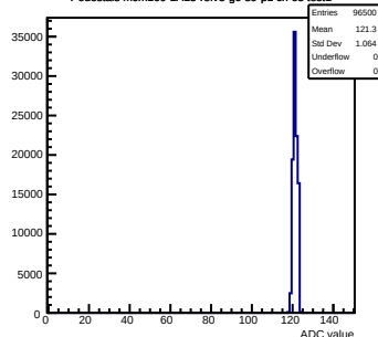
Pedestals mcm160-1A15-refV5-g0-s0-p1 ch 63 test1
