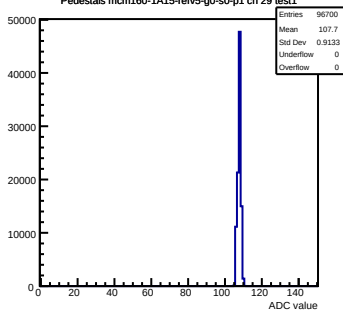
Pedestals mcm160-1A15-relv5-g0-s0-p1 ch 29 test1
