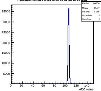
Pedestals mcm160-1A15-refV5-g0-s0-p1 ch 96 test1
