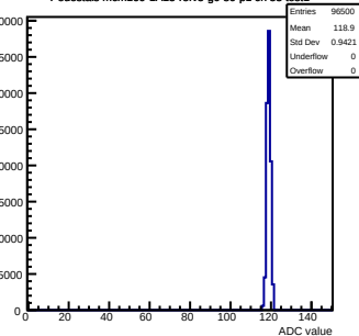
Pedestals mcm160-1A15-refV5-g0-s0-p1 ch 53 test1
