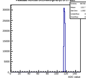
Pedestals mcm160-1A15-relv5-g0-s0-p1 ch 27 test1
