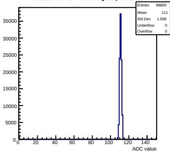
Pedestals mcm160-1A15-relV5-g0-s0-p1 ch 8 test1
