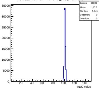
Pedestals mcm160-1A15-relV5-g0-s0-p1 ch 4 test1
