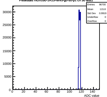
Pedestals mcm160-1A15-relv5-g0-s0-p1 ch 30 test1
