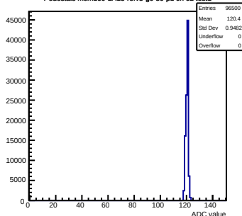
Pedestals mcm160-1A15-refV5-g0-s0-p1 ch 62 test1
