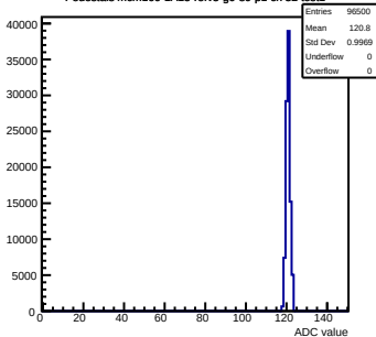
Pedestals mcm160-1A15-refV5-g0-s0-p1 ch 52 test1
