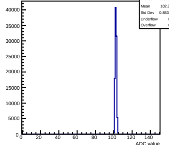
Pedestals mcm160-1A15-refV5-g0-s0-p1 ch 123 test1
