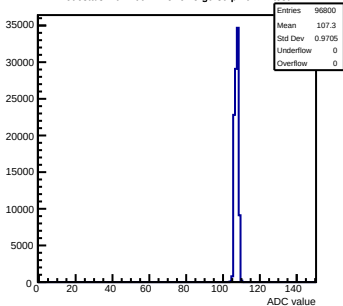
Pedestals mcm160-1A15-relV5-g0-s0-p1 ch 12 test1
