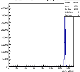
Pedestals mcm160-1A15-refV5-g0-s0-p1 ch 112 test1
