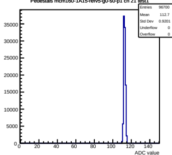
Pedestals mcm160-1A15-relv5-g0-s0-p1 ch 21 test1
