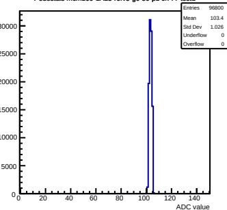
Pedestals mcm160-1A15-refV5-g0-s0-p1 ch 77 test1
