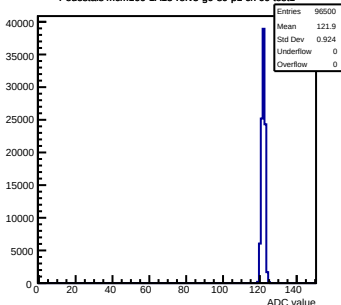
Pedestals mcm160-1A15-refV5-g0-s0-p1 ch 60 test1
