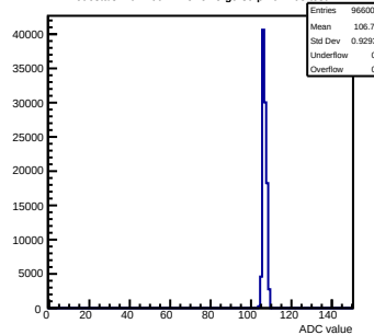
Pedestals mcm160-1A15-refV5-g0-s0-p1 ch 103 test1
