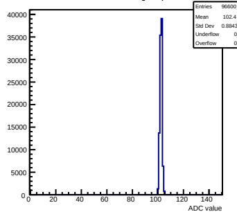
Pedestals mcm160-1A15-refV5-g0-s0-p1 ch 110 test1
