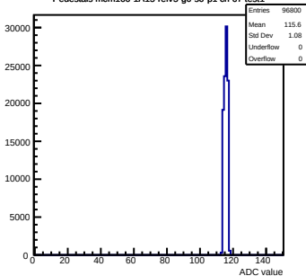
Pedestals mcm160-1A15-refV5-g0-s0-p1 ch 67 test1
