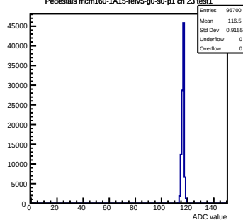
Pedestals mcm160-1A15-relv5-g0-s0-p1 ch 23 test1
