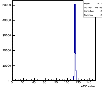
Pedestals mcm160-1A15-refV5-g0-s0-p1 ch 126 test1
