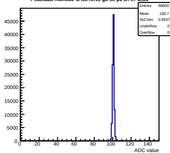
Pedestals mcm160-1A15-refV5-g0-s0-p1 ch 97 test1
