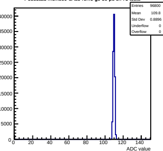
Pedestals mcm160-1A15-refV5-g0-s0-p1 ch 73 test1
