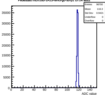
Pedestals mcm160-1A15-relv5-g0-s0-p1 ch 24 test1
