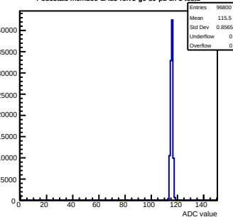
Pedestals mcm160-1A15-relV5-g0-s0-p1 ch 5 test1
