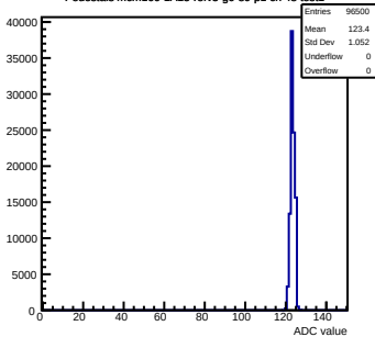
Pedestals mcm160-1A15-refV5-g0-s0-p1 ch 48 test1
