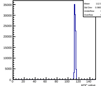
Pedestals mcm160-1A15-refV5-g0-s0-p1 ch 127 test1
