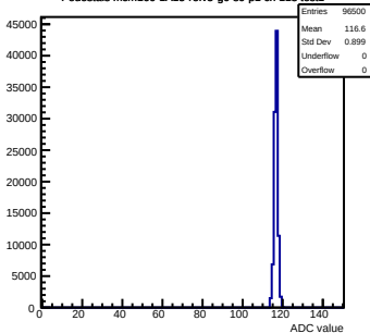
Pedestals mcm160-1A15-refV5-g0-s0-p1 ch 113 test1
