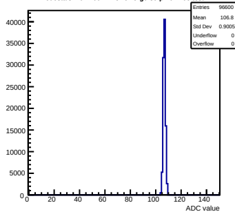
Pedestals mcm160-1A15-refV5-g0-s0-p1 ch 105 test1
