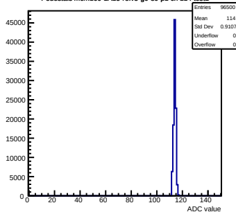
Pedestals mcm160-1A15-refV5-g0-s0-p1 ch 114 test1
