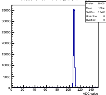
Pedestals mcm160-1A15-refV5-g0-s0-p1 ch 74 test1
