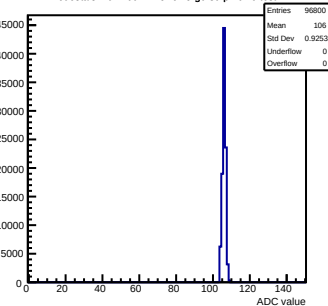
Pedestals mcm160-1A15-relV5-g0-s0-p1 ch 9 test1
