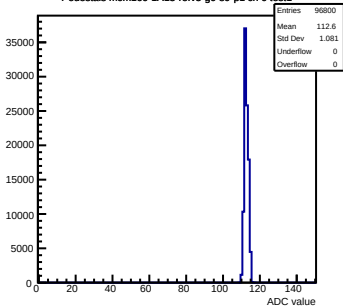
Pedestals mcm160-1A15-relV5-g0-s0-p1 ch 0 test1
