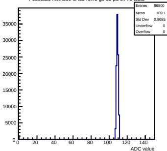
Pedestals mcm160-1A15-refV5-g0-s0-p1 ch 75 test1
