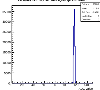
Pedestals mcm160-1A15-relv5-g0-s0-p1 ch 26 test1
