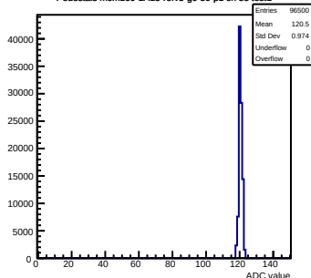
Pedestals mcm160-1A15-refV5-g0-s0-p1 ch 58 test1
