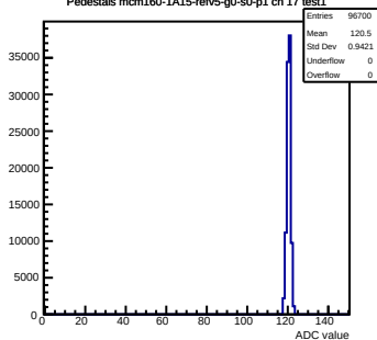
Pedestals mcm160-1A15-relv5-g0-s0-p1 ch 17 test1
