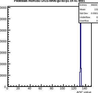
Pedestals mcm160-1A15-refv6-g0-s0-p1 ch 41 test1
