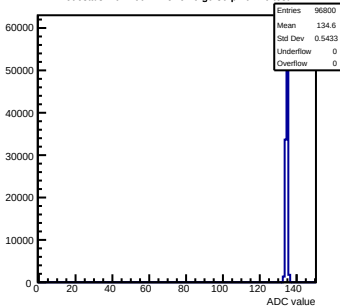
Pedestals mcm160-1A15-relv6-g0-s0-p1 ch 10 test1
