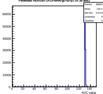
Pedestals mcm160-1A15-refv6-g0-s0-p1 ch 38 test1
