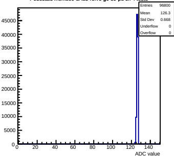
Pedestals mcm160-1A15-relv6-g0-s0-p1 ch 4 test1
