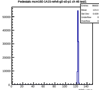
Pedestals mcm160-1A15-refv6-g0-s0-p1 ch 46 test1
