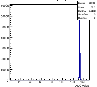
Pedestals mcm160-1A15-relv6-g0-s0-p1 ch 12 test1
