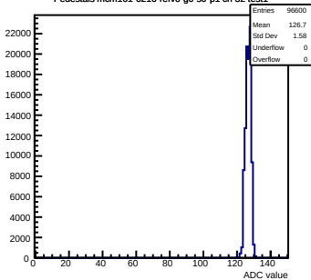
Pedestals mcm161-6216-rev0-g0-s0-p1 ch 32 test1
