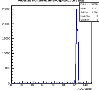
Pedestals mcm161-6216-refV0-g0-s0-p1 ch 6 test1
