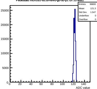
Pedestals mcm161-6216-refV0-g0-s0-p1 ch 13 test1
