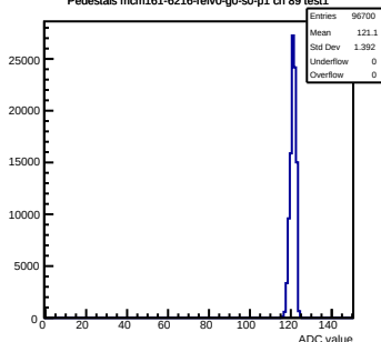
Pedestals mcm161-6216-rev0-g0-s0-p1 ch 89 test1
