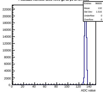
Pedestals mcm161-6216-rev0-g0-s0-p1 ch 34 test1
