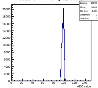
Pedestals mcm161-6216-rv1-q0-s0-p1 ch 55 test1
