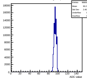
Pedestals mcm161-6216-refv1-g0-s0-p1 ch 14 test1
