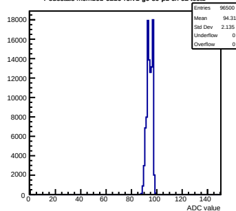
Pedestals mcm161-6216-rv1-q0-s0-p1 ch 62 test1
