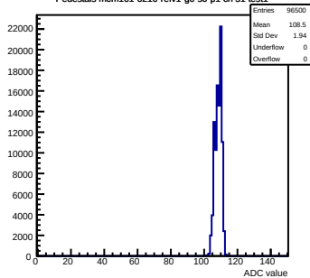
Pedestals mcm161-6216-rv1-q0-s0-p1 ch 51 test1
