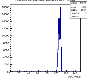
Pedestals mcm161-6216-rv1-q0-s0-p1 ch 48 test1
