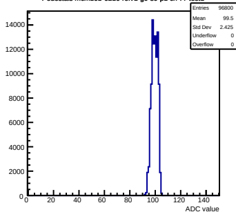
Pedestals mcm161-6216-rv1-q0-s0-p1 ch 77 test1
