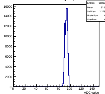
Pedestals mcm161-6216-refv1-g0-s0-p1 ch 6 test1
