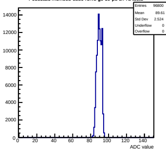
Pedestals mcm161-6216-rv1-q0-s0-p1 ch 72 test1
