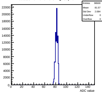
Pedestals mcm161-6216-refv1-g0-s0-p1 ch 124 test1
