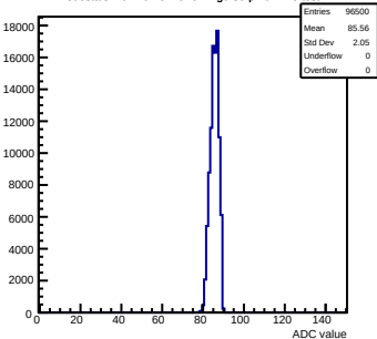
Pedestals mcm161-6216-refv1-g0-s0-p1 ch 125 test1
