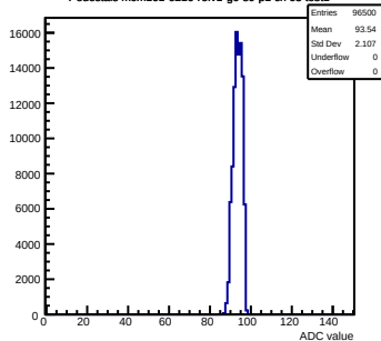
Pedestals mcm161-6216-rv1-q0-s0-p1 ch 63 test1
