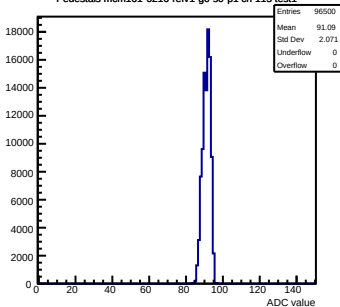
Pedestals mcm161-6216-refv1-g0-s0-p1 ch 115 test1
