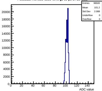
Pedestals mcm161-6216-rv1-q0-s0-p1 ch 53 test1
