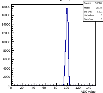
Pedestals mcm161-6216-refv1-g0-s0-p1 ch 127 test1
