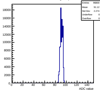
Pedestals mcm161-6216-refv1-g0-s0-p1 ch 13 test1
