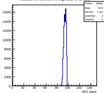
Pedestals mcm161-6216-rv1-q0-s0-p1 ch 59 test1
