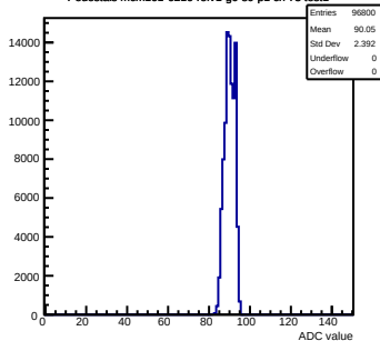
Pedestals mcm161-6216-rv1-q0-s0-p1 ch 73 test1
