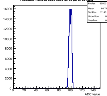
Pedestals mcm161-6216-rv1-q0-s0-p1 ch 50 test1
