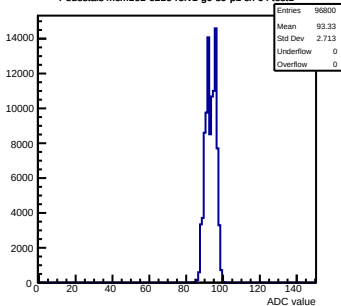
Pedestals mcm161-6216-rv1-q0-s0-p1 ch 64 test1
