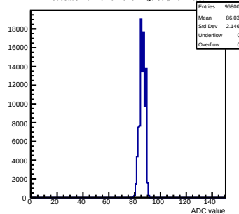
Pedestals mcm161-6216-refv1-g0-s0-p1 ch 2 test1
