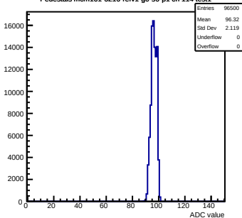
Pedestals mcm161-6216-refv1-g0-s0-p1 ch 114 test1
