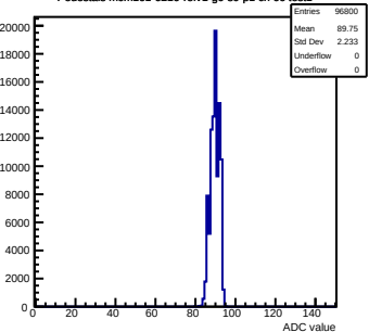
Pedestals mcm161-6216-rv1-q0-s0-p1 ch 66 test1
