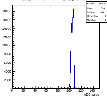
Pedestals mcm161-6216-rv1-q0-s0-p1 ch 60 test1
