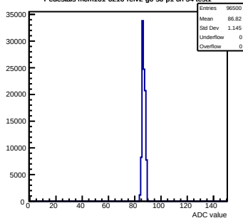
Pedestals mcm161-6216-refv2-g0-s0-p1 ch 54 test1
