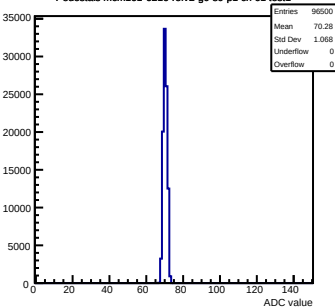
Pedestals mcm161-6216-refv2-g0-s0-p1 ch 61 test1
