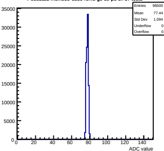
Pedestals mcm161-6216-refv2-g0-s0-p1 ch 57 test1
