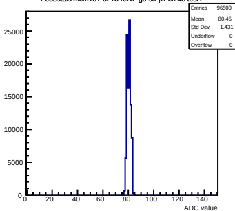
Pedestals mcm161-6216-g0-s0-p1 ch 48 test1
