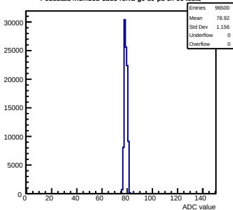
Pedestals mcm161-6216-refv2-g0-s0-p1 ch 60 test1
