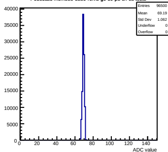
Pedestals mcm161-6216-refv2-g0-s0-p1 ch 62 test1
