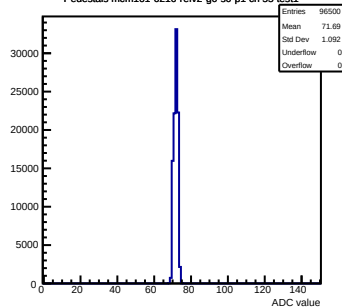
Pedestals mcm161-6216-refv2-g0-s0-p1 ch 55 test1
