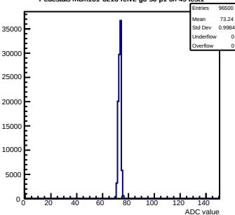
Pedestals mcm161-6216-refv2-g0-s0-p1 ch 49 test1
