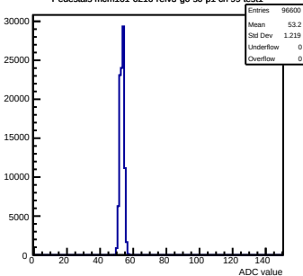
Pedestals mcm161-6216-refv3-g0-s0-p1 ch 99 test1
