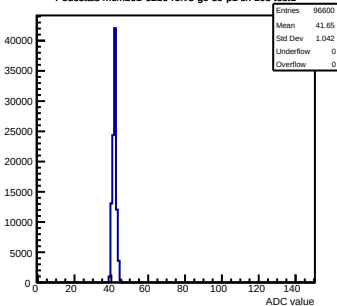
Pedestals mcm161-6216-refv3-g0-s0-p1 ch 103 test1
