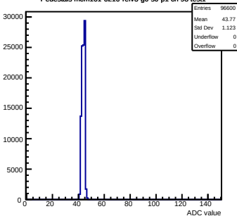
Pedestals mcm161-6216-refv3-g0-s0-p1 ch 98 test1
