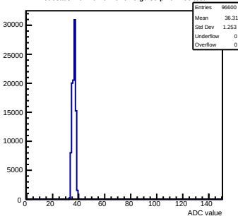
Pedestals mcm161-6216-refv3-g0-s0-p1 ch 106 test1
