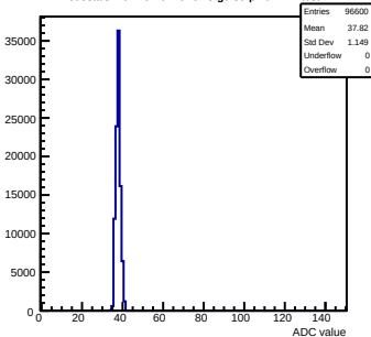
Pedestals mcm161-6216-refv3-g0-s0-p1 ch 111 test1
