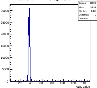
Pedestals mcm161-6216-refv3-g0-s0-p1 ch 101 test1
