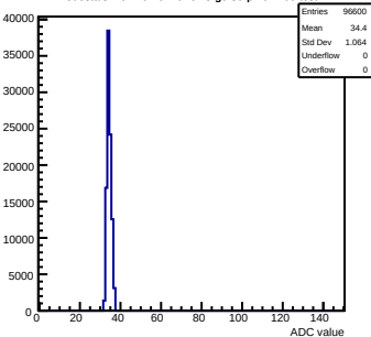
Pedestals mcm161-6216-refv3-g0-s0-p1 ch 109 test1
