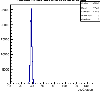
Pedestals mcm161-6216-refv3-g0-s0-p1 ch 96 test1
