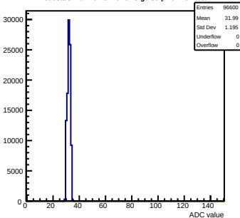
Pedestals mcm161-6216-refv3-g0-s0-p1 ch 107 test1
