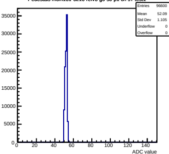
Pedestals mcm161-6216-refv3-g0-s0-p1 ch 97 test1
