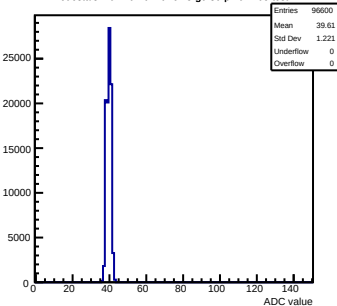
Pedestals mcm161-6216-refv3-g0-s0-p1 ch 105 test1
