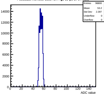
Pedestals mcm161-6216-rlv4-g0-s0-p1 ch 64 test1
