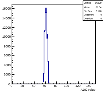
Pedestals mcm161-6216-rlv4-g0-s0-p1 ch 77 test1
