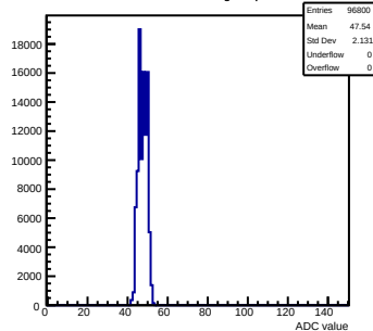
Pedestals mcm161-6216-rlv4-g0-s0-p1 ch 75 test1
