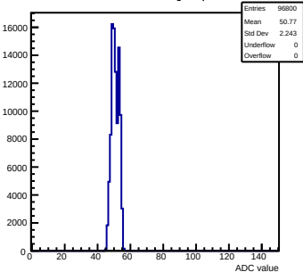
Pedestals mcm161-6216-rlv4-g0-s0-p1 ch 72 test1
