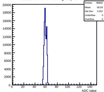
Pedestals mcm161-6216-rlv4-g0-s0-p1 ch 70 test1
