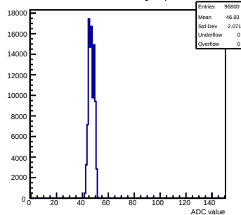
Pedestals mcm161-6216-rlv4-g0-s0-p1 ch 79 test1
