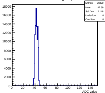
Pedestals mcm161-6216-rlv4-g0-s0-p1 ch 69 test1
