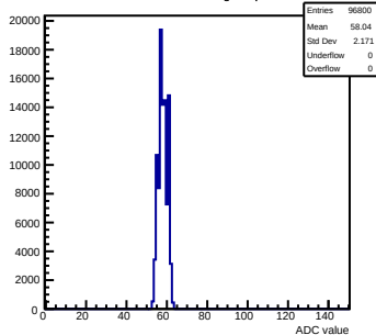
Pedestals mcm161-6216-rlv4-g0-s0-p1 ch 74 test1
