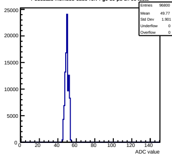
Pedestals mcm161-6216-rlv4-g0-s0-p1 ch 66 test1
