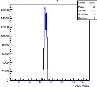
Pedestals mcm161-6216-rlv4-g0-s0-p1 ch 68 test1
