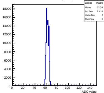
Pedestals mcm161-6216-rlv4-g0-s0-p1 ch 78 test1
