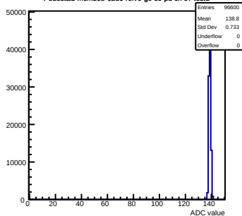
Pedestals mcm161-6216-refV0-g0-s0-p1 ch 97 test1
