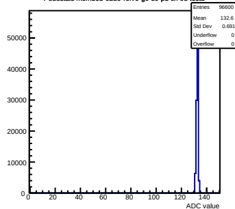
Pedestals mcm161-6216-refV0-g0-s0-p1 ch 98 test1
