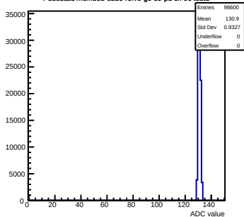
Pedestals mcm161-6216-refV0-g0-s0-p1 ch 96 test1
