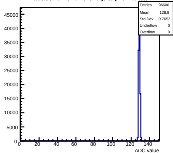
Pedestals mcm161-6216-refV0-g0-s0-p1 ch 100 test1
