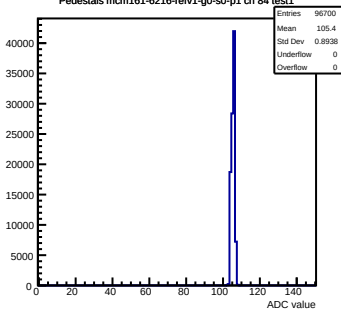
Pedestals mcm161-6216-rlv1-g0-s0-p1 ch 84 test1
