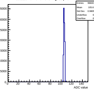
Pedestals mcm161-6216-relv1-g0-s0-p1 ch 41 test1
