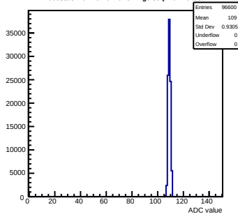
Pedestals mcm161-6216-relv1-g0-s0-p1 ch 46 test1
