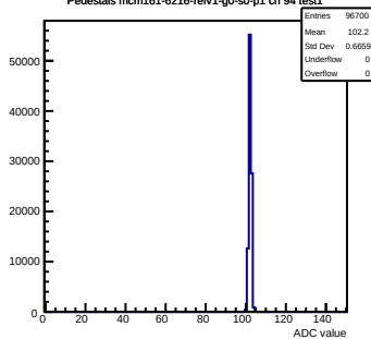
Pedestals mcm161-6216-rlv1-g0-s0-p1 ch 94 test1
