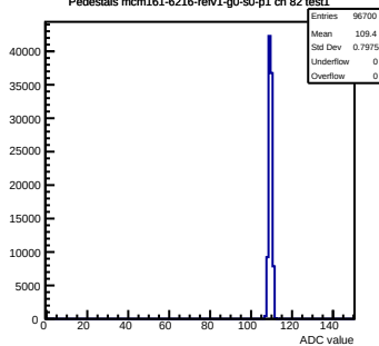
Pedestals mcm161-6216-rlv1-g0-s0-p1 ch 82 test1
