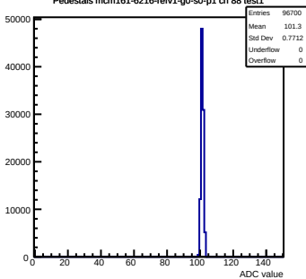
Pedestals mcm161-6216-rlv1-g0-s0-p1 ch 88 test1
