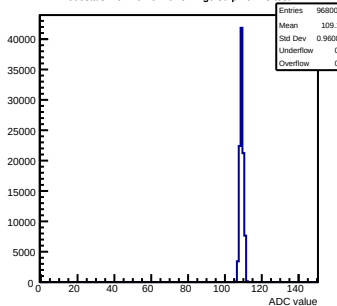
Pedestals mcm161-6216-rlv1-g0-s0-p1 ch 78 test1
