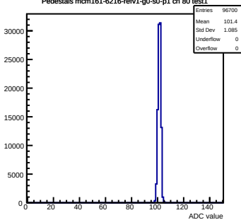
Pedestals mcm161-6216-rlv1-g0-s0-p1 ch 80 test1
