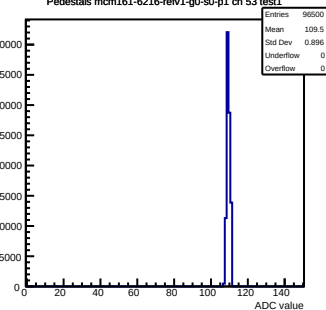
Pedestals mcm161-6216-relv1-g0-s0-p1 ch 53 test1
