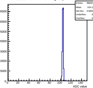
Pedestals mcm161-6216-relv1-g0-s0-p1 ch 45 test1
