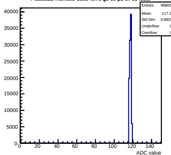
Pedestals mcm161-6216-rlv1-g0-s0-p1 ch 65 test1
