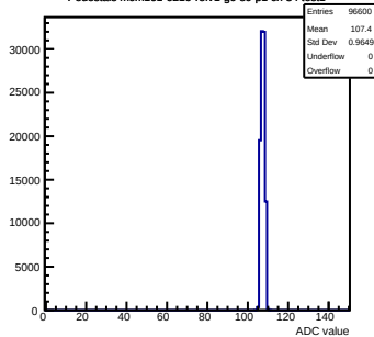
Pedestals mcm161-6216-relv1-g0-s0-p1 ch 34 test1
