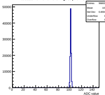
Pedestals mcm161-6216-rlv1-g0-s0-p1 ch 73 test1
