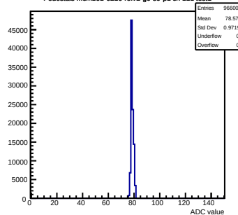
Pedestals mcm161-6216-refv2-g0-s0-p1 ch 111 test1
