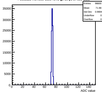
Pedestals mcm161-6216-refv2-g0-s0-p1 ch 109 test1
