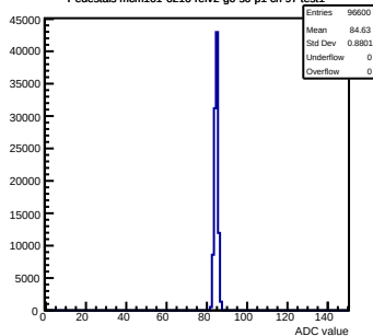
Pedestals mcm161-6216-refv2-g0-s0-p1 ch 97 test1
