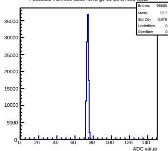
Pedestals mcm161-6216-refv2-g0-s0-p1 ch 105 test1
