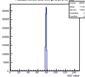
Pedestals mcm161-6216-g0-s0-p1 ch 50 test1
