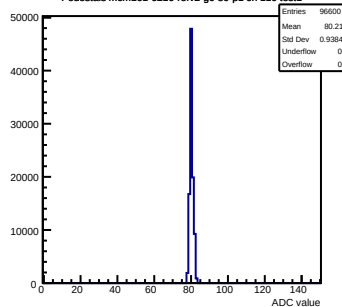
Pedestals mcm161-6216-refv2-g0-s0-p1 ch 110 test1
