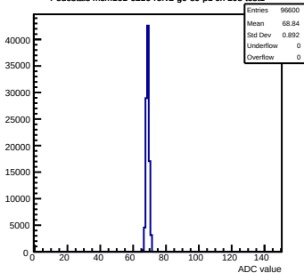
Pedestals mcm161-6216-refv2-g0-s0-p1 ch 108 test1
