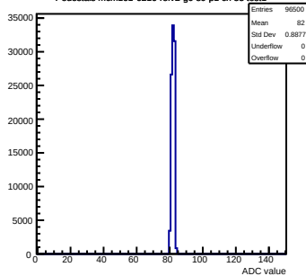
Pedestals mcm161-6216-refv2-g0-s0-p1 ch 53 test1
