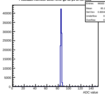
Pedestals mcm161-6216-g0-s0-p1 ch 51 test1
