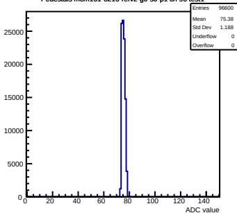
Pedestals mcm161-6216-refv2-g0-s0-p1 ch 96 test1
