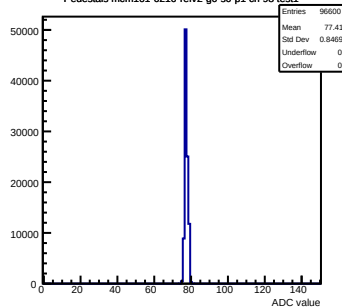
Pedestals mcm161-6216-refv2-g0-s0-p1 ch 98 test1
