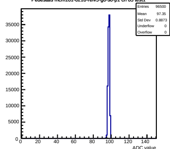
Pedestals mcm161-6216-refV5-g0-s0-p1 ch 63 test1
