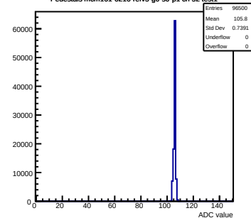
Pedestals mcm161-6216-refV5-g0-s0-p1 ch 52 test1
