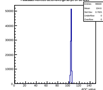
Pedestals mcm161-6216-refV5-g0-s0-p1 ch 60 test1
