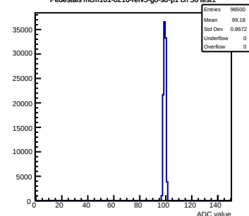
Pedestals mcm161-6216-refV5-g0-s0-p1 ch 56 test1
