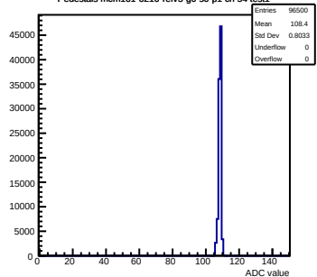
Pedestals mcm161-6216-refV5-g0-s0-p1 ch 54 test1
