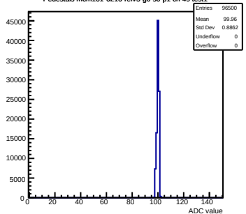
Pedestals mcm161-6216-refV5-g0-s0-p1 ch 49 test1
