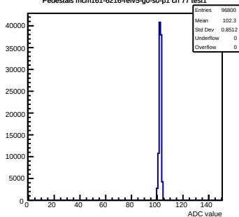
Pedestals mcm161-6216- \text{rev5-g0-s0-p1} ch 77 test1
