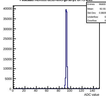
Pedestals mcm161-6216- \text{rev5-g0-s0-p1} ch 75 test1
