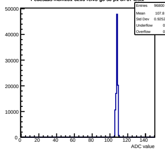
Pedestals mcm161-6216- \text{rev5-g0-s0-p1} ch 67 test1
