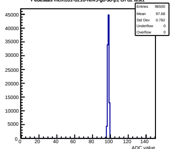
Pedestals mcm161-6216-refV5-g0-s0-p1 ch 62 test1
