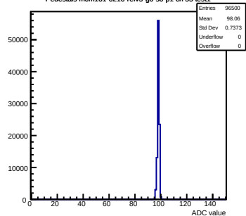
Pedestals mcm161-6216-refV5-g0-s0-p1 ch 55 test1
