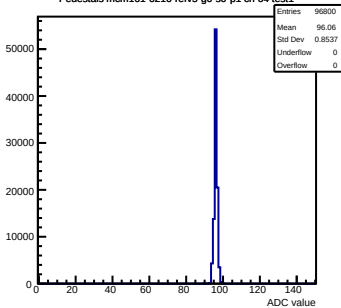
Pedestals mcm161-6216- \text{rev5-g0-s0-p1} ch 64 test1
