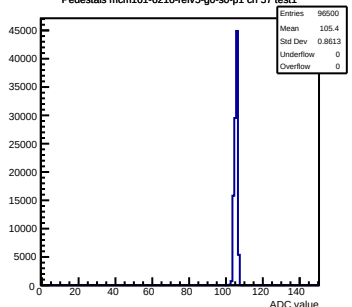
Pedestals mcm161-6216-refV5-g0-s0-p1 ch 57 test1
