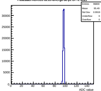
Pedestals mcm161-6216- \text{rev5-g0-s0-p1} ch 72 test1
