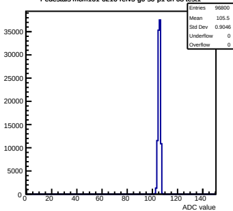
Pedestals mcm161-6216- \text{rev5-g0-s0-p1} ch 68 test1
