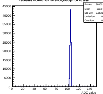
Pedestals mcm161-6216- \text{rev5-g0-s0-p1} ch 78 test1
