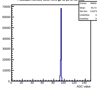
Pedestals mcm161-6216- \text{rev5-g0-s0-p1} ch 66 test1
