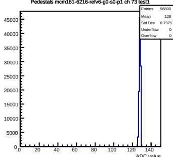
Pedestals mcm161-6216-relv6-g0-s0-p1 ch 73 test1
