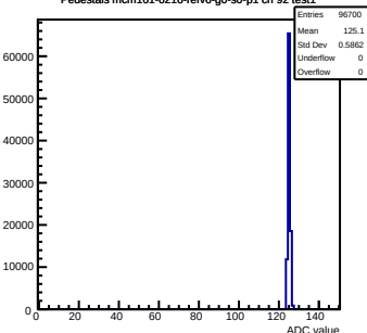
Pedestals mcm161-6216-relv6-g0-s0-p1 ch 92 test1
