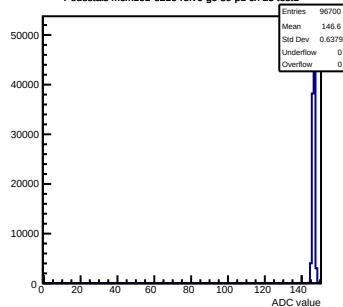
Pedestals mcm161-6216-relv6-g0-s0-p1 ch 25 test1
