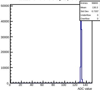
Pedestals mcm161-6216-rtv6-g0-s0-p1 ch 8 test1
