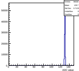
Pedestals mcm161-6216-relv6-g0-s0-p1 ch 55 test1
