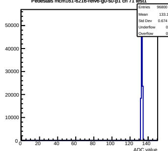
Pedestals mcm161-6216-relv6-g0-s0-p1 ch 71 test1
