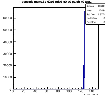
Pedestals mcm161-6216-relv6-g0-s0-p1 ch 79 test1
