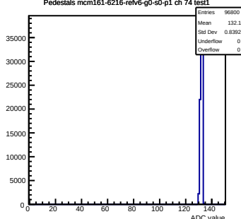
Pedestals mcm161-6216-relv6-g0-s0-p1 ch 74 test1
