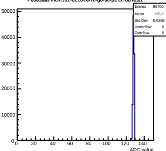
Pedestals mcm161-6216-relv6-g0-s0-p1 ch 88 test1
