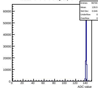
Pedestals mcm161-6216-relv6-g0-s0-p1 ch 29 test1
