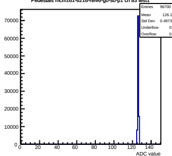
Pedestals mcm161-6216-relv6-g0-s0-p1 ch 83 test1
