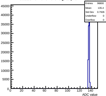
Pedestals mcm161-6216-rtv6-g0-s0-p1 ch 12 test1
