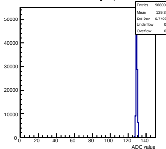
Pedestals mcm161-6216-rtv6-g0-s0-p1 ch 14 test1
