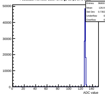
Pedestals mcm161-6216-rtv6-g0-s0-p1 ch 6 test1
