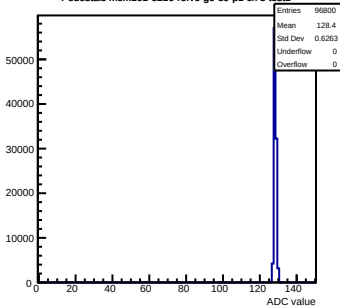
Pedestals mcm161-6216-rtv6-g0-s0-p1 ch 5 test1
