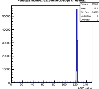
Pedestals mcm161-6216-relv6-g0-s0-p1 ch 69 test1
