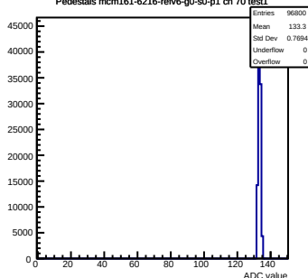
Pedestals mcm161-6216-relv6-g0-s0-p1 ch 70 test1
