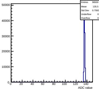
Pedestals mcm161-6216-relv6-g0-s0-p1 ch 53 test1
