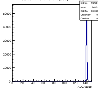
Pedestals mcm161-6216-relv6-g0-s0-p1 ch 21 test1
