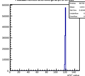
Pedestals mcm161-6216-relv6-g0-s0-p1 ch 91 test1
