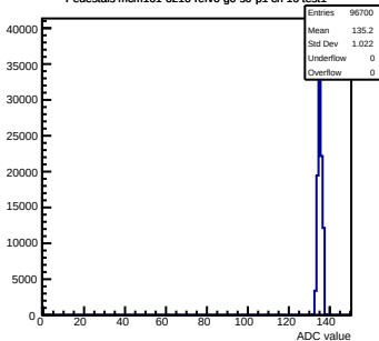
Pedestals mcm161-6216-relv6-g0-s0-p1 ch 16 test1
