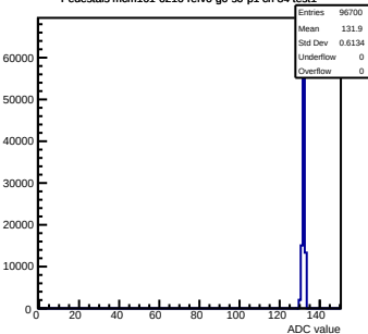
Pedestals mcm161-6216-relv6-g0-s0-p1 ch 84 test1
