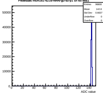
Pedestals mcm161-6216-relv6-g0-s0-p1 ch 65 test1
