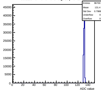
Pedestals mcm161-6216-relv6-g0-s0-p1 ch 30 test1
