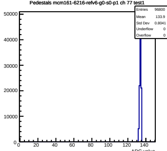
Pedestals mcm161-6216-relv6-g0-s0-p1 ch 77 test1
