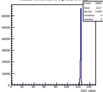
Pedestals mcm161-6216-rtv6-g0-s0-p1 ch 1 test1
