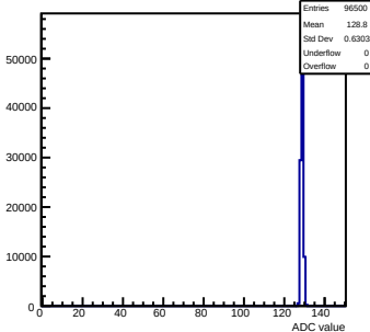
Pedestals mcm161-6216-relv6-g0-s0-p1 ch 59 test1
