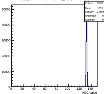
Pedestals mcm161-6216-relv6-g0-s0-p1 ch 50 test1
