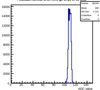
Pedestals mcm162-3A14-refv1-g0-s0-p1 ch 16 test1
