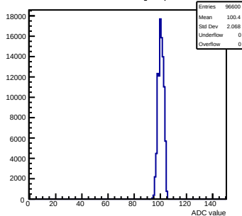
Pedestals mcm162-3A14-refv1-g0-s0-p1 ch 110 test1
