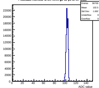
Pedestals mcm162-3A14-refv1-g0-s0-p1 ch 87 test1
