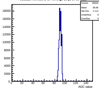
Pedestals mcm162-3A14-refv1-g0-s0-p1 ch 99 test1
