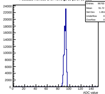
Pedestals mcm162-3A14-refv1-g0-s0-p1 ch 91 test1
