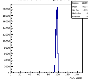
Pedestals mcm162-3A14-refv1-g0-s0-p1 ch 30 test1
