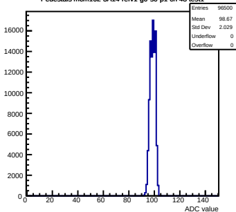
Pedestals mcm162-3A14-refv1-g0-s0-p1 ch 48 test1
