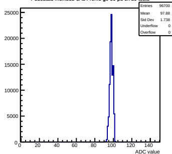
Pedestals mcm162-3A14-refv1-g0-s0-p1 ch 29 test1
