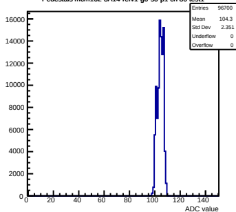
Pedestals mcm162-3A14-refv1-g0-s0-p1 ch 80 test1
