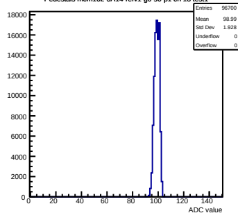
Pedestals mcm162-3A14-refv1-g0-s0-p1 ch 18 test1
