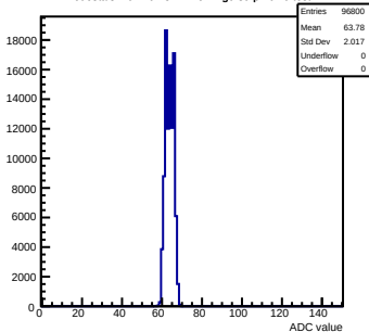
Pedestals mcm162-3A14-refV4-g0-s0-p1 ch 9 test1
