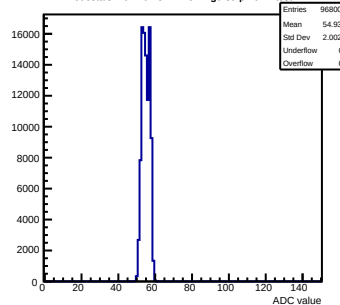
Pedestals mcm162-3A14-refV4-g0-s0-p1 ch 7 test1
