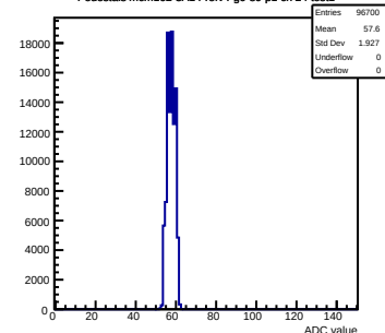
Pedestals mcm162-3A14-refv4-g0-s0-p1 ch 24 test1
