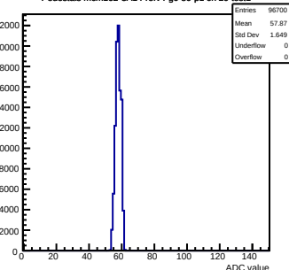
Pedestals mcm162-3A14-refv4-g0-s0-p1 ch 29 test1
