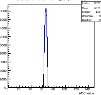
Pedestals mcm162-3A14-refv4-g0-s0-p1 ch 17 test1
