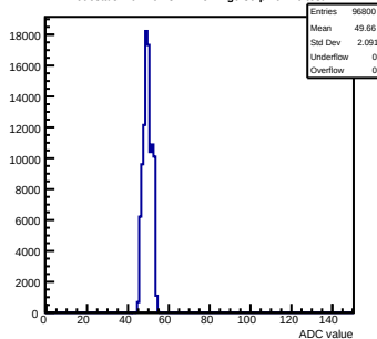
Pedestals mcm162-3A14-refV4-g0-s0-p1 ch 10 test1
