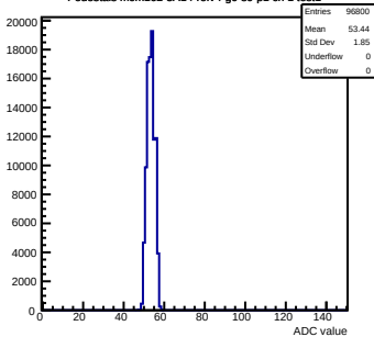
Pedestals mcm162-3A14-refV4-g0-s0-p1 ch 1 test1
