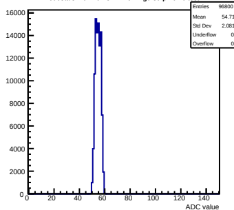
Pedestals mcm162-3A14-refV4-g0-s0-p1 ch 6 test1
