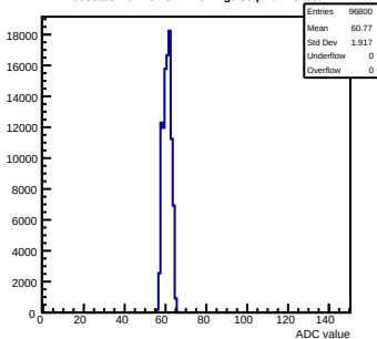
Pedestals mcm162-3A14-refV4-g0-s0-p1 ch 13 test1
