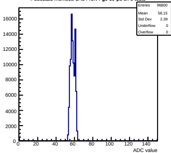
Pedestals mcm162-3A14-refV4-g0-s0-p1 ch 0 test1
