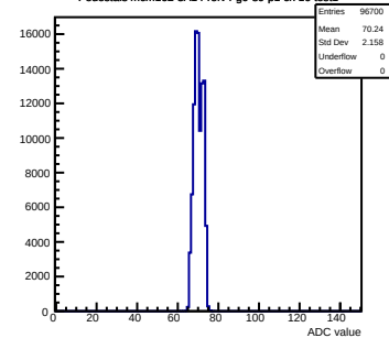
Pedestals mcm162-3A14-refv4-g0-s0-p1 ch 16 test1
