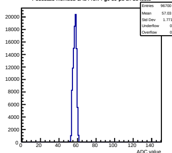
Pedestals mcm162-3A14-refv4-g0-s0-p1 ch 31 test1
