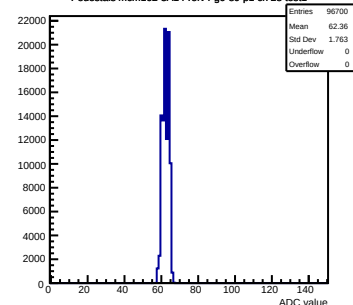
Pedestals mcm162-3A14-refv4-g0-s0-p1 ch 28 test1
