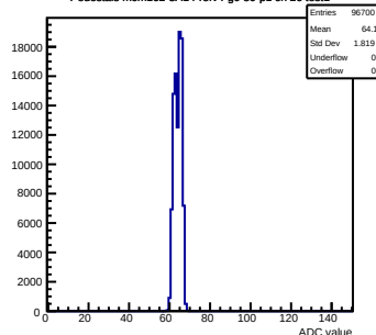
Pedestals mcm162-3A14-refv4-g0-s0-p1 ch 26 test1
