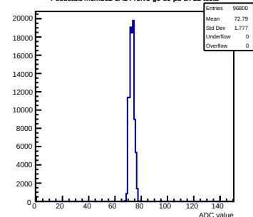
Pedestals mcm162-3A14-relv5-g0-s0-p1 ch 12 test1
