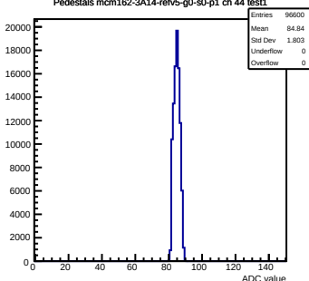
Pedestals mcm162-3A14-rfv5-g0-s0-p1 ch 44 test1
