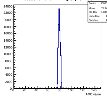
Pedestals mcm162-3A14-relv5-g0-s0-p1 ch 2 test1
