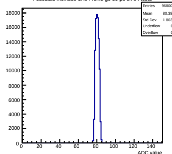
Pedestals mcm162-3A14-relv5-g0-s0-p1 ch 14 test1
