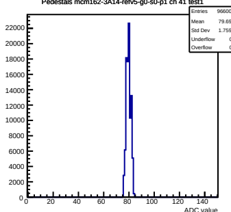
Pedestals mcm162-3A14-rfv5-g0-s0-p1 ch 41 test1
