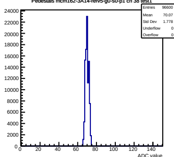
Pedestals mcm162-3A14-rfv5-g0-s0-p1 ch 38 test1
