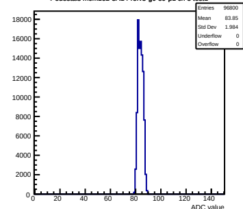
Pedestals mcm162-3A14-relv5-g0-s0-p1 ch 8 test1
