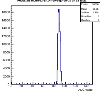
Pedestals mcm162-3A14-rfv5-g0-s0-p1 ch 32 test1
