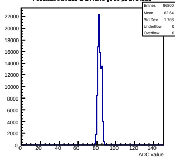
Pedestals mcm162-3A14-relv5-g0-s0-p1 ch 5 test1
