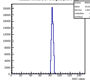
Pedestals mcm162-3A14-relv5-g0-s0-p1 ch 6 test1
