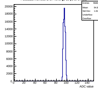
Pedestals mcm162-3A14-relv5-g0-s0-p1 ch 3 test1
