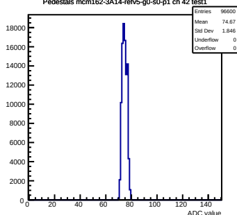
Pedestals mcm162-3A14-rfv5-g0-s0-p1 ch 42 test1
