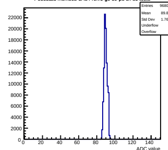
Pedestals mcm162-3A14-relv5-g0-s0-p1 ch 15 test1
