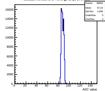
Pedestals mcm162-3A14-relv5-g0-s0-p1 ch 0 test1
