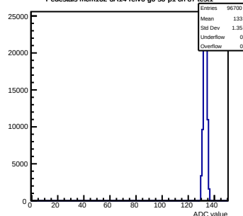
Pedestals mcm162-3A14-refv6-g0-s0-p1 ch 87 test1
