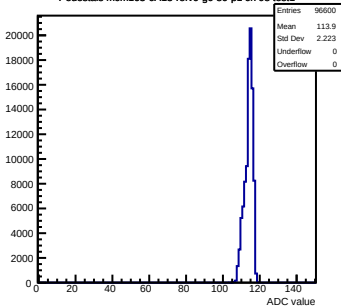
Pedestals mcm163-6A13-refV0-g0-s0-p1 ch 98 test1
