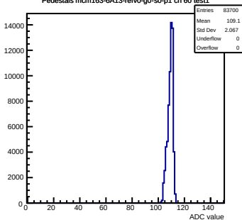
Pedestals mcm163-6A13-refV0-g0-s0-p1 ch 60 test1
