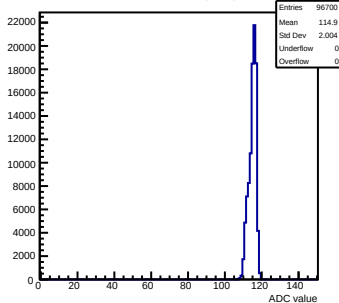
Pedestals mcm163-6A13-rev0-g0-s0-p1 ch 87 test1
