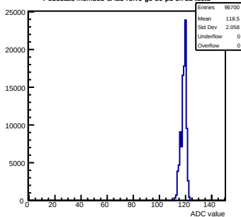
Pedestals mcm163-6A13-rev0-g0-s0-p1 ch 82 test1
