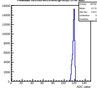
Pedestals mcm163-6A13-refV0-g0-s0-p1 ch 62 test1
