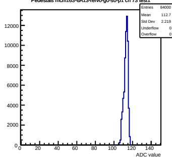
Pedestals mcm163-6A13-refV0-g0-s0-p1 ch 73 test1
