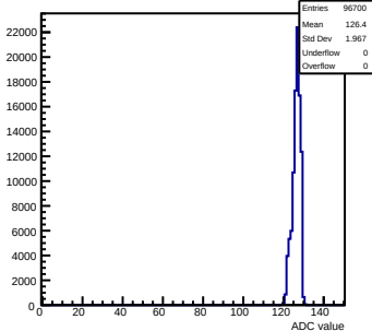
Pedestals mcm163-6A13-rev0-g0-s0-p1 ch 88 test1
