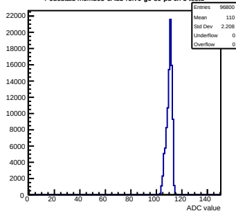
Pedestals mcm163-6A13-refV0-g0-s0-p1 ch 5 test1
