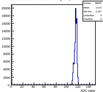
Pedestals mcm163-6A13-refV0-g0-s0-p1 ch 102 test1
