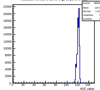
Pedestals mcm163-6A13-refV0-g0-s0-p1 ch 2 test1
