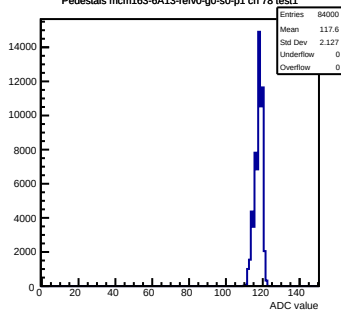
Pedestals mcm163-6A13-refV0-g0-s0-p1 ch 78 test1
