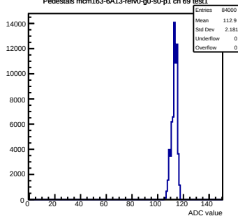
Pedestals mcm163-6A13-refV0-g0-s0-p1 ch 69 test1
