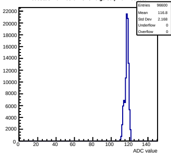
Pedestals mcm163-6A13-refV0-g0-s0-p1 ch 108 test1
