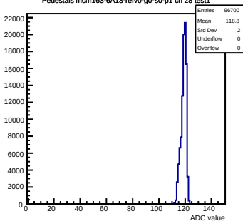
Pedestals mcm163-6A13-refV0-g0-s0-p1 ch 28 test1
