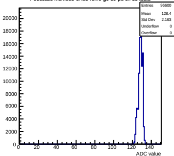
Pedestals mcm163-6A13-refV0-g0-s0-p1 ch 35 test1
