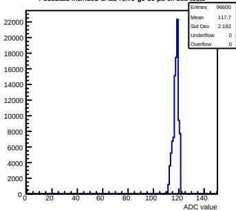
Pedestals mcm163-6A13-refV0-g0-s0-p1 ch 101 test1
