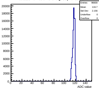
Pedestals mcm163-6A13-refV0-g0-s0-p1 ch 38 test1
