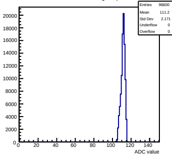
Pedestals mcm163-6A13-refV0-g0-s0-p1 ch 45 test1
