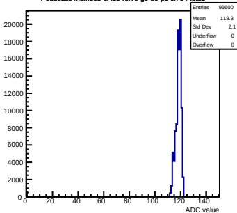
Pedestals mcm163-6A13-refV0-g0-s0-p1 ch 34 test1
