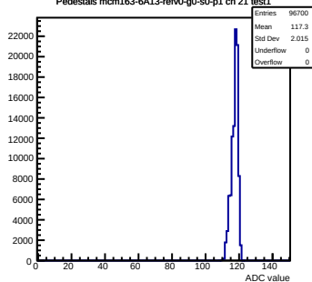
Pedestals mcm163-6A13-refV0-g0-s0-p1 ch 21 test1
