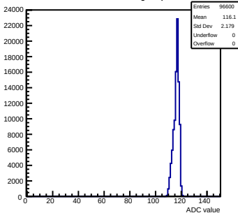
Pedestals mcm163-6A13-refV0-g0-s0-p1 ch 43 test1
