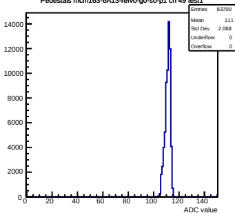
Pedestals mcm163-6A13-refV0-g0-s0-p1 ch 49 test1
