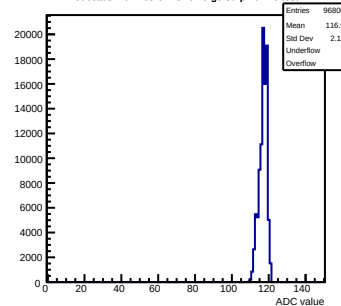
Pedestals mcm163-6A13-refV0-g0-s0-p1 ch 15 test1
