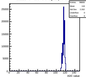
Pedestals mcm163-6A13-refV0-g0-s0-p1 ch 37 test1
