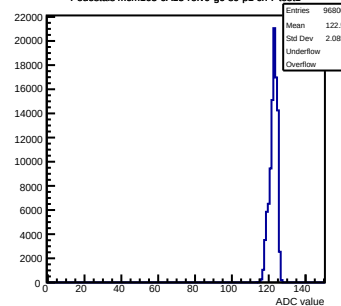
Pedestals mcm163-6A13-refV0-g0-s0-p1 ch 7 test1
