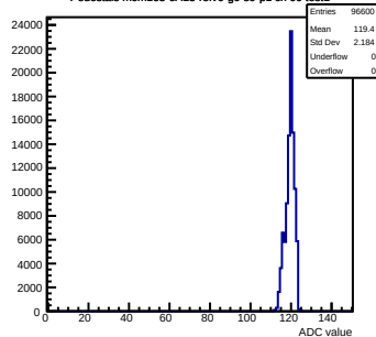
Pedestals mcm163-6A13-refV0-g0-s0-p1 ch 99 test1
