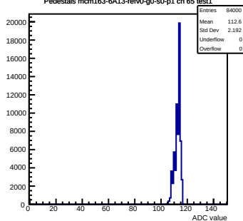
Pedestals mcm163-6A13-refV0-g0-s0-p1 ch 65 test1
