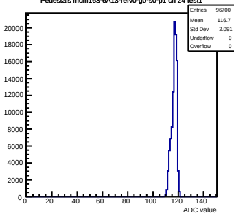
Pedestals mcm163-6A13-refV0-g0-s0-p1 ch 24 test1
