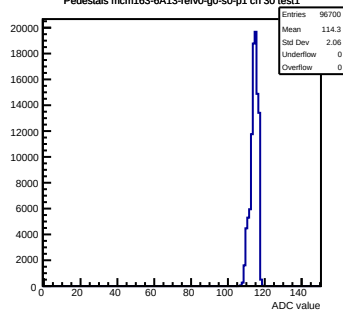
Pedestals mcm163-6A13-refV0-g0-s0-p1 ch 30 test1
