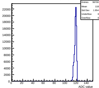
Pedestals mcm163-6A13-rev0-g0-s0-p1 ch 85 test1
