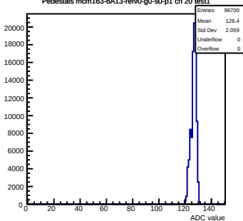
Pedestals mcm163-6A13-refV0-g0-s0-p1 ch 20 test1
