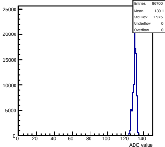
Pedestals mcm163-6A13-rev0-g0-s0-p1 ch 84 test1
