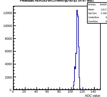
Pedestals mcm163-6A13-refV0-g0-s0-p1 ch 67 test1
