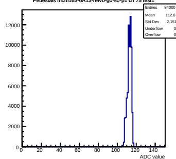
Pedestals mcm163-6A13-refV0-g0-s0-p1 ch 75 test1
