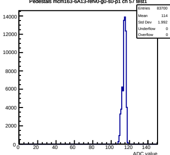
Pedestals mcm163-6A13-refV0-g0-s0-p1 ch 57 test1
