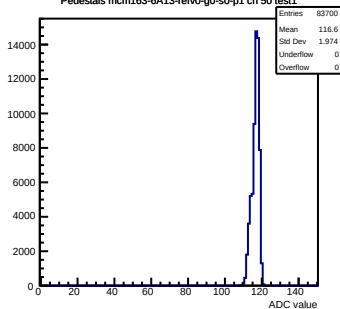
Pedestals mcm163-6A13-refV0-g0-s0-p1 ch 50 test1
