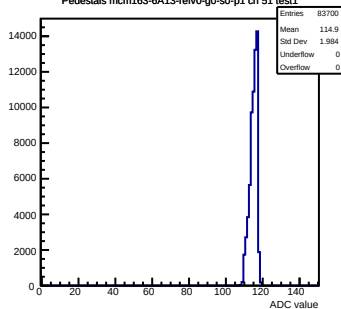
Pedestals mcm163-6A13-refV0-g0-s0-p1 ch 51 test1
