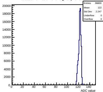
Pedestals mcm163-6A13-refV0-g0-s0-p1 ch 8 test1
