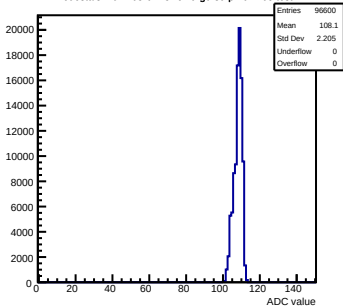
Pedestals mcm163-6A13-refV0-g0-s0-p1 ch 105 test1
