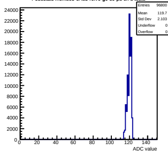
Pedestals mcm163-6A13-refV0-g0-s0-p1 ch 1 test1
