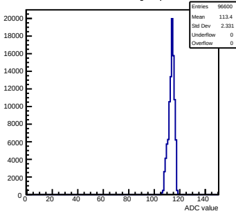
Pedestals mcm163-6A13-refV0-g0-s0-p1 ch 42 test1
