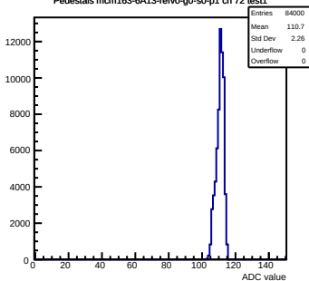
Pedestals mcm163-6A13-refV0-g0-s0-p1 ch 72 test1
