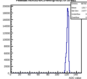
Pedestals mcm163-6A13-refV0-g0-s0-p1 ch 18 test1
