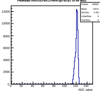
Pedestals mcm163-6A13-refV0-g0-s0-p1 ch 64 test1
