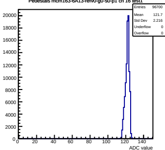
Pedestals mcm163-6A13-refV0-g0-s0-p1 ch 16 test1
