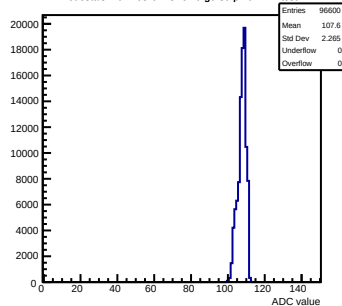
Pedestals mcm163-6A13-refV0-g0-s0-p1 ch 111 test1
