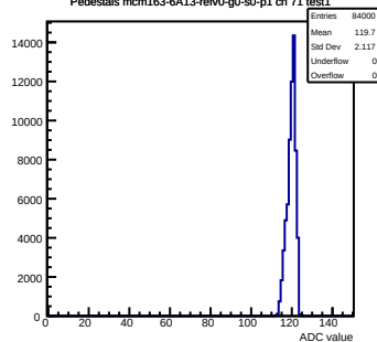
Pedestals mcm163-6A13-refV0-g0-s0-p1 ch 71 test1
