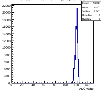
Pedestals mcm163-6A13-refV0-g0-s0-p1 ch 4 test1
