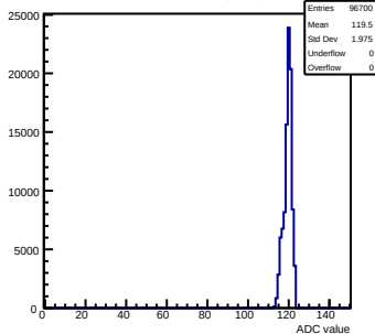
Pedestals mcm163-6A13-rev0-g0-s0-p1 ch 86 test1
