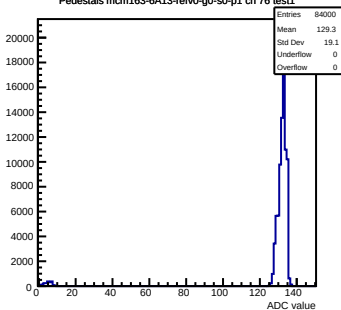
Pedestals mcm163-6A13-refV0-g0-s0-p1 ch 76 test1
