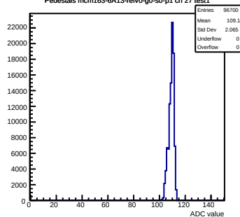
Pedestals mcm163-6A13-refV0-g0-s0-p1 ch 27 test1
