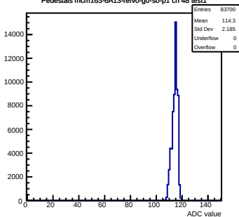
Pedestals mcm163-6A13-refV0-g0-s0-p1 ch 48 test1
