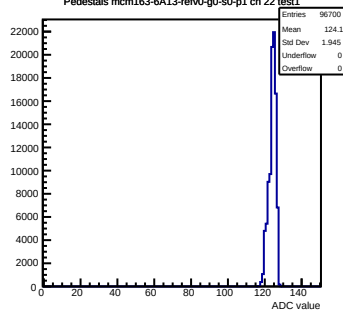
Pedestals mcm163-6A13-refV0-g0-s0-p1 ch 22 test1
