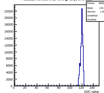
Pedestals mcm163-6A13-refV0-g0-s0-p1 ch 3 test1
