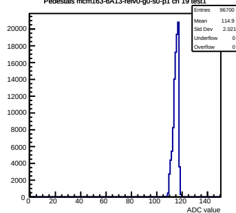
Pedestals mcm163-6A13-refV0-g0-s0-p1 ch 19 test1
