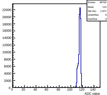
Pedestals mcm163-6A13-rev0-g0-s0-p1 ch 94 test1
