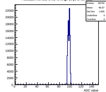
Pedestals mcm163-6A13-refv1-g0-s0-p1 ch 20 test1
