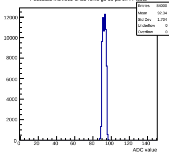
Pedestals mcm163-6A13-refv1-g0-s0-p1 ch 77 test1
