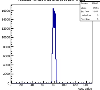
Pedestals mcm163-6A13-refv1-g0-s0-p1 ch 0 test1
