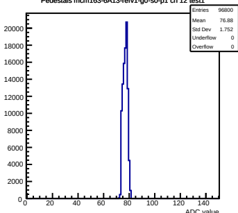
Pedestals mcm163-6A13-refv1-g0-s0-p1 ch 12 test1
