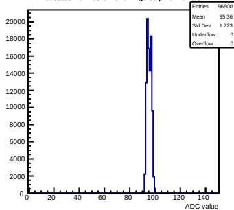
Pedestals mcm163-6A13-refv1-g0-s0-p1 ch 102 test1
