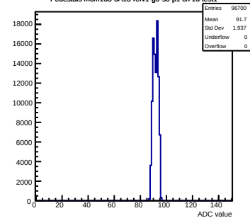
Pedestals mcm163-6A13-refv1-g0-s0-p1 ch 16 test1
