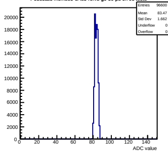
Pedestals mcm163-6A13-refv1-g0-s0-p1 ch 98 test1
