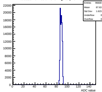
Pedestals mcm163-6A13-refv1-g0-s0-p1 ch 103 test1
