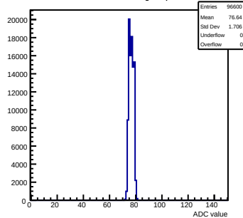
Pedestals mcm163-6A13-refv1-g0-s0-p1 ch 111 test1
