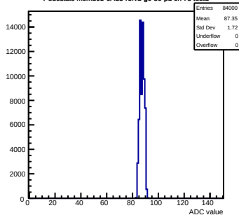
Pedestals mcm163-6A13-refv1-g0-s0-p1 ch 78 test1
