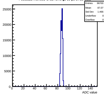
Pedestals mcm163-6A13-refv1-g0-s0-p1 ch 21 test1
