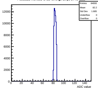
Pedestals mcm163-6A13-refv1-g0-s0-p1 ch 73 test1
