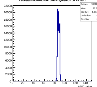
Pedestals mcm163-6A13-refv1-g0-s0-p1 ch 15 test1
