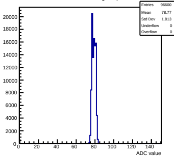
Pedestals mcm163-6A13-refv1-g0-s0-p1 ch 104 test1
