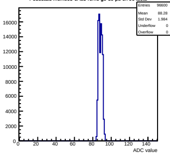
Pedestals mcm163-6A13-refv1-g0-s0-p1 ch 96 test1
