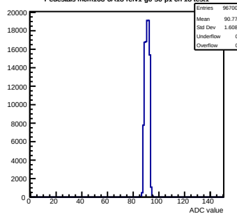
Pedestals mcm163-6A13-refv1-g0-s0-p1 ch 18 test1
