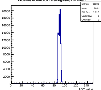
Pedestals mcm163-6A13-refv1-g0-s0-p1 ch 4 test1
