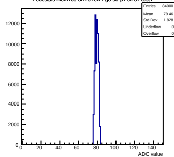
Pedestals mcm163-6A13-refv1-g0-s0-p1 ch 67 test1
