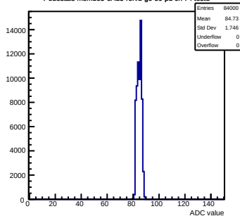
Pedestals mcm163-6A13-refv1-g0-s0-p1 ch 74 test1
