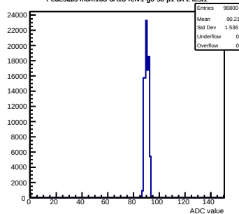
Pedestals mcm163-6A13-refv1-g0-s0-p1 ch 2 test1
