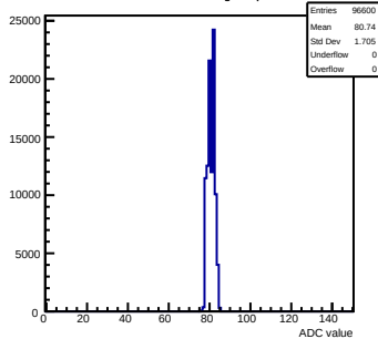
Pedestals mcm163-6A13-refv1-g0-s0-p1 ch 110 test1
