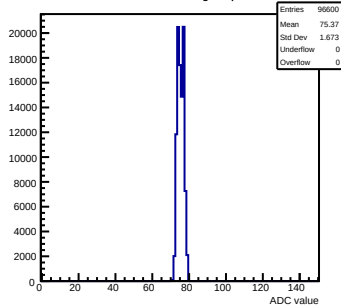
Pedestals mcm163-6A13-refv1-g0-s0-p1 ch 109 test1
