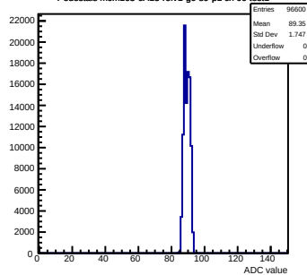
Pedestals mcm163-6A13-refv1-g0-s0-p1 ch 99 test1
