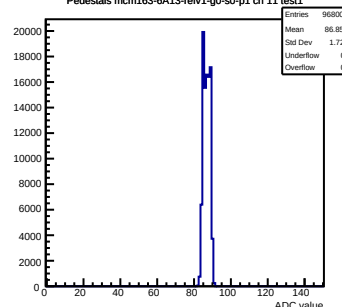
Pedestals mcm163-6A13-refv1-g0-s0-p1 ch 11 test1
