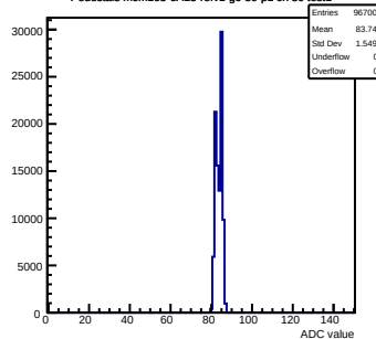
Pedestals mcm163-6A13-refv1-g0-s0-p1 ch 30 test1
