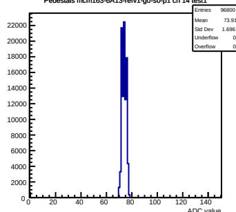
Pedestals mcm163-6A13-refv1-g0-s0-p1 ch 14 test1
