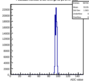
Pedestals mcm163-6A13-refv1-g0-s0-p1 ch 17 test1
