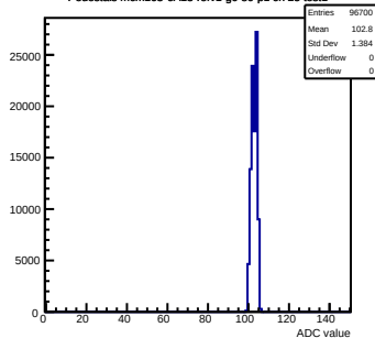
Pedestals mcm163-6A13-refv1-g0-s0-p1 ch 25 test1
