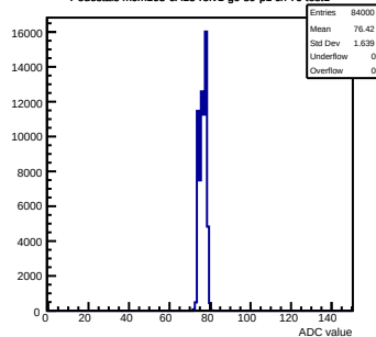
Pedestals mcm163-6A13-refv1-g0-s0-p1 ch 79 test1
