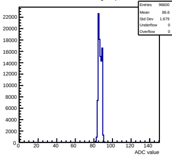
Pedestals mcm163-6A13-refv1-g0-s0-p1 ch 108 test1
