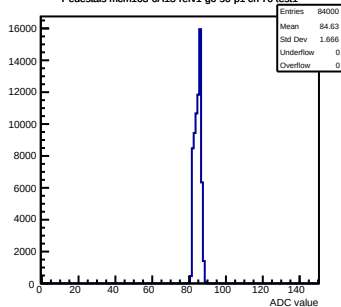
Pedestals mcm163-6A13-refv1-g0-s0-p1 ch 70 test1
