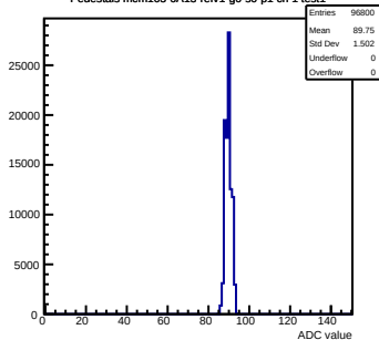
Pedestals mcm163-6A13-refv1-g0-s0-p1 ch 1 test1
