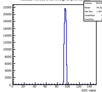
Pedestals mcm163-6A13-refv1-g0-s0-p1 ch 22 test1
