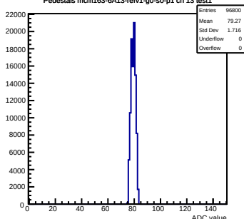
Pedestals mcm163-6A13-refv1-g0-s0-p1 ch 13 test1
