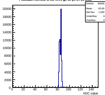
Pedestals mcm163-6A13-refv1-g0-s0-p1 ch 66 test1
