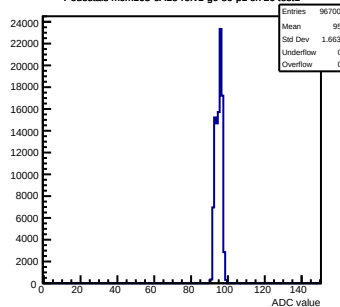
Pedestals mcm163-6A13-refv1-g0-s0-p1 ch 26 test1
