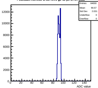
Pedestals mcm163-6A13-refv1-g0-s0-p1 ch 64 test1
