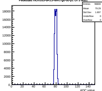
Pedestals mcm163-6A13-refv1-g0-s0-p1 ch 5 test1
