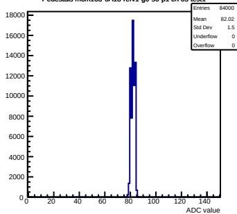
Pedestals mcm163-6A13-refv1-g0-s0-p1 ch 65 test1
