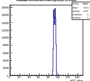
Pedestals mcm163-6A13-refv1-g0-s0-p1 ch 8 test1
