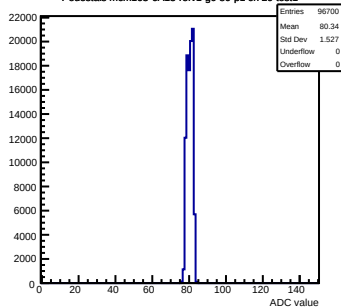
Pedestals mcm163-6A13-refv1-g0-s0-p1 ch 29 test1
