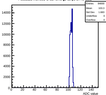
Pedestals mcm163-6A13-refv1-g0-s0-p1 ch 76 test1
