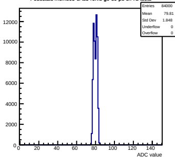
Pedestals mcm163-6A13-refv1-g0-s0-p1 ch 72 test1
