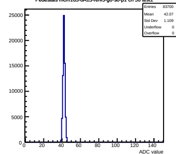
Pedestals mcm163-6A13-refv3-g0-s0-p1 ch 56 test1
