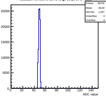
Pedestals mcm163-6A13-refV3-g0-s0-p1 ch 84 test1
