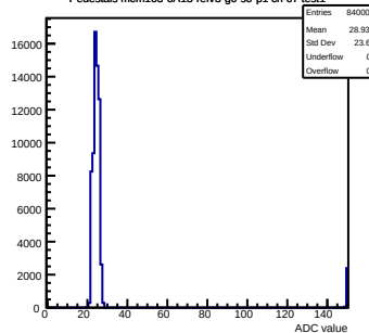
Pedestals mcm163-6A13-refv3-g0-s0-p1 ch 67 test1
