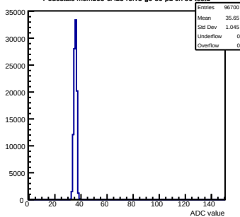
Pedestals mcm163-6A13-refV3-g0-s0-p1 ch 86 test1
