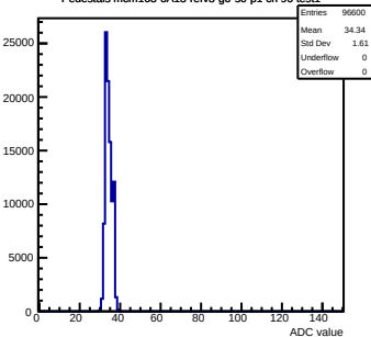
Pedestals mcm163-6A13-refv3-g0-s0-p1 ch 96 test1
