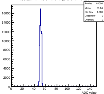
Pedestals mcm163-6A13-refv3-g0-s0-p1 ch 76 test1
