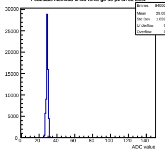
Pedestals mcm163-6A13-refv3-g0-s0-p1 ch 66 test1
