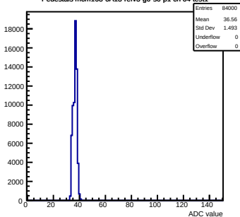
Pedestals mcm163-6A13-refv3-g0-s0-p1 ch 64 test1
