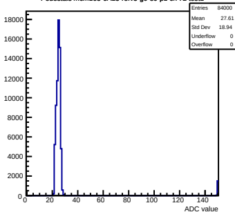
Pedestals mcm163-6A13-refv3-g0-s0-p1 ch 72 test1
