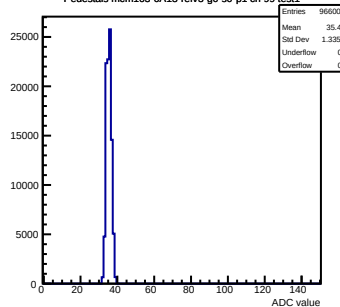
Pedestals mcm163-6A13-refv3-g0-s0-p1 ch 99 test1
