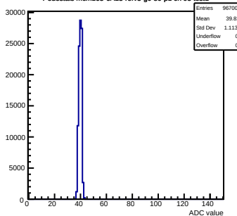
Pedestals mcm163-6A13-refV3-g0-s0-p1 ch 93 test1
