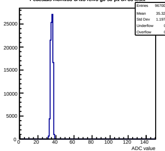
Pedestals mcm163-6A13-refV3-g0-s0-p1 ch 83 test1
