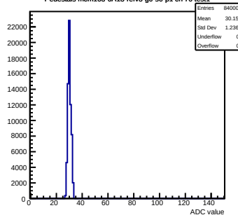
Pedestals mcm163-6A13-refv3-g0-s0-p1 ch 70 test1
