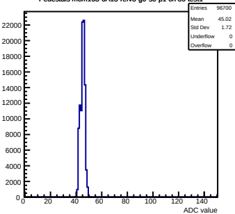
Pedestals mcm163-6A13-refV3-g0-s0-p1 ch 80 test1
