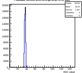
Pedestals mcm163-6A13-refv3-g0-s0-p1 ch 61 test1
