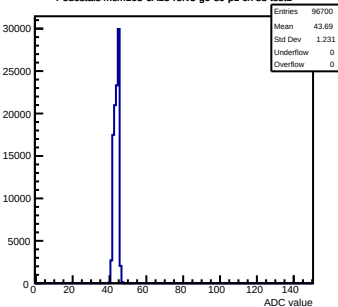
Pedestals mcm163-6A13-refV3-g0-s0-p1 ch 88 test1
