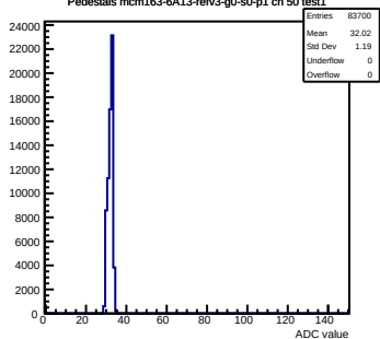
Pedestals mcm163-6A13-refv3-g0-s0-p1 ch 50 test1
