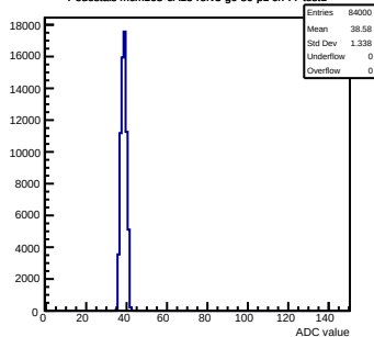
Pedestals mcm163-6A13-refv3-g0-s0-p1 ch 77 test1
