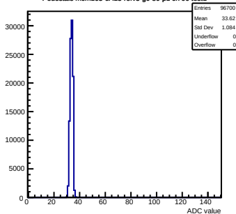
Pedestals mcm163-6A13-refV3-g0-s0-p1 ch 90 test1
