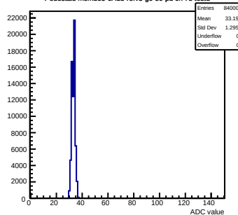
Pedestals mcm163-6A13-refv3-g0-s0-p1 ch 78 test1
