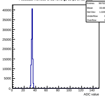
Pedestals mcm163-6A13-refV3-g0-s0-p1 ch 85 test1
