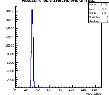
Pedestals mcm163-6A13-refv3-g0-s0-p1 ch 48 test1
