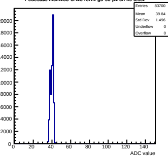
Pedestals mcm163-6A13-refv4-g0-s0-p1 ch 49 test1
