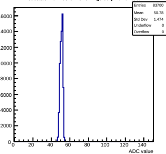
Pedestals mcm163-6A13-refv4-g0-s0-p1 ch 61 test1
