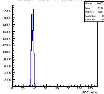
Pedestals mcm163-6A13-refv4-g0-s0-p1 ch 107 test1
