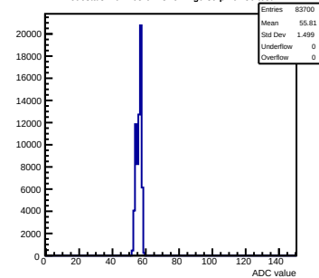
Pedestals mcm163-6A13-refv4-g0-s0-p1 ch 56 test1
