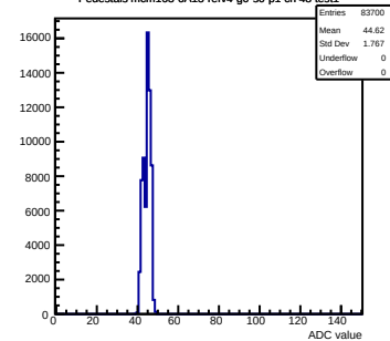
Pedestals mcm163-6A13-refv4-g0-s0-p1 ch 48 test1
