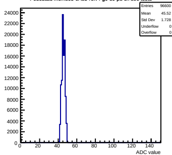
Pedestals mcm163-6A13-refv4-g0-s0-p1 ch 106 test1
