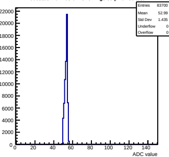
Pedestals mcm163-6A13-refv4-g0-s0-p1 ch 59 test1
