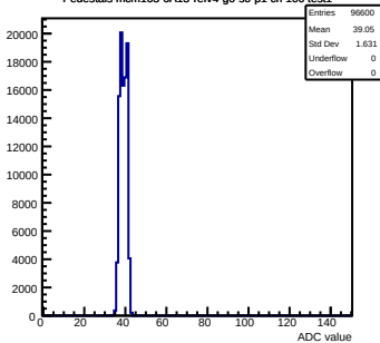
Pedestals mcm163-6A13-refv4-g0-s0-p1 ch 100 test1
