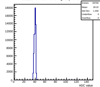
Pedestals mcm163-6A13-refv4-g0-s0-p1 ch 60 test1
