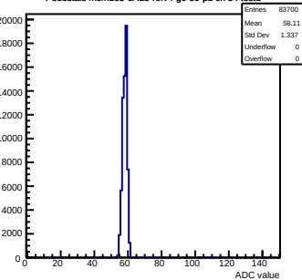
Pedestals mcm163-6A13-refv4-g0-s0-p1 ch 54 test1
