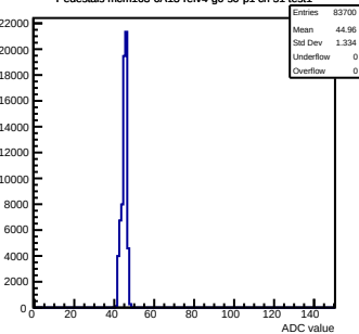
Pedestals mcm163-6A13-refv4-g0-s0-p1 ch 51 test1
