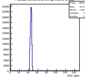
Pedestals mcm163-6A13-refv4-g0-s0-p1 ch 98 test1
