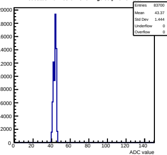
Pedestals mcm163-6A13-refv4-g0-s0-p1 ch 57 test1
