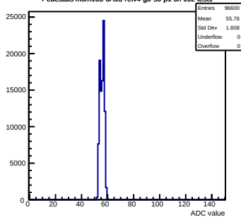
Pedestals mcm163-6A13-refv4-g0-s0-p1 ch 102 test1
