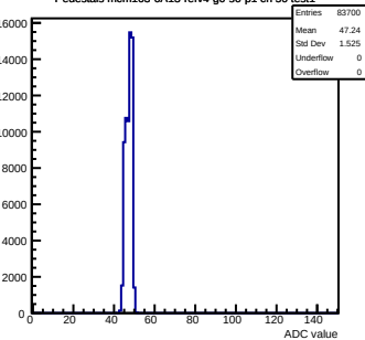
Pedestals mcm163-6A13-refv4-g0-s0-p1 ch 50 test1
