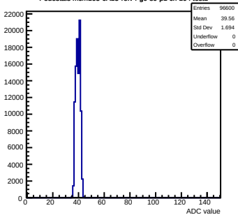
Pedestals mcm163-6A13-refv4-g0-s0-p1 ch 104 test1
