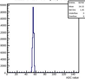
Pedestals mcm163-6A13-refv4-g0-s0-p1 ch 58 test1
