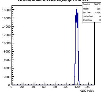
Pedestals mcm163-6A13-relv6-g0-s0-p1 ch 10 test1
