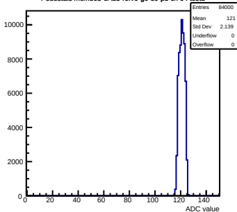
Pedestals mcm163-6A13-refv6-g0-s0-p1 ch 64 test1
