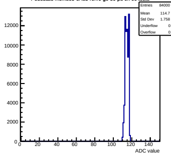
Pedestals mcm163-6A13-refv6-g0-s0-p1 ch 66 test1
