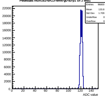
Pedestals mcm163-6A13-relv6-g0-s0-p1 ch 2 test1
