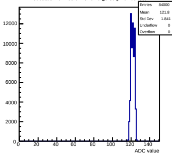
Pedestals mcm163-6A13-refv6-g0-s0-p1 ch 68 test1
