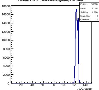
Pedestals mcm163-6A13-relv6-g0-s0-p1 ch 8 test1
