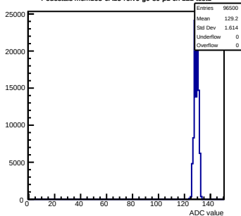
Pedestals mcm163-6A13-refv6-g0-s0-p1 ch 122 test1
