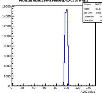
Pedestals mcm163-6A13-relv6-g0-s0-p1 ch 6 test1
