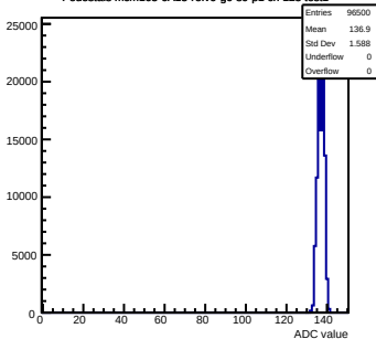
Pedestals mcm163-6A13-refv6-g0-s0-p1 ch 125 test1
