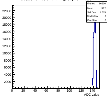
Pedestals mcm163-6A13-refv6-g0-s0-p1 ch 126 test1
