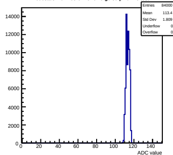
Pedestals mcm163-6A13-refv6-g0-s0-p1 ch 75 test1
