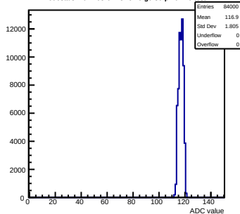
Pedestals mcm163-6A13-refv6-g0-s0-p1 ch 70 test1
