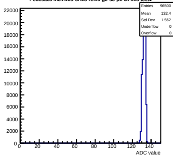
Pedestals mcm163-6A13-refv6-g0-s0-p1 ch 118 test1
