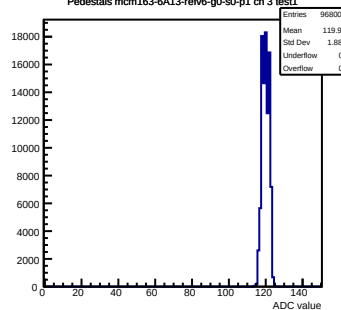
Pedestals mcm163-6A13-relv6-g0-s0-p1 ch 3 test1
