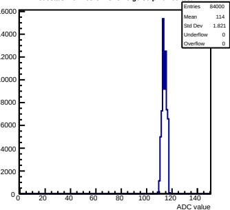
Pedestals mcm163-6A13-refv6-g0-s0-p1 ch 69 test1
