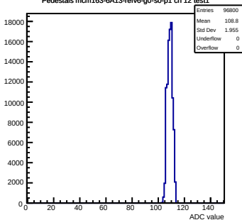
Pedestals mcm163-6A13-relv6-g0-s0-p1 ch 12 test1
