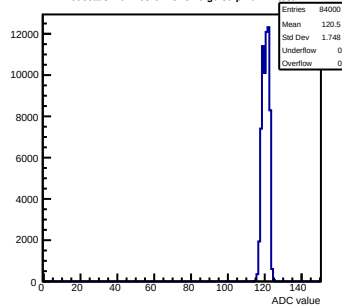
Pedestals mcm163-6A13-refv6-g0-s0-p1 ch 71 test1
