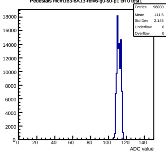
Pedestals mcm163-6A13-relv6-g0-s0-p1 ch 0 test1
