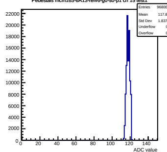
Pedestals mcm163-6A13-relv6-g0-s0-p1 ch 15 test1
