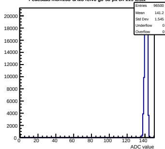
Pedestals mcm163-6A13-refv6-g0-s0-p1 ch 119 test1
