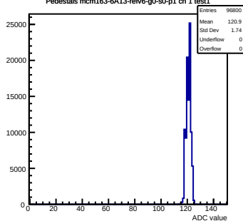
Pedestals mcm163-6A13-relv6-g0-s0-p1 ch 1 test1
