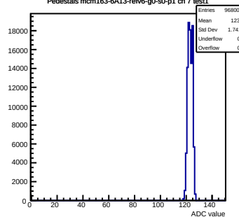
Pedestals mcm163-6A13-relv6-g0-s0-p1 ch 7 test1
