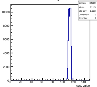
Pedestals mcm163-6A13-refv6-g0-s0-p1 ch 72 test1
