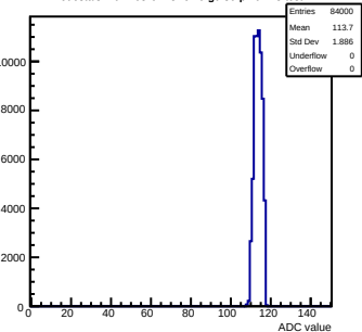
Pedestals mcm163-6A13-refv6-g0-s0-p1 ch 73 test1
