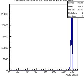
Pedestals mcm163-6A13-refv6-g0-s0-p1 ch 117 test1
