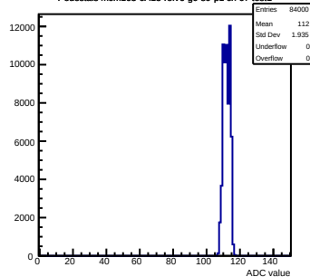
Pedestals mcm163-6A13-refv6-g0-s0-p1 ch 67 test1
