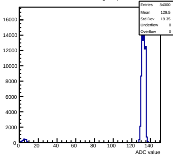
Pedestals mcm163-6A13-refv6-g0-s0-p1 ch 76 test1
