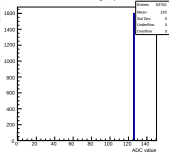
Pedestals mcm163-6A13-refv7-g0-s0-p1 ch 60 test1
