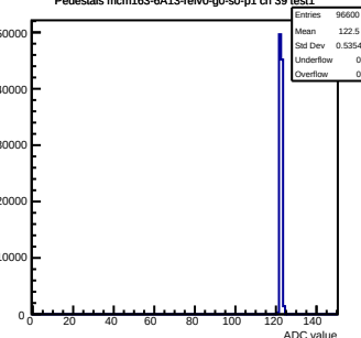
Pedestals mcm163-6A13-refV0-g0-s0-p1 ch 39 test1
