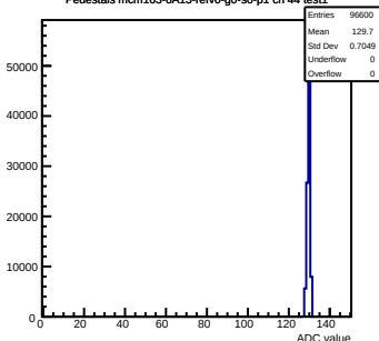
Pedestals mcm163-6A13-refV0-g0-s0-p1 ch 44 test1
