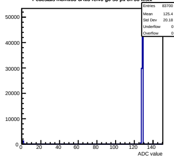
Pedestals mcm163-6A13-refV0-g0-s0-p1 ch 50 test1
