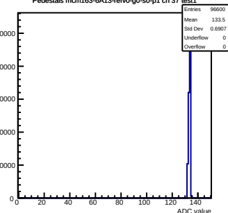
Pedestals mcm163-6A13-refV0-g0-s0-p1 ch 37 test1
