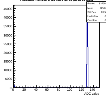
Pedestals mcm163-6A13-refV0-g0-s0-p1 ch 55 test1
