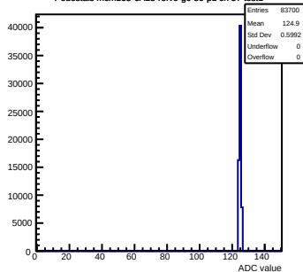
Pedestals mcm163-6A13-refV0-g0-s0-p1 ch 57 test1
