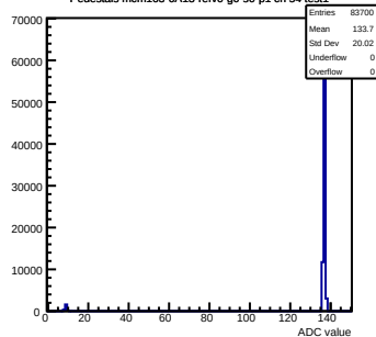
Pedestals mcm163-6A13-refV0-g0-s0-p1 ch 54 test1
