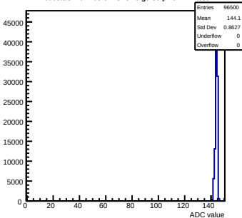
Pedestals mcm163-6A13-refV0-g0-s0-p1 ch 127 test1
