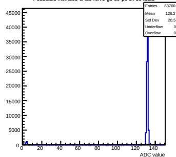
Pedestals mcm163-6A13-refV0-g0-s0-p1 ch 59 test1
