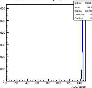
Pedestals mcm163-6A13-refV0-g0-s0-p1 ch 125 test1
