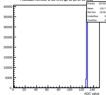
Pedestals mcm163-6A13-refV0-g0-s0-p1 ch 51 test1
