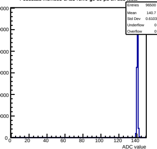
Pedestals mcm163-6A13-refV0-g0-s0-p1 ch 113 test1
