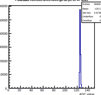
Pedestals mcm163-6A13-refV0-g0-s0-p1 ch 47 test1
