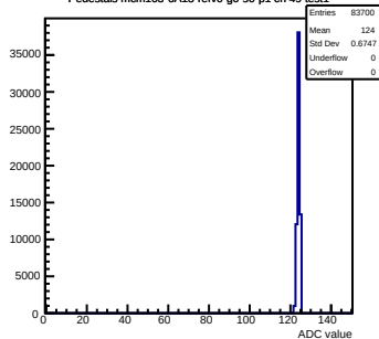
Pedestals mcm163-6A13-refV0-g0-s0-p1 ch 49 test1
