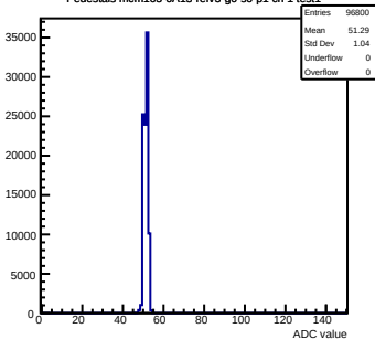
Pedestals mcm163-6A13-refV3-g0-s0-p1 ch 1 test1
