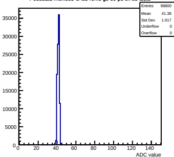
Pedestals mcm163-6A13-refV3-g0-s0-p1 ch 13 test1
