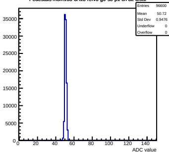
Pedestals mcm163-6A13-refv3-g0-s0-p1 ch 32 test1
