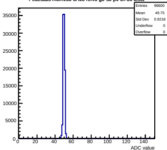
Pedestals mcm163-6A13-refv3-g0-s0-p1 ch 36 test1
