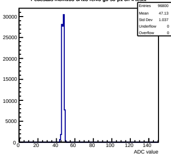
Pedestals mcm163-6A13-refV3-g0-s0-p1 ch 4 test1
