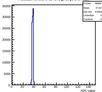
Pedestals mcm163-6A13-refV3-g0-s0-p1 ch 14 test1
