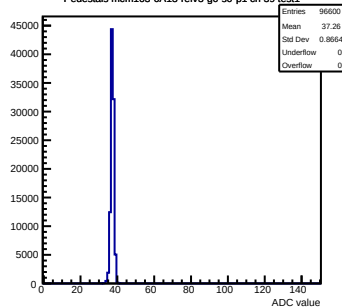
Pedestals mcm163-6A13-refv3-g0-s0-p1 ch 39 test1
