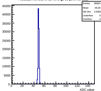
Pedestals mcm163-6A13-refV3-g0-s0-p1 ch 10 test1
