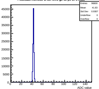
Pedestals mcm163-6A13-refV3-g0-s0-p1 ch 5 test1
