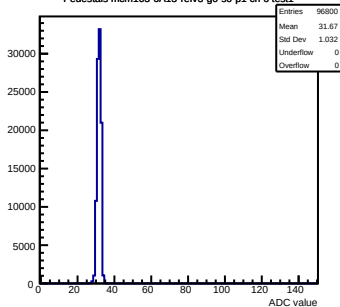
Pedestals mcm163-6A13-refV3-g0-s0-p1 ch 6 test1
