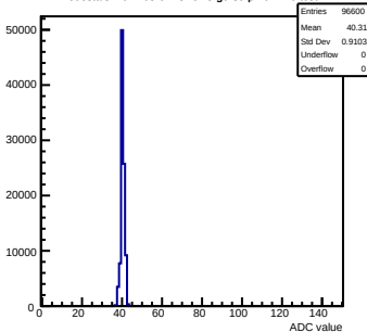
Pedestals mcm163-6A13-refv3-g0-s0-p1 ch 110 test1
